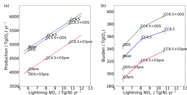
Figure 2. Correlation between (a) P(\text{O}_x) and \text{LNO}_x and (b) tropospheric ozone burden and \text{LNO}_x . Linear fits in (a) and connecting lines in (b) are drawn between runs which differ only in their climate states. Error bars indicate \pm 1 standard deviation.
