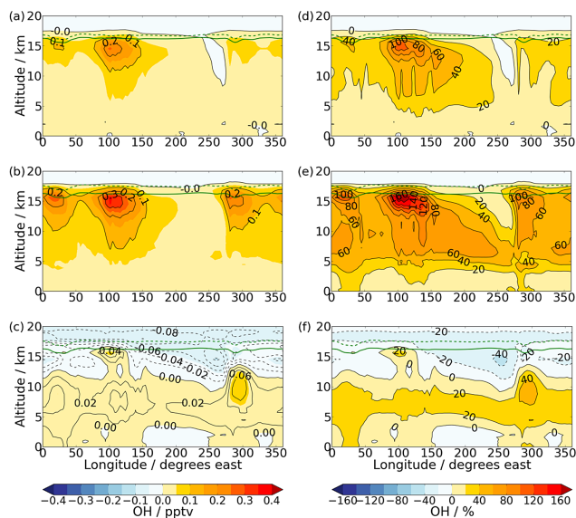
Figure 4. Annual mean, longitude–altitude cross sections of tropically averaged ( 20^\circ \text{S} – 20^\circ \text{N} ) changes (shading and contours) in OH volume mixing ratios (pptv) from Base to (a) \Delta\text{CC4.5} (b) \Delta\text{CC8.5} and (c) \Delta\text{CC8.5}(f\text{LNO}_x) ; the differences as a percentage of the Base values for (d) \Delta\text{CC4.5} (e) \Delta\text{CC8.5} and (f) \Delta\text{CC8.5}(f\text{LNO}_x) . Solid (Base run) or dashed (future runs) green lines indicate the height of the thermal tropopause.
