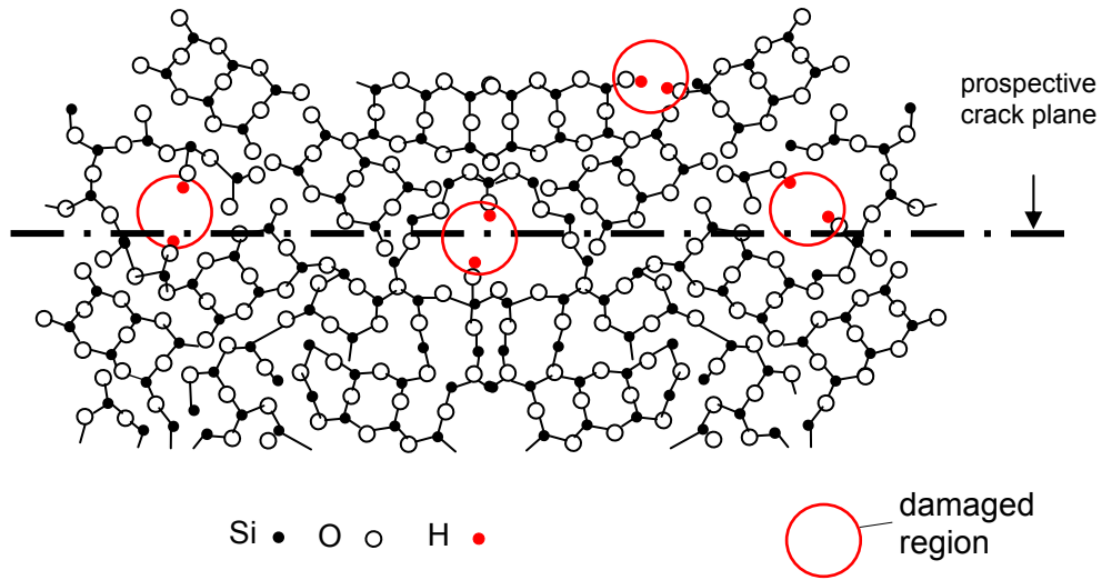
Fig. 3 Volume element of silica showing damage by bond breaking due to water/silica reaction, third dimension ignored.
