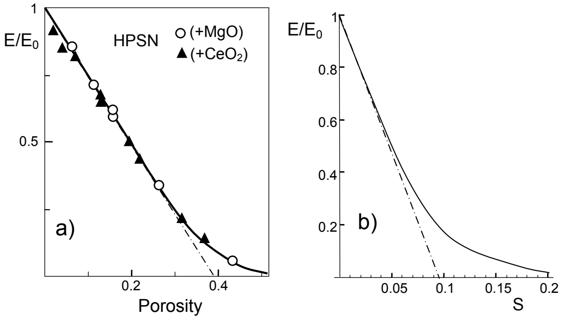
Fig. 2 a) Effect of pores on Young's modulus of HPSN-ceramics, b) behaviour for silica; expected behaviour tentatively introduced by the curve (dash-dotted lines: extrapolation of initially linear variation).
