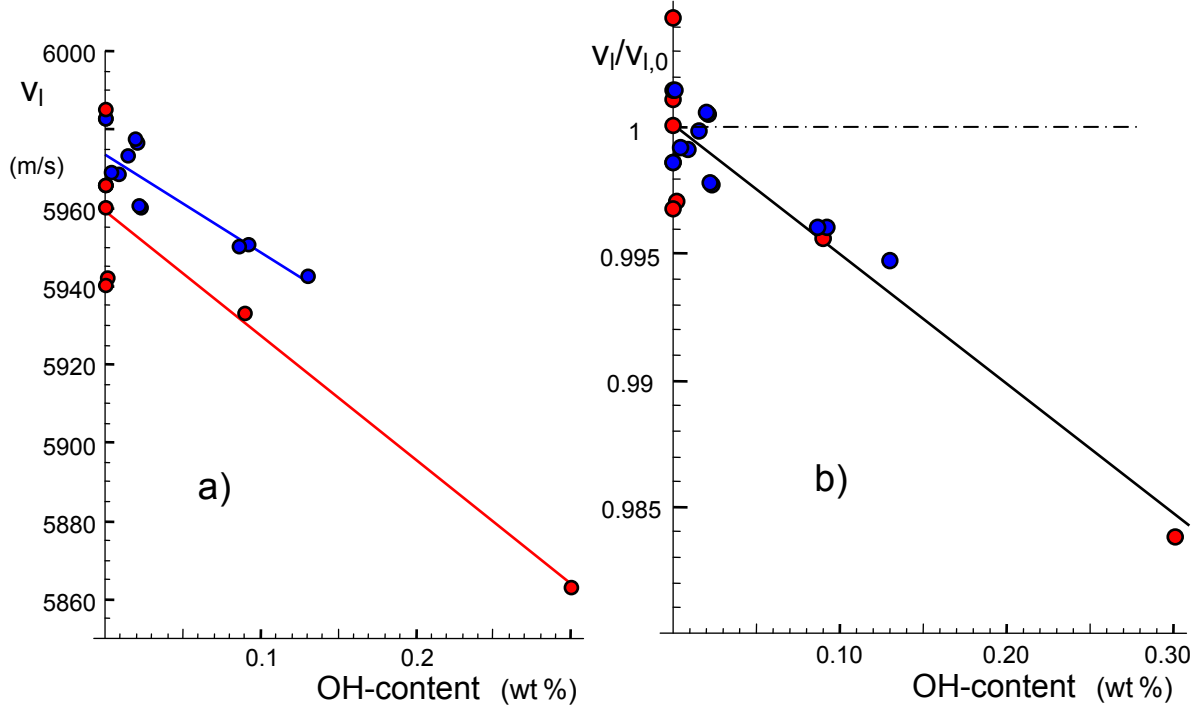
Fig. 1 a) Longitudinal sound velocity in silica with different OH-content (blue circles: results by Fraser [5], red circles: results by LeParc et al. [6]), b) normalized representation of the two data sets.
