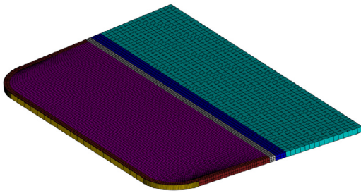
Fig. 3. Hexahedral mesh HCPB breeder blanket slice showing the tungsten armour (yellow), Eurofer first wall (red), lithium ceramic (purple), rear blanket casing (grey), shielding (blue) and the blanket coolant supply (turquoise). (For interpretation of the references to color in this figure legend, the reader is referred to the web version of this article.)
