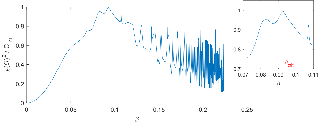
Figure 1: Plot of \chi(\Omega)^2/C_{\text{int}} against \beta for k = \sqrt{10} , \varepsilon_r = 2 and \mu_r = 1 . The inset is an enlarged view of the plot around \beta_{\text{crit}}^+ \approx 0.0926 .
