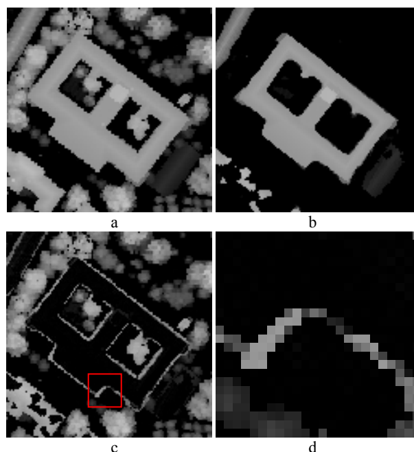
Figure 1. Sections of an urban scene (Test area Karlsruhe, Germany). a) elevation images captured by first pulse mode, b) elevation images captured by last pulse mode, c) difference image of first and last pulse mode, d) subsection of the difference image (building boundary).
