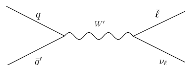
Fig. 1. Production and decay of an SSM W' boson. The final state shown denotes both the (\bar{l}\nu_l) state and its charge conjugate.
