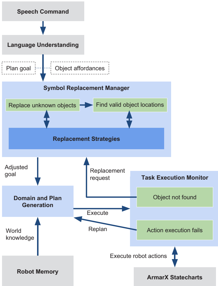
Figure 6.1: The main modules, control flow and data flow of the task execution approach. The green and blue components were developed in this work.
