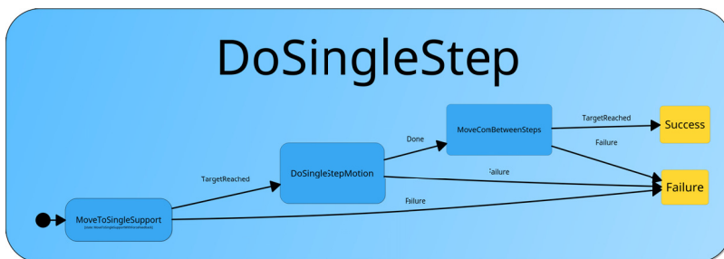
Figure 7.16: State for a single step with the bipedal robot ARMAR-4.
