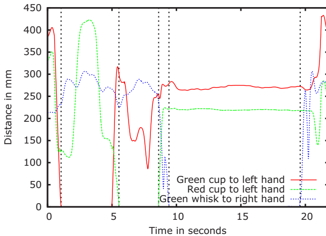
Figure 7.4: Segmentation based on object contact relations: When two objects get in contact with each other (contact in this case is approximated as distance < 7 mm) or lose contact, a new key frame is inserted with the current world state attached to it. The dotted vertical lines depict the detected semantic segments. Only distances between objects that get in contact during the complete demonstration are shown. Source: (Wächter and Asfour, 2015) © 2015 IEEE
