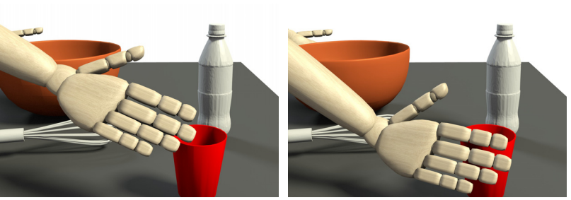
Figure 4.5: When approaching an object the first contact (left) between two entities is not always the desired key frame. Therefore, the key frame detection is deferred until the contact relation is stable (right).
