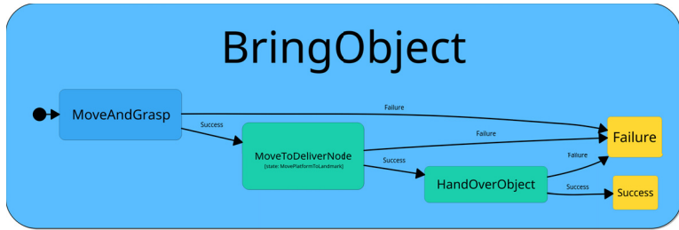
Figure 7.10: Top level of the BringObject task statechart, in which the robot moves to a given location, grasps an object and hands it over to a human at a delivery location. This and the following statecharts are exported directly using the graphical statechart editor.
