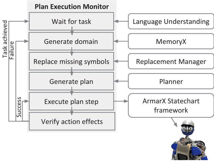
Figure 6.7: Control flow of the task execution and monitoring with the main components for each phase.
