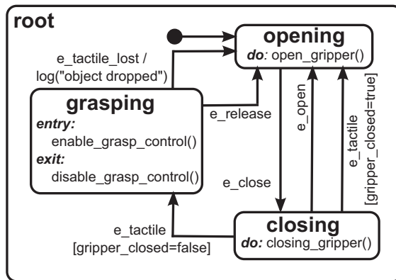
Figure 3.5: Example for coordinating a gripper with restricted Finite State Machines (rFSM) for modeling hierarchical robot skills. Source: (Klotzbücher and Bruyninckx, 2012) © Joser 2012
