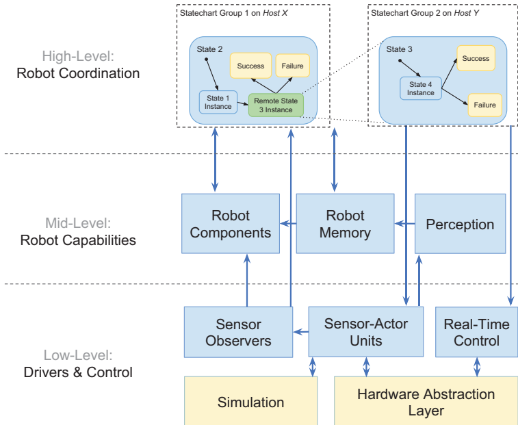
Figure 2.3: Layers and main elements of ArmarX.
