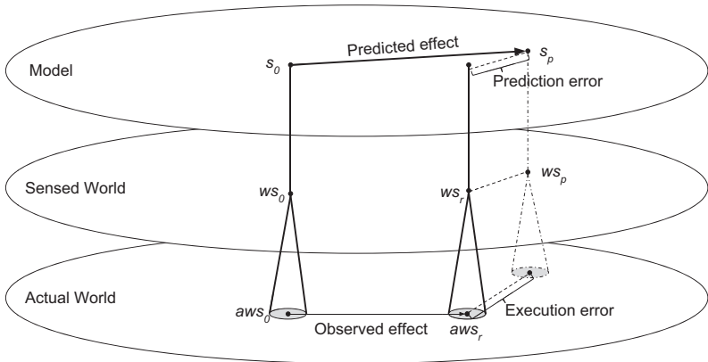
Figure 2.2: OACs work in three different attribute spaces: Actual world space, sensor world space and model space. A state from the actual world ( aws ) is perceived with noisy sensors and mapped into the sensed world space ( ws ). The sensed world state can be mapped without loss into the model world state ( s ). The execution of an OAC might lead to a different world state than the predicted world state. Hence, the OAC should learn to minimize the prediction error as well as the execution error.
