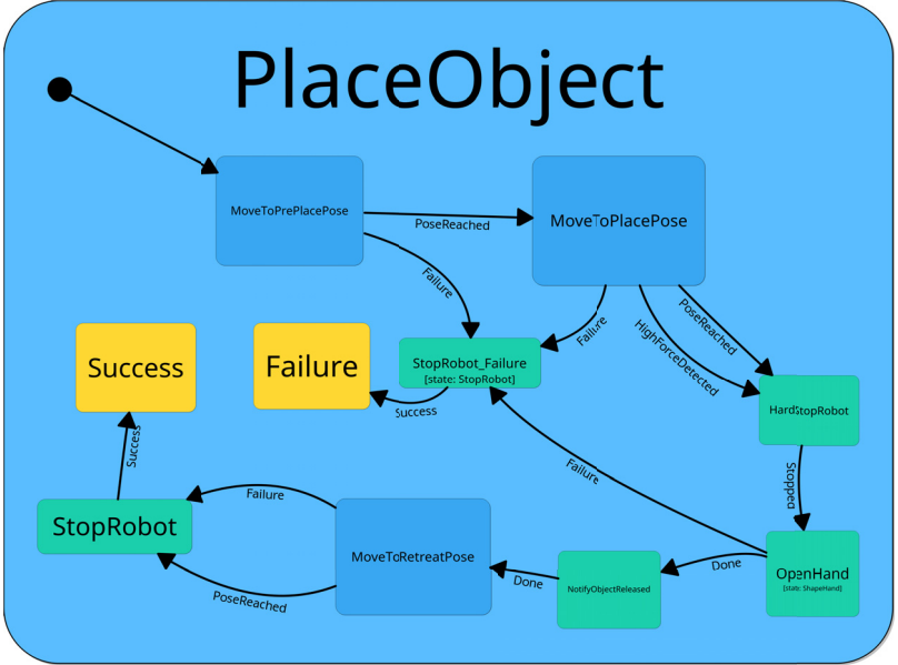
Figure 6.6: The equivalent of the planning operator PlaceObject represented as a statechart for execution on a robot. Only the first level of the hierarchical statechart is shown for simplicity.
