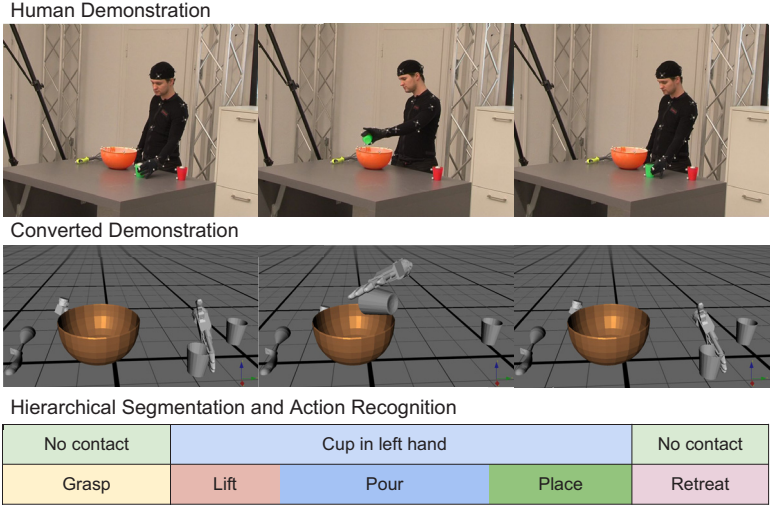
Figure 4.1: Overview over the segmentation and recognition approach.
