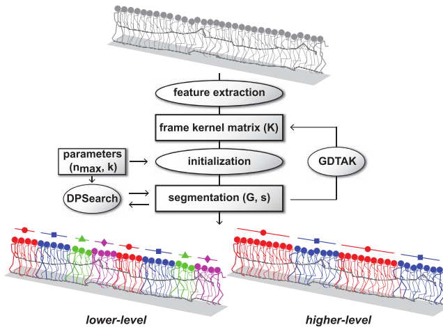
Figure 3.2: Hierarchical Aligned Cluster Analysis used to segment motions into recurring motion primitives. Source: (Zhou et al., 2013) © 2013 IEEE
