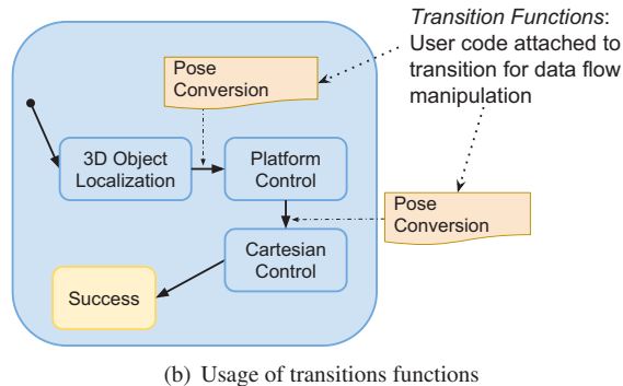
Figure 5.4: Transition Functions reduce the number of needed states and improve the comprehensibility of reused statecharts.
