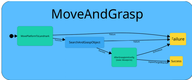
Figure 7.11: Second level of the BringObject task statechart: move to a location and grasp an object.
