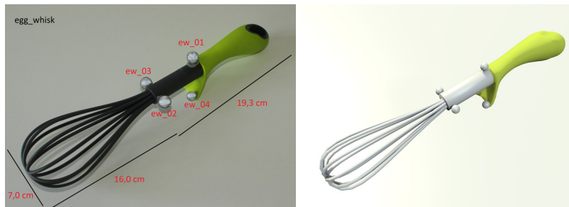
Figure 7.2: Left : Image of a real object with attached reflective markers from the KIT Whole-Body Human Motion Database (Mandery et al., 2016b). Right : A visualization of the corresponding 3D mesh model with attached virtual markers.
