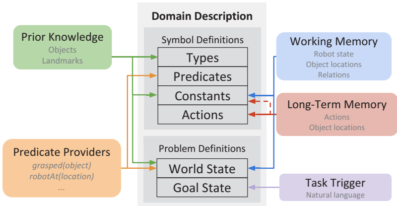
Figure 6.5: Components involved in the domain description generation.
