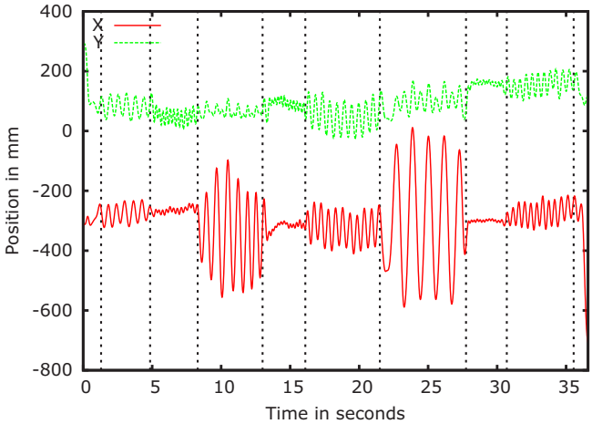
Figure 7.5: Sub-segmentation of one semantic segment (sponge touches hand and table) into different subsegments, i.e. different wiping styles. The dotted vertical lines depict the segmentation points. Whenever the wiping styles changes, a key frame is inserted. Source: (Wächter and Asfour, 2015) © 2015 IEEE
