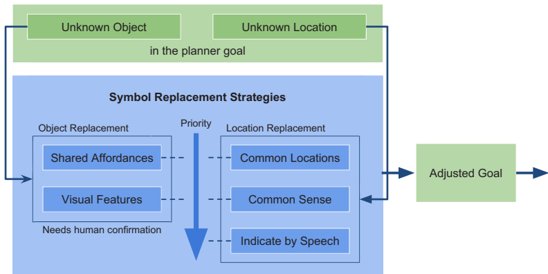
Figure 6.2: The Symbol Replacement Manager provides replacements for objects and locations based on various replacement strategies. These strategies include replacement based on shared visual affordances or on common sense knowledge extracted from large text corpora.
