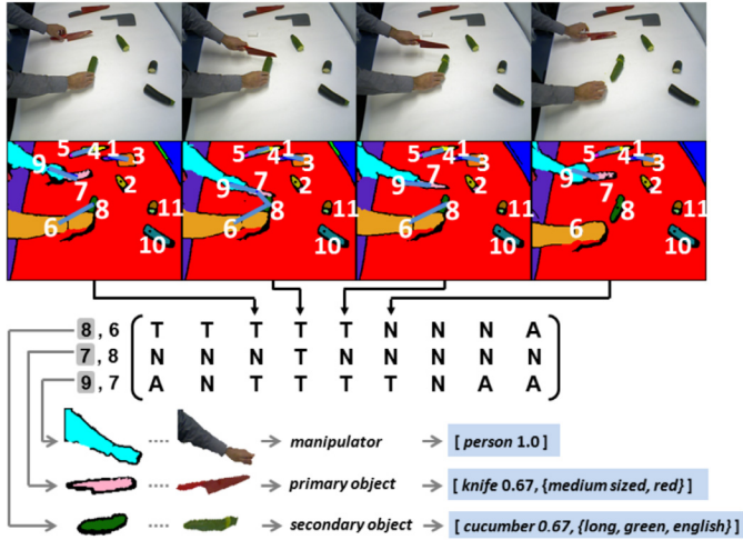
Figure 3.4: Segmentation of manipulation actions based on object relation changes extracted from color and depth regions calculated from RGB-D images. Source: (Aksoy et al., 2017) © 2017 IEEE
