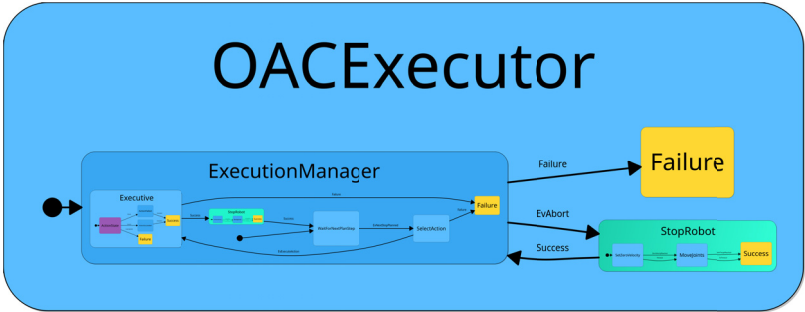
Figure 7.19: The top level state for OACs execution encapsulates the ExecutionManager state to allow unexpected abort of the execution (event EvAbort ).
