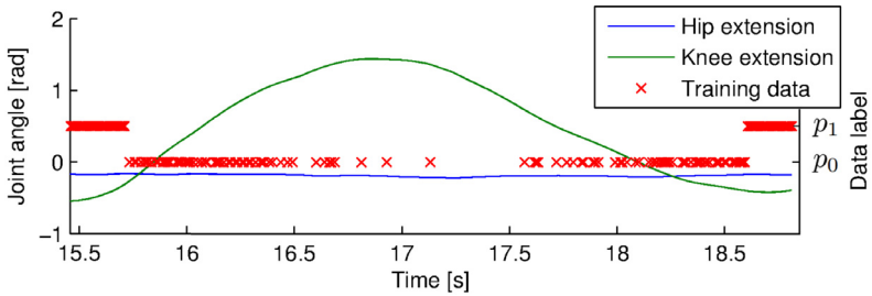
Figure 3.3: Segmentation based on data point classification. p_1 denote segment points, while p_0 denote non-segment points. Instead of only using single segment points for classification a window around each segment point is used to obtain a more balanced training set. Source: (Lin et al., 2014) © 2014 IEEE
