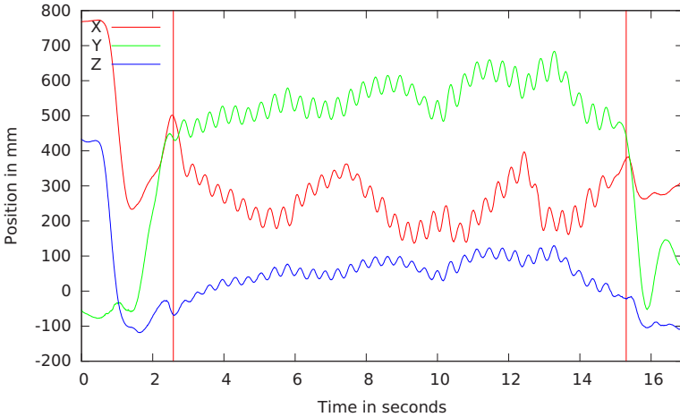
Figure 7.26: Hierarchical segmentation of a wiping task. The curves depict the motion of the right hand on the Cartesian axes whereas the red vertical dashed lines are semantic key frames.
