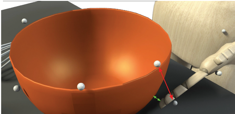
Figure 4.2: Difference between resulting object distances of marker representation and mesh model representation. The red arrow illustrates the distance between the closest two markers of two objects while the green arrow illustrates the minimum distance between the mesh models. The mesh model distance is significantly smaller.
