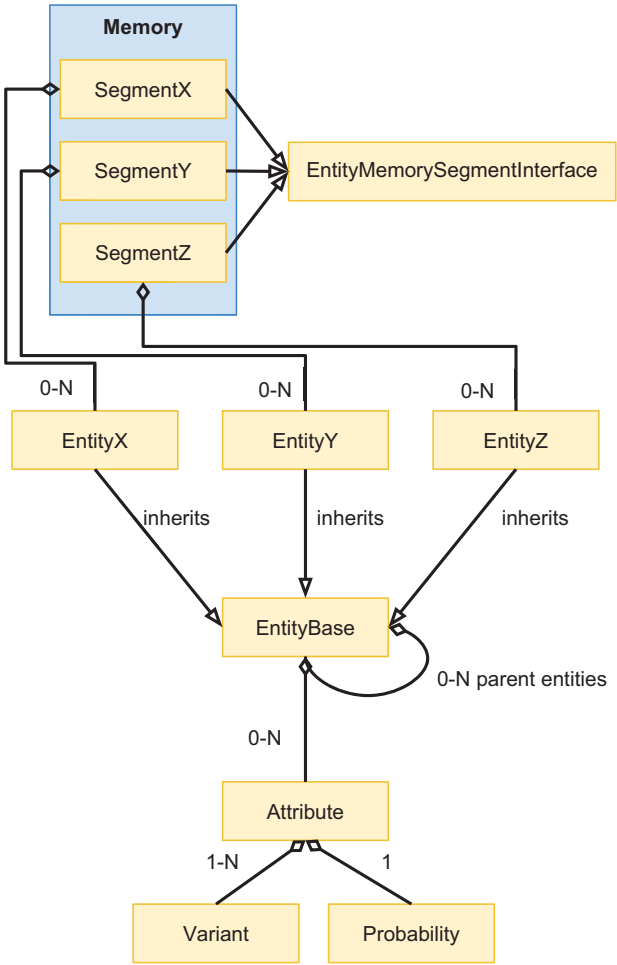
Figure 2.4: A memory in MemoryX is a segmented memory. Each segment contains data elements of one type (e.g. object class). Each element type is of the base type Entity . An entity is a generic data type with a set of attributes. Attributes themselves consist of 1 \dots n values of a generic type called Variant and a probability measure. Variants can be any type of data, from primitive types like int or string to arbitrary complex types like 6D-poses or n-dimensional trajectories.
