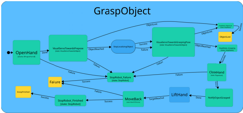
Figure 7.14: Fifth level of the BringObject task statechart: Execute grasping using visual servoing.
