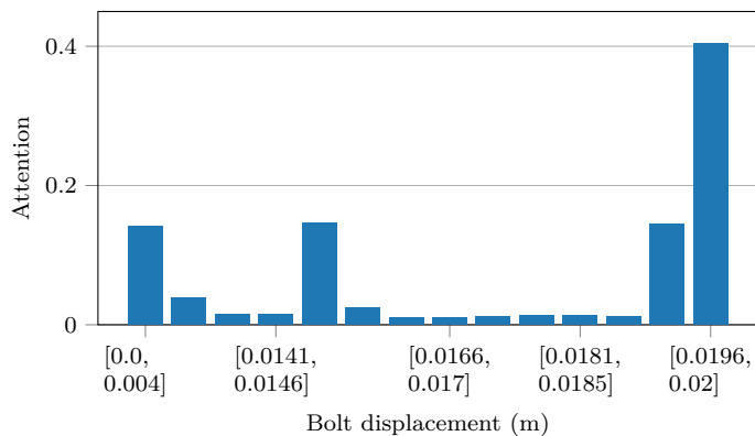
(a) Attention grouped by bcd intervals.
