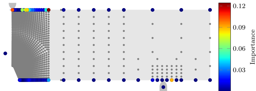
(a) Profile of half of the specimen with importance of sensors.
