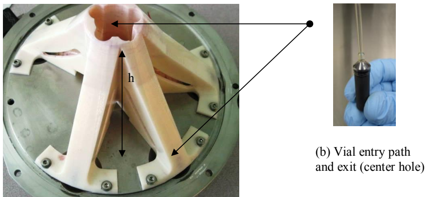
Figure 8. (a) Vial guide mounted at cryostat top plate bottom, \text{\O} = 250 \text{ mm} , h = 100 \text{ mm} , (b) vial.
