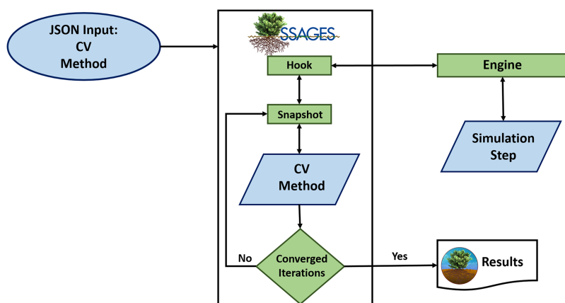
FIG. 1. Flowchart of running a simulation using SSAGES. A JSON input file defines collective variables and sampling methods to be used. SSAGES then starts the simulation with a given engine and updates quantities according to the method until convergence or a prescribed number of iterations are met.
