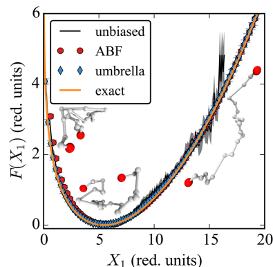
FIG. 7. Free energy profiles along the first Rouse mode amplitude X_1 , using reduced units, for an ideal Gaussian chain obtained from unbiased, brute-force MD simulation (black line with gray error region), the ABF method in SSAGES (red circles), the umbrella sampling method in SSAGES (blue diamonds), and Eq. (2) (orange line). Insets are three representative configurations of the Gaussian chain for X_1 \approx 1.0, 5.0, and 15.0 from left to right. Error bars and/or error regions represent the standard error of the mean.
