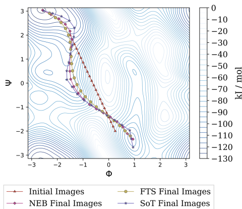
FIG. 6. Free energy landscape with chain-of-states results for ADP calculated using nudged elastic band (diamonds), finite temperature string (circles), and swarm of trajectories (stars). The contour map was obtained using ABF. We observe excellent agreement between nudged elastic band and the string methods, as well as with ABF.
