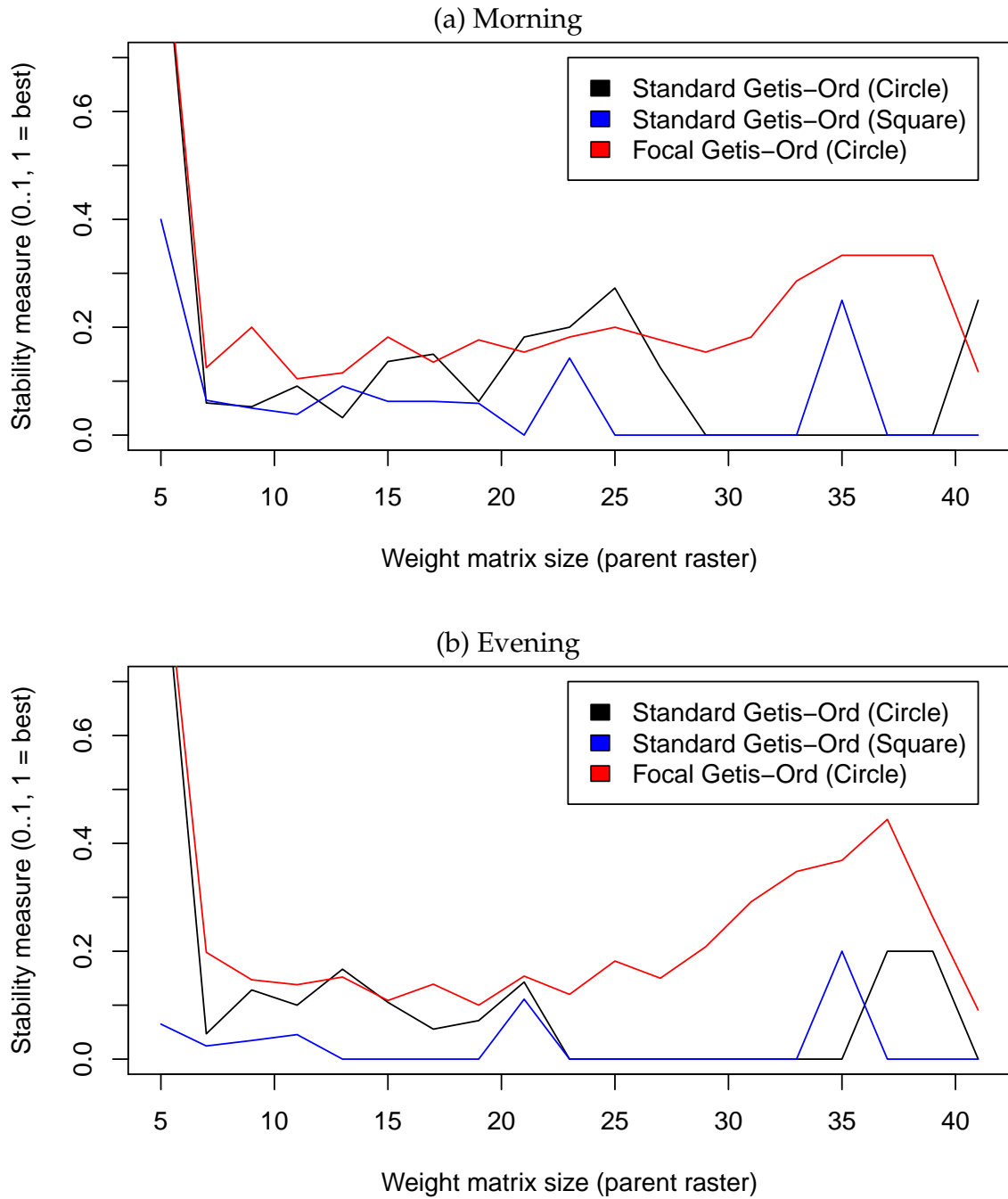
Figure 5.2: Evaluation results - Standard vs Focal G^*
