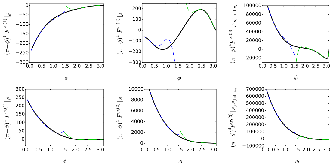
Figure 6. Same as figure 5 but for the scalar and pseudo-scalar currents.
