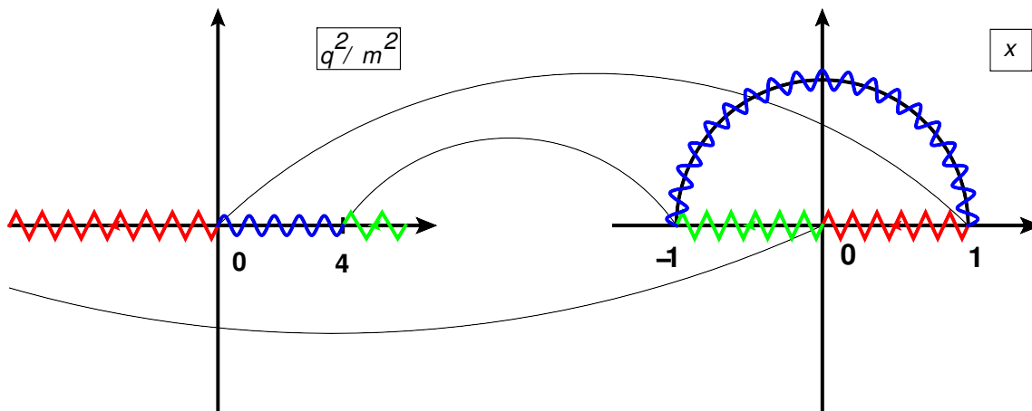
Figure 2. Illustration of the variable transformation between q^2/m^2 and x as given in eq. (2.1). The left graph represents the q^2/m^2 plane and on the right the complex x plane is shown. The (coloured) wiggled and zigzag lines show the mapping of the various intervals, whereas the straight lines indicate the mapping for special values of q^2/m^2 and x .
