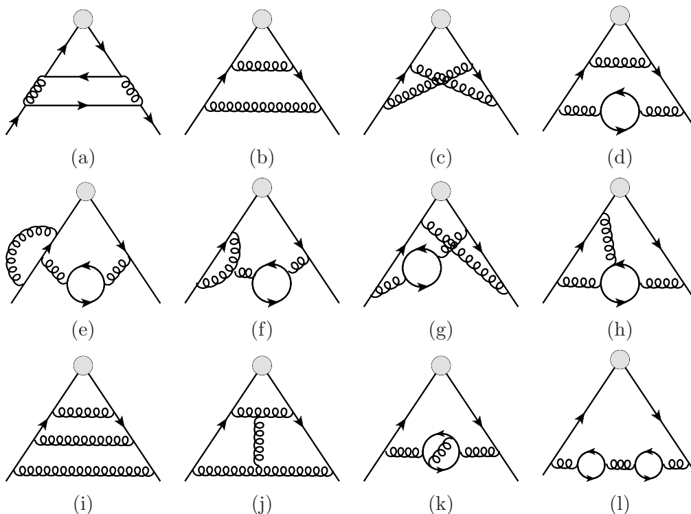
Figure 1. Sample diagrams contributing to the form factors. Solid and curly lines represent quarks and gluons, respectively. The grey blob refers to one of the external currents given in eq. (1.1). Singlet contributions, as shown in (a), are not considered in this paper.
