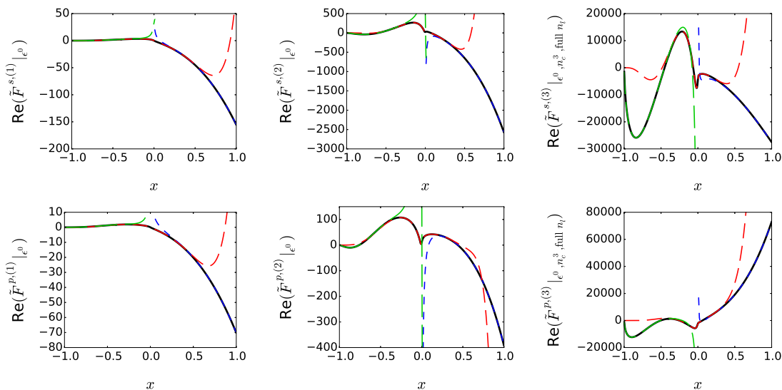
Figure 4. Same as figure 3 but for the scalar and pseudo-scalar currents.
