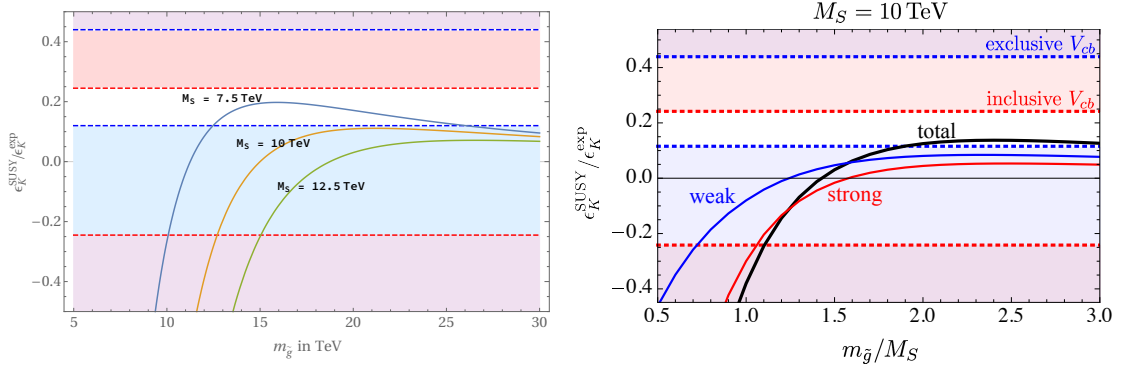
Figure 2.3.: The behaviour of the gluino box contribution to \epsilon_K^{\text{NP}} normalized to the SM value. The blue (red) shading represents the regions which are excluded at 95 % confidence level by \epsilon_K measurements, if the exclusive (inclusive) value for |V_{cb}| is taken for the SM prediction. See section 2.5 for a discussion of the exclusive and inclusive values of |V_{cb}| . The left plot shows the behaviour according to the approximate formula given in the text, while the right plot is taken from our paper [1] and shows the exact numerical behaviour. There, the red line corresponds to gluino box contribution while the blue line corresponds to the sum of the box contributions with one or two winos.
