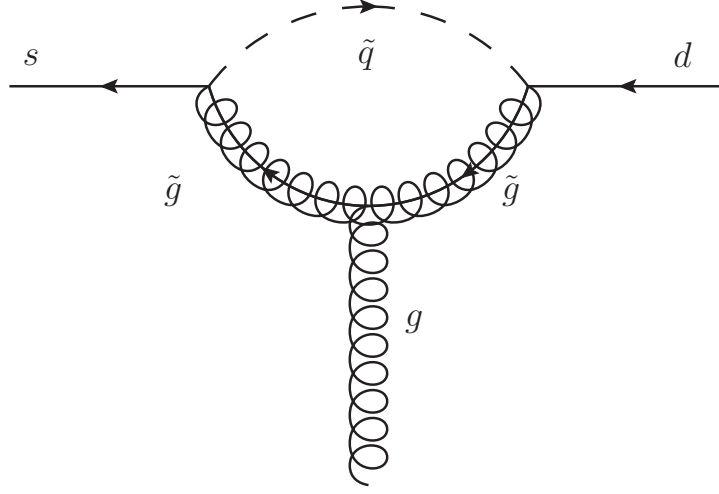
Figure B.1.: The gluino gluon chromomagnetic penguin, gluon attached to the gluino line.
