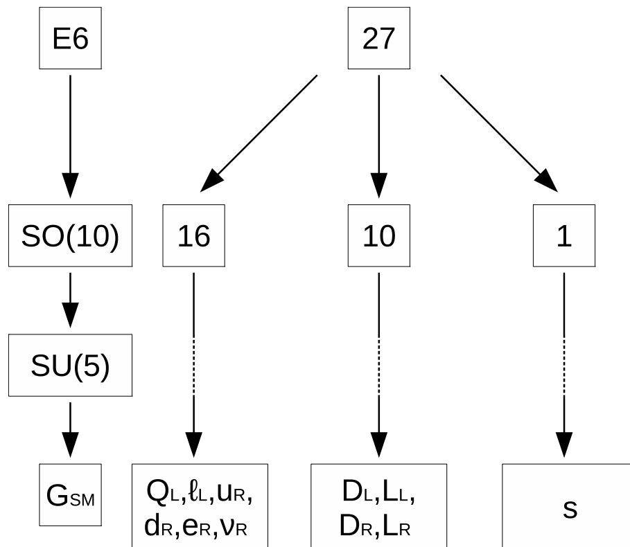
Figure 1.1.: Sketch of the spectrum of our model.
