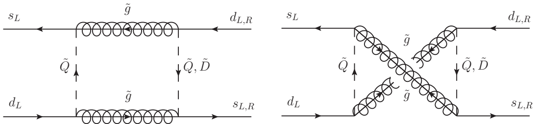
Figure 2.2.: Suppression of diagrams contributing to \epsilon_K : For m_{\tilde{g}} = 1.5M_S , the diagrams with outgoing left chiral quarks cancel exactly. The diagrams with outgoing right chiral quarks vanish in the limit of negligible mixing among right chiral squarks.
