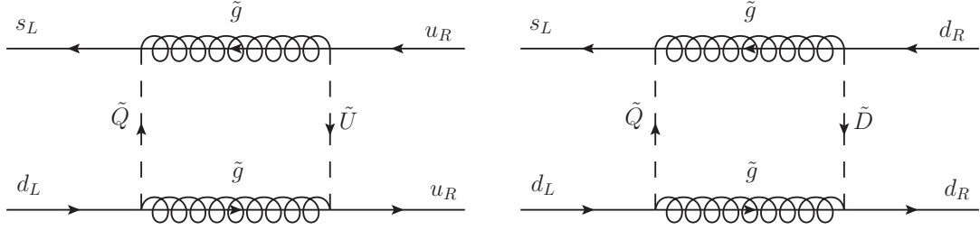
Figure 2.1.: Trojan penguins [48] [49]: Gluino boxes contributing to \epsilon'_K/\epsilon_K
