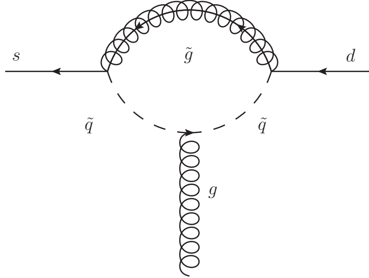
Figure B.2.: The gluino gluon chromomagnetic penguin, gluon attached to the squark line.
