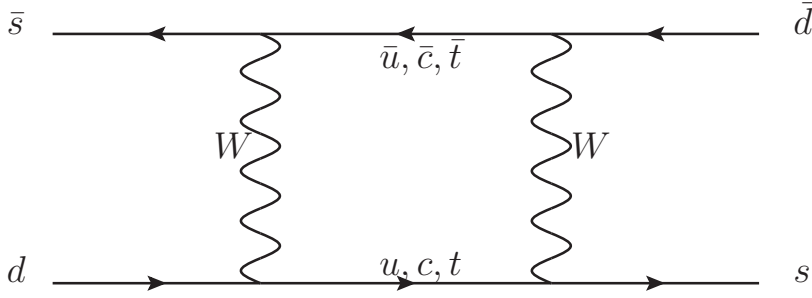
Figure 3.1.: Feynman diagram representing the transition of a K^0 into a \bar{K}^0 by the exchange of two W bosons.
