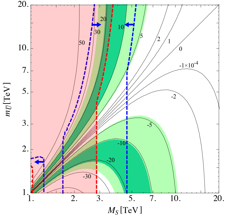
Figure 2.4.: Contour plot of the supersymmetric contributions to \epsilon'_K/\epsilon_K in 10^{-4} as appeared in our paper [1]. The dark (light) green bands resolve the \epsilon'_K/\epsilon_K discrepancy at 1\sigma ( 2\sigma ). The red shaded region is the 95% exclusion region of \epsilon_K in case of an inclusive V_{cb} ; the region between the two blue dashed lines is the favored region of \epsilon_K in case of an exclusive V_{cb} .
