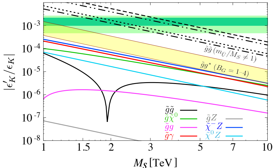
Figure 2.5.: All contributions to \epsilon'_K/\epsilon_K as appeared in our paper [1]. The dark (light) green bands resolve the \epsilon'_K/\epsilon_K discrepancy at 1\sigma ( 2\sigma ).
