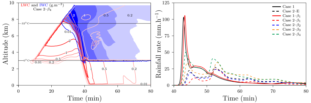
Figure 6.13 – (a, left) Liquid water content ( \text{g}\cdot\text{m}^{-3} , red) and ice water content ( \text{g}\cdot\text{m}^{-3} , blue) simulated by DESCAM as a function of altitude and time for the case with all minerals active as INP and all ice nucleation mechanisms active for an increased mineral aerosol particles number concentration (case 2- \beta_4 ). (b, right) Time evolution of the rainfall rate ( \text{mm}\cdot\text{h}^{-1} ) for the only-liquid case (cases 1, continuous) and all minerals cases for all ice processes (cases 2, dashed) for the reference study (black), a mineral aerosols concentration of 10c_0 ( \beta_1 , red), 2c_0 ( \beta_2 , blue) and 0.1c_0 ( \beta_3 , orange) and 0.01c_0 ( \beta_4 , green).
