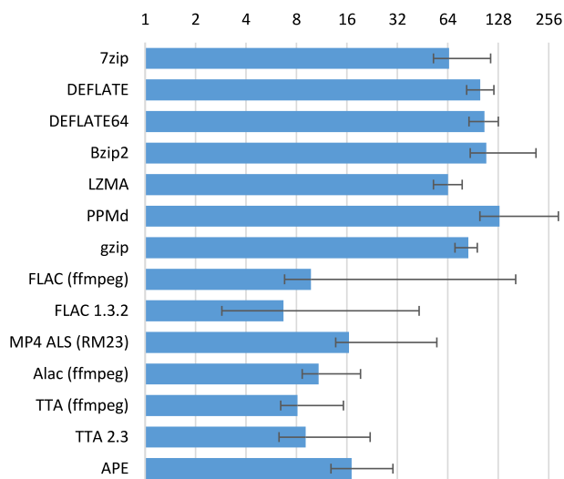
Fig. 3. Mean decompression times. Values are relative to DELFLATE in %.
