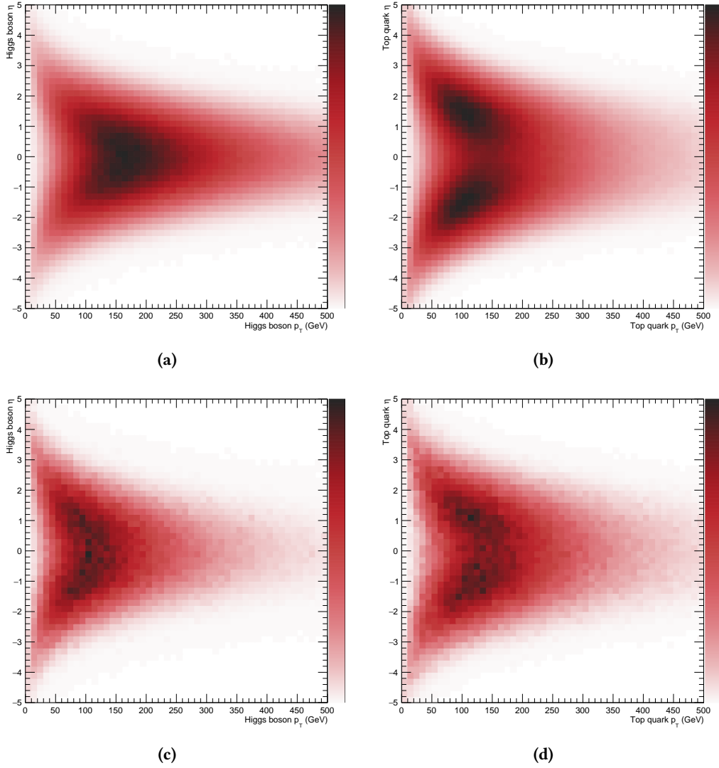
Figure C.4: Two-dimensional distributions of the transverse momentum and pseudorapidity of the Higgs boson (a) and the top quark (b), both for the ITC scenario, in the simulation of the tH W process. The corresponding distributions for the SM scenario ((c) and (d)) are obtained by reweighting each generated event.
