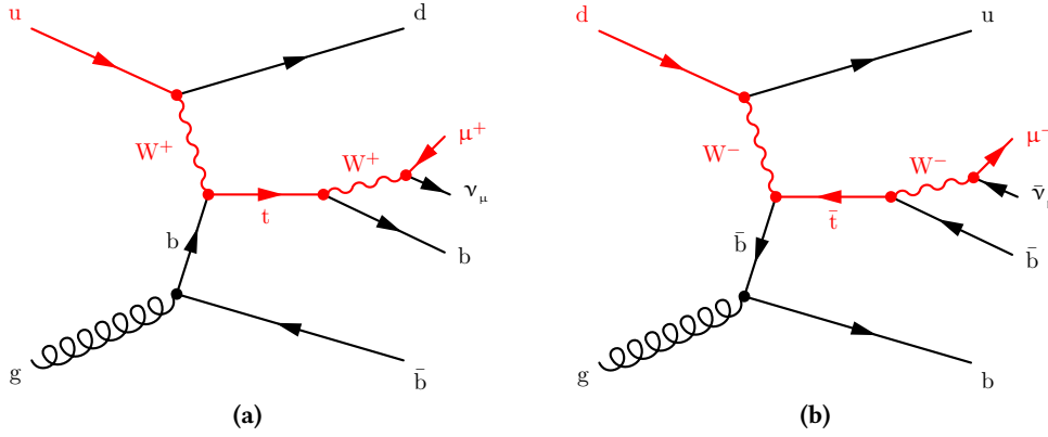
Figure 6.2.: Leading-order Feynman diagrams for single top quark (a) and single top antiquark (b) production in the t channel in the 4FS description. The electric charge of the muon from the top quark or top antiquark decay can be directly related to an up- or down-type quark in the initial state of the process. Therefore, t -channel single top quark production can be used to probe the initial state PDF.
