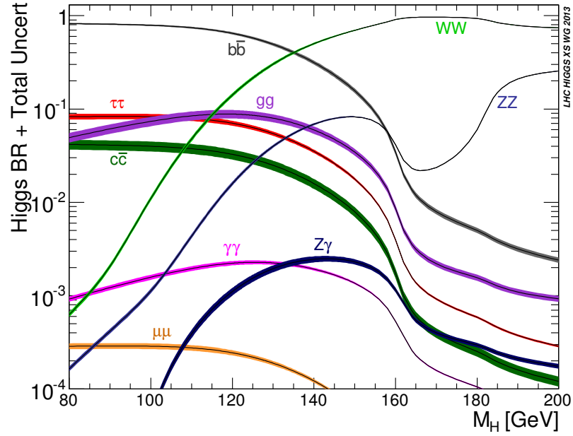
Figure 1.11: The predicted branching ratios of the Higgs boson depending on the Higgs boson mass. Since the Higgs boson couples directly to mass, the branching ratio into heavier particles is higher compared to lighter particles. Although no direct decay to massless particles like gluons or photons is allowed, they can couple to the Higgs boson through virtual loops of heavier particles like the top quark or the W boson [54].
