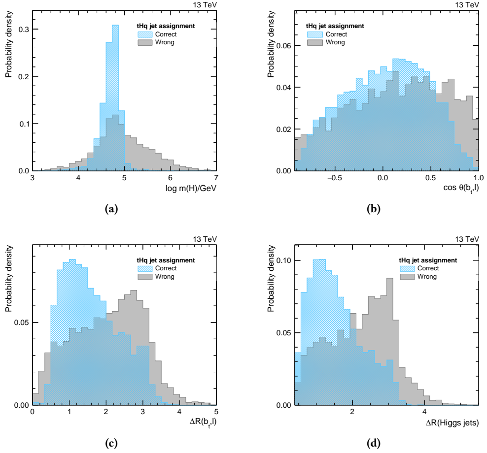
Figure C.5.: Distributions of input variables for the tHq event reconstruction, ranked 1 st to 4 th in the training of the BDT: the invariant mass of the reconstructed Higgs boson (a), the cosine of the angle between the jet assigned to the bottom quark of the top quark decay and the lepton (b), \Delta R between the jet assigned to the bottom quark from the top quark decay and the lepton (c) and \Delta R between the two jets assigned to the Higgs boson (d).
