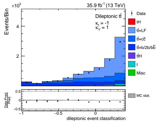
Figure 8.23: The resulting distribution of the dileptonic event classification BDT in the dileptonic control region. The simulation is scaled to the expected number of events and the last bin of the distribution also contains all events that have larger values. The data is well described by the simulation.
