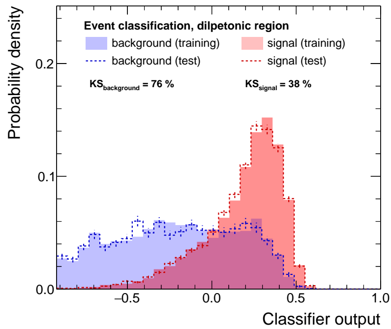
Figure 8.21.: The performance of the dileptonic event classification BDT is tested against overtraining by comparing the result on the training data set with a data set that has not been used in training process. Similar separation power is observed, no overtraining is present.
