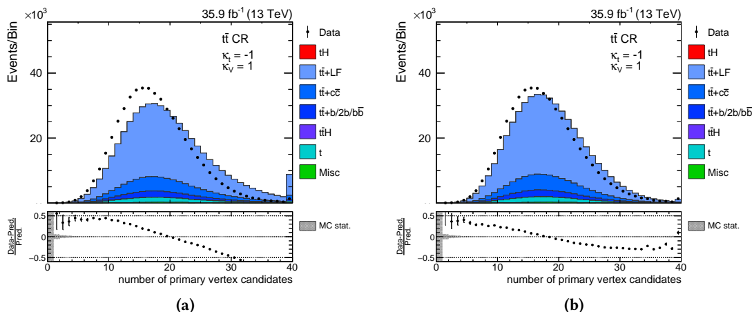
Figure 8.8.: The distribution of the number of primary vertices is different for simulation and data (a) in the 2 tag control region ( \bar{t}\bar{t} CR). To correct this disagreement, the simulated events are reweighted to match the observed distribution (b). A slight improvement is achieved, but disagreement can still be observed. The simulation is scaled to the integral of data.
