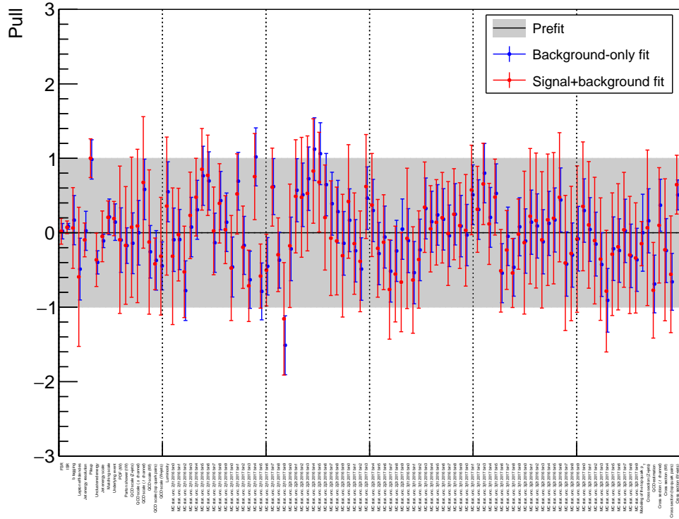
Figure B.15.: Pulls of all nuisance parameters in the combined fit for the background-only fit (blue) and the signal+background fit (red). The pull of a nuisance parameter shows how the value of the nuisance parameter changes during the maximum-likelihood fit with respect to its initial (prefit) value and uncertainty.
