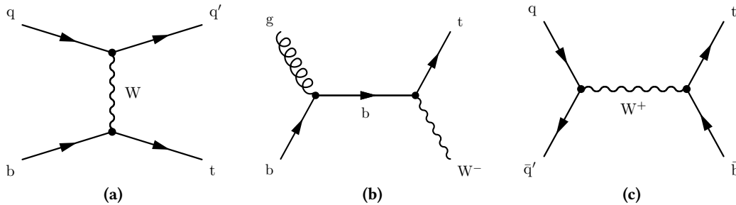
Figure 1.7.: The three main possibilities to produce a single top quark at the LHC through a Wtb vertex. The most common one is the t channel (a), followed by the tW -associated production (b) and the s channel (c).
