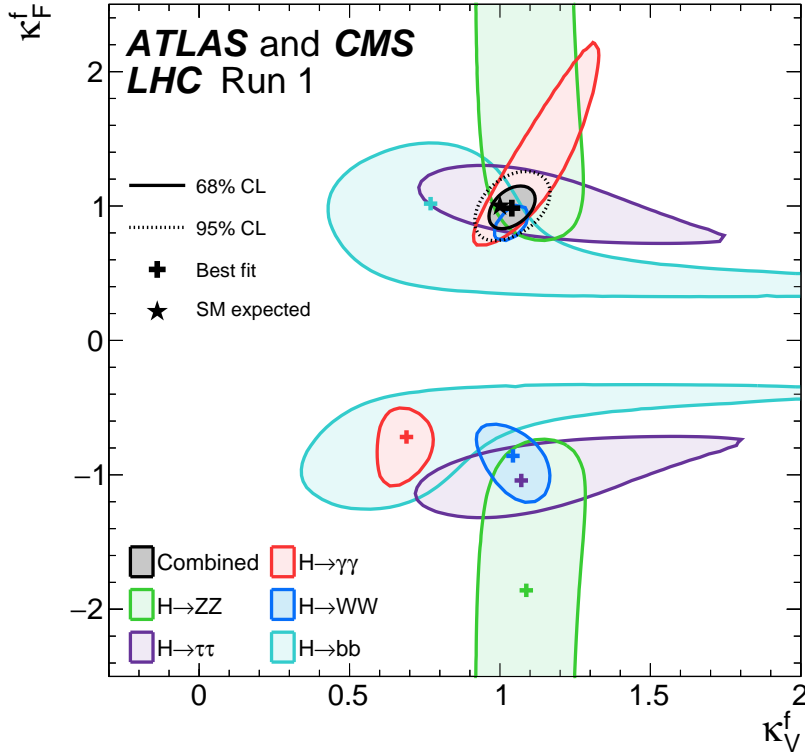
Figure 1.12.: The experimental status of constraints on the coupling modifiers of the Higgs boson to fermions \kappa_F^f and vector bosons \kappa_V^f after the combination of the Higgs boson measurements from the ATLAS and CMS Collaborations at Run I of the LHC [49].
