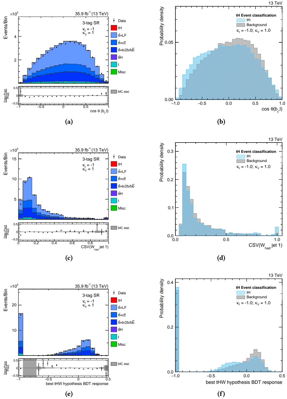
Figure C.15.: Distributions of input variables for the single-lepton event classification, ranked 9 th to 11 th in the training of the BDT: the cosine of the angle between the b -tagged jet from the top quark decay and the lepton ((a) and (b)), the output of the b tagging discriminant for the jet assigned to the hadronically decaying W boson with the highest transverse momentum ((c) and (d)) and the output of the tHW reconstruction BDT ((e) and (f)). The distributions on the left are scaled to the expected number of events.
