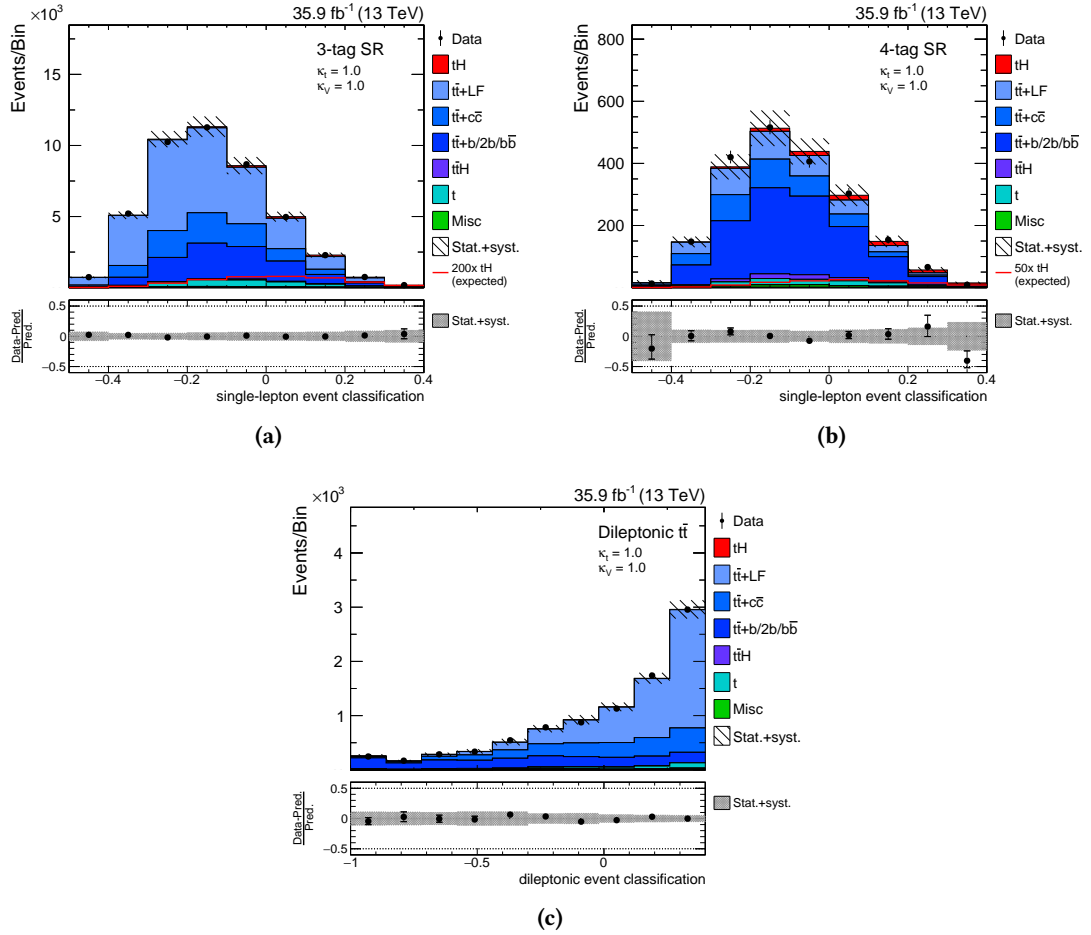
Figure 8.25: The resulting distributions after the simultaneous maximum-likelihood fit of the single-lepton event-classification output in the 3 tag (a) and 4 tag (b) signal regions, as well as the dileptonic event classification output in the dileptonic control region (c), assuming the SM coupling scenario and tH production as signal. The simulation is scaled to the result of the fit.
