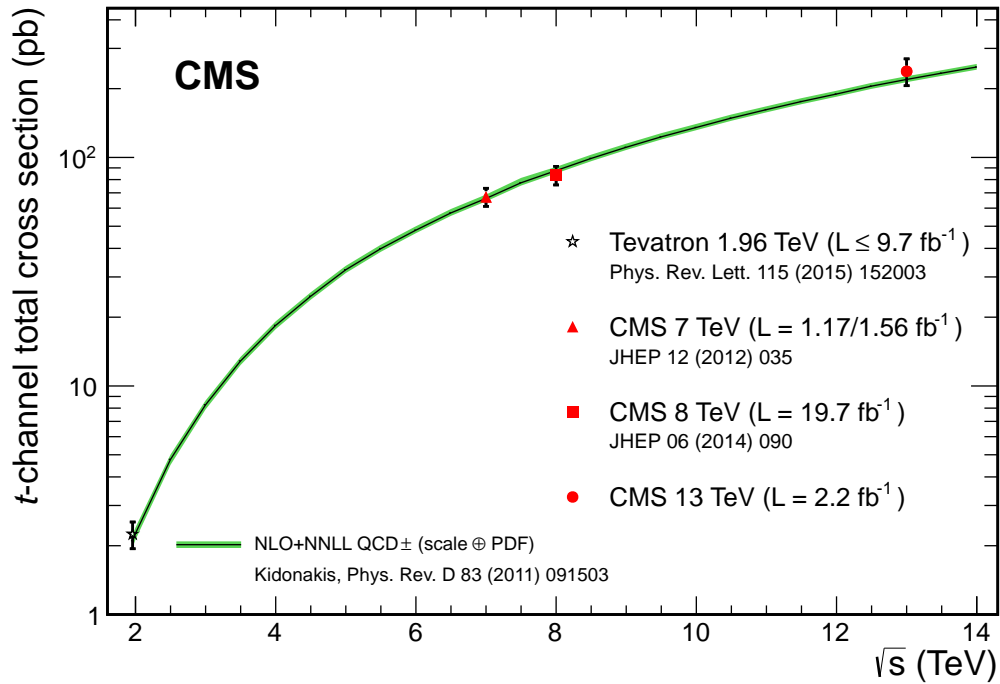
Figure 6.25: Comparison of the measured t -channel single top quark production cross section with the prediction from the theory. The measurements of the CMS Collaboration at a center-of-mass energy of 7 and 8 TeV are also shown, along with combined result at the Tevatron. All measurements are in agreement with the prediction.
