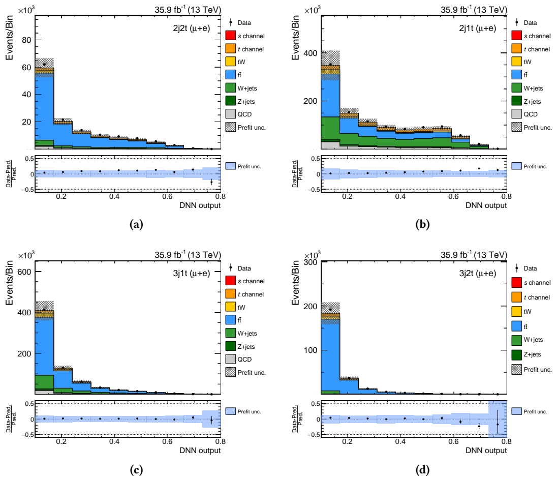
Figure 7.11. : Resulting distributions for the DNN classifier output in 2016 for the 2-jets–2-tags signal region (a), as well as the 2-jets–1-tag (b), 3-jets–1-tag (c) and 3-jets–2-tags (d) control regions. The simulation is scaled to the expected number of events.
