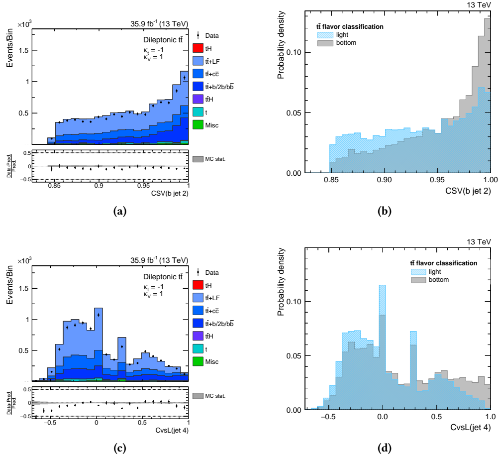
Figure C.19. : Distributions of input variables for the dileptonic event classification, ranked 4 th and 5 th in the training of the BDT: the output of the b tagging discriminant for the b-tagged jet with the second highest b tagging value in the event ((a) and (b)) and the output of the charm vs. light flavor tagging algorithm for the jet with the fourth highest momentum in the event ((c) and (d)). The distributions on the left are scaled to the expected number of events.
