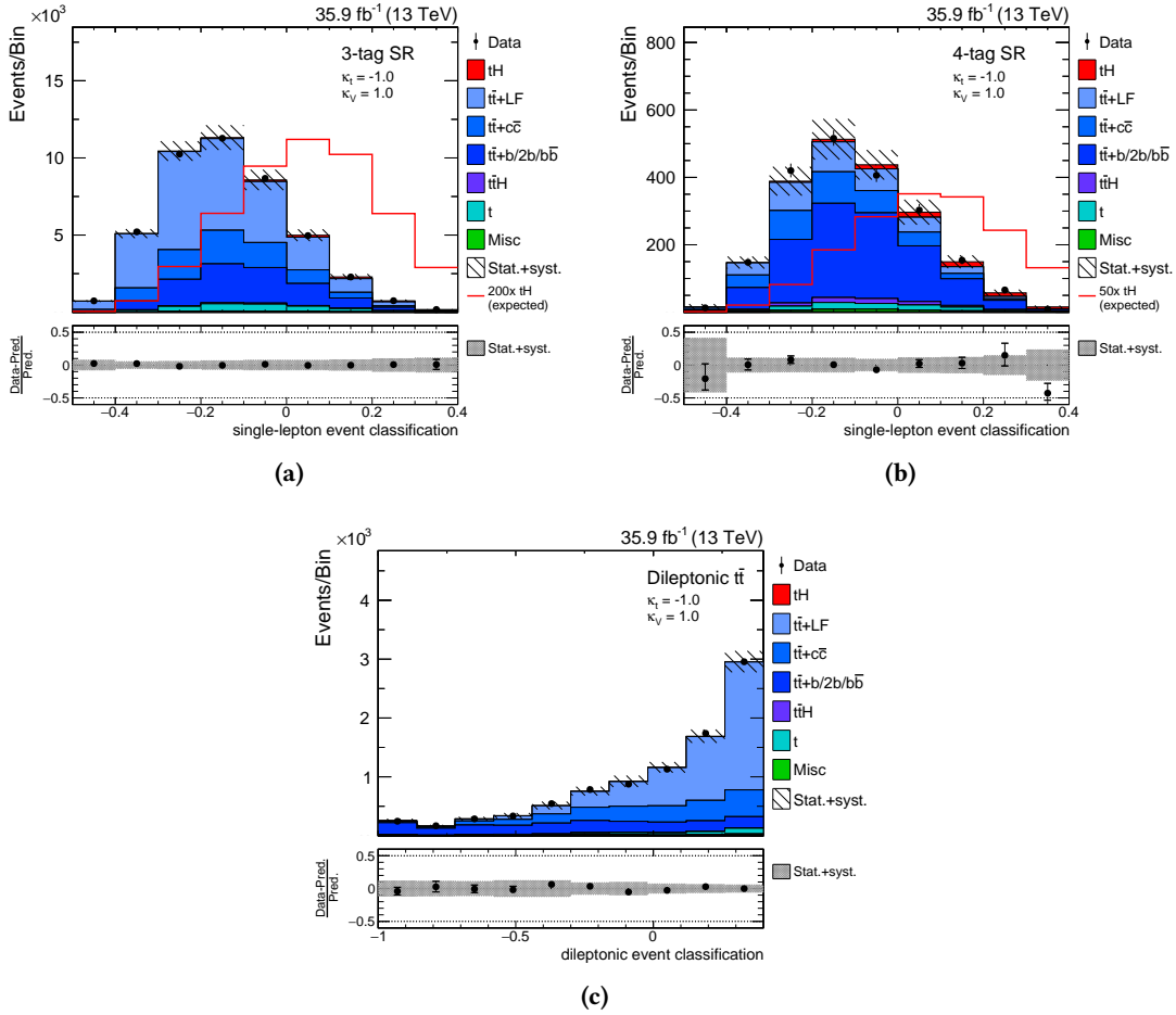
Figure 8.24: The resulting distributions after the simultaneous maximum-likelihood fit of the single-lepton event-classification output in the 3 tag (a) and 4 tag (b) signal regions, as well as the dileptonic event classification output in the dileptonic control region (c), assuming the ITC coupling scenario and tH production as signal. The simulation is scaled to the result of the fit.
