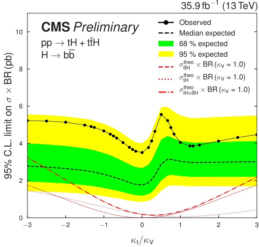
Figure 8.27.: Observed and expected 95% C.L. exclusion limits obtained for the scan over different \kappa_t/\kappa_V ratios on the combined tH+t\bar{t}H cross section times branching ratio. In addition, the exclusion curves for tH , t\bar{t}H and tH+t\bar{t}H production are shown in red (assuming \kappa_V = 1 ).
