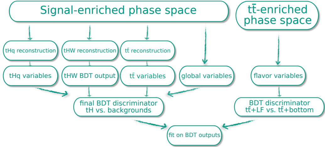
Figure 8.3.: Scheme of the analysis workflow. Events in the signal-enriched phase space are reconstructed under three different event interpretations before being classified as signal- or background-like. A similar classification is performed in a background-dominated sideband. Both distributions are used in a simultaneous maximum-likelihood fit to extract exclusion limits for associated production of a Higgs boson with a single top quark and coupling modifications.
