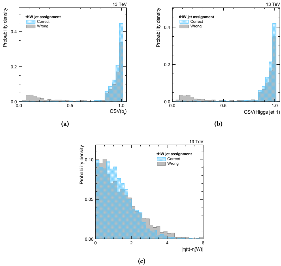
Figure C.10.: Distributions of input variables for the tHW event reconstruction, ranked 11 th to 13 th in the training of the BDT: the output of the b tagging discriminant for the jet assigned to the bottom quark from the top quark decay (a), the output of the b tagging discriminant for the jet assigned to the Higgs boson with the highest transverse momentum (b) and the absolute difference of pseudorapidities of the reconstructed top quark and the reconstructed W boson from the top quark production vertex (c).
