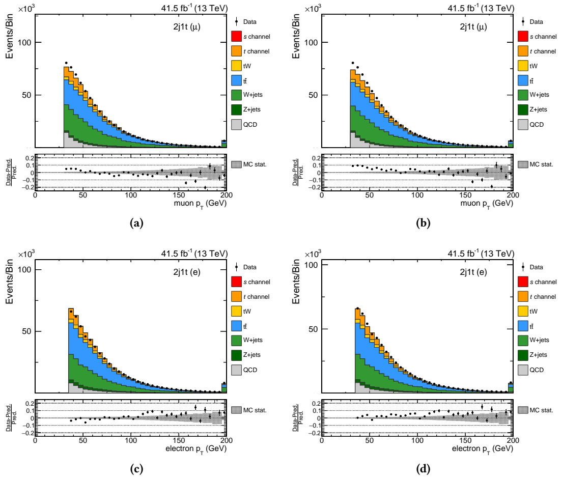
Figure B.3.: Effect of correcting the simulation for different lepton efficiencies in simulation and data of 2017.
