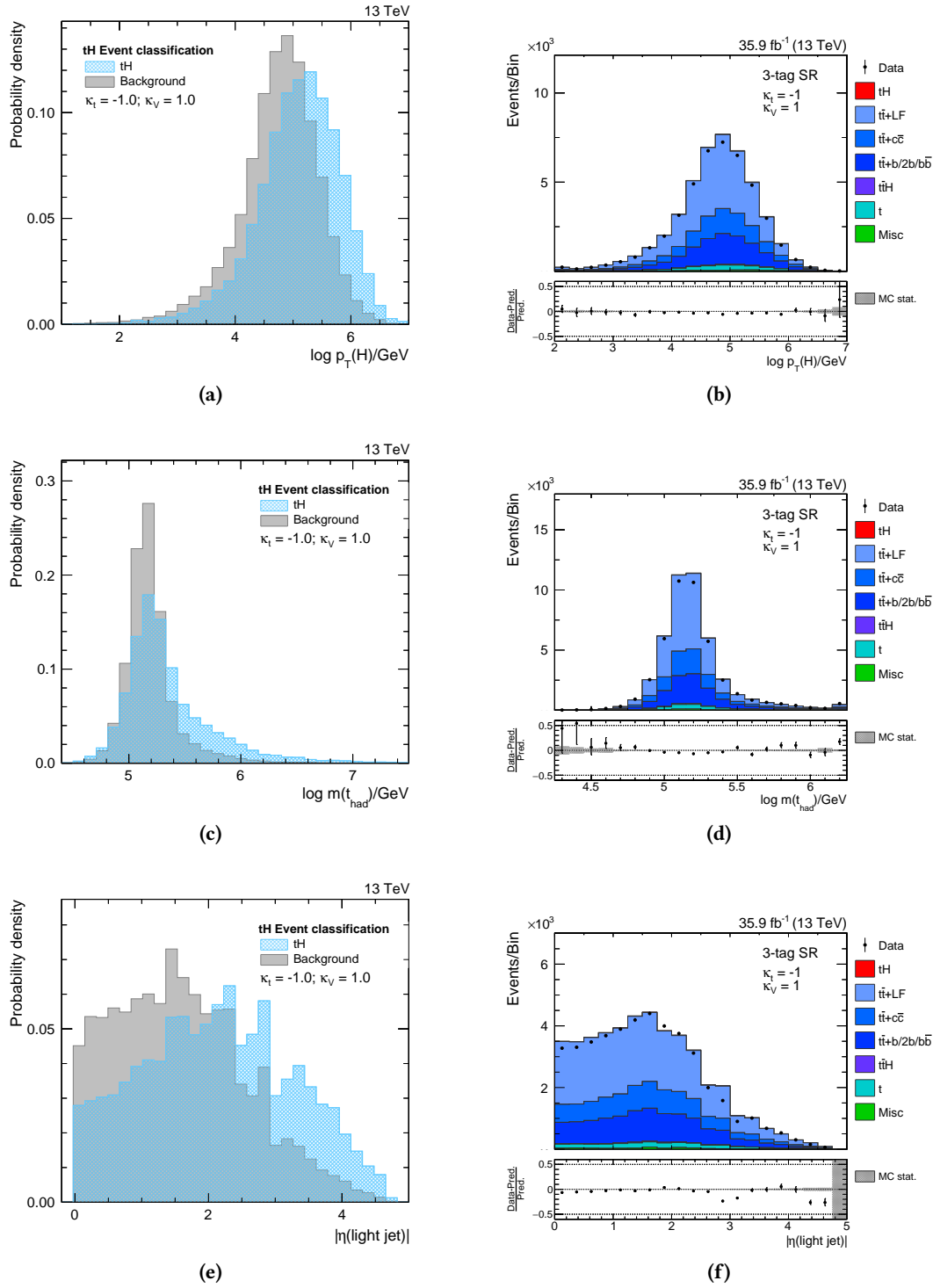
Figure 8.19: The three most important variables in the training of the single-lepton event classification. For the distributions on the right, the simulation is scaled to the expected number of events. All input variables are modeled well by the simulation.
