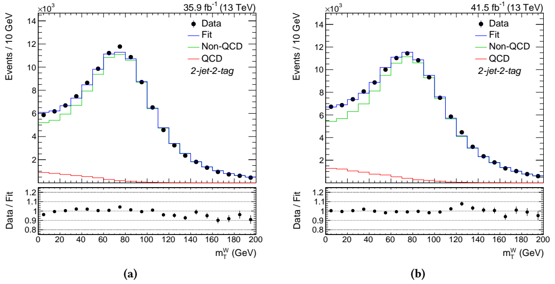
Figure 7.5.: The result of the QCD estimation from the fit to the transverse W boson mass distribution in the muon channel in 2016 (a) and 2017 (b). Good agreement between data and the fitted templates is observed for both years.
