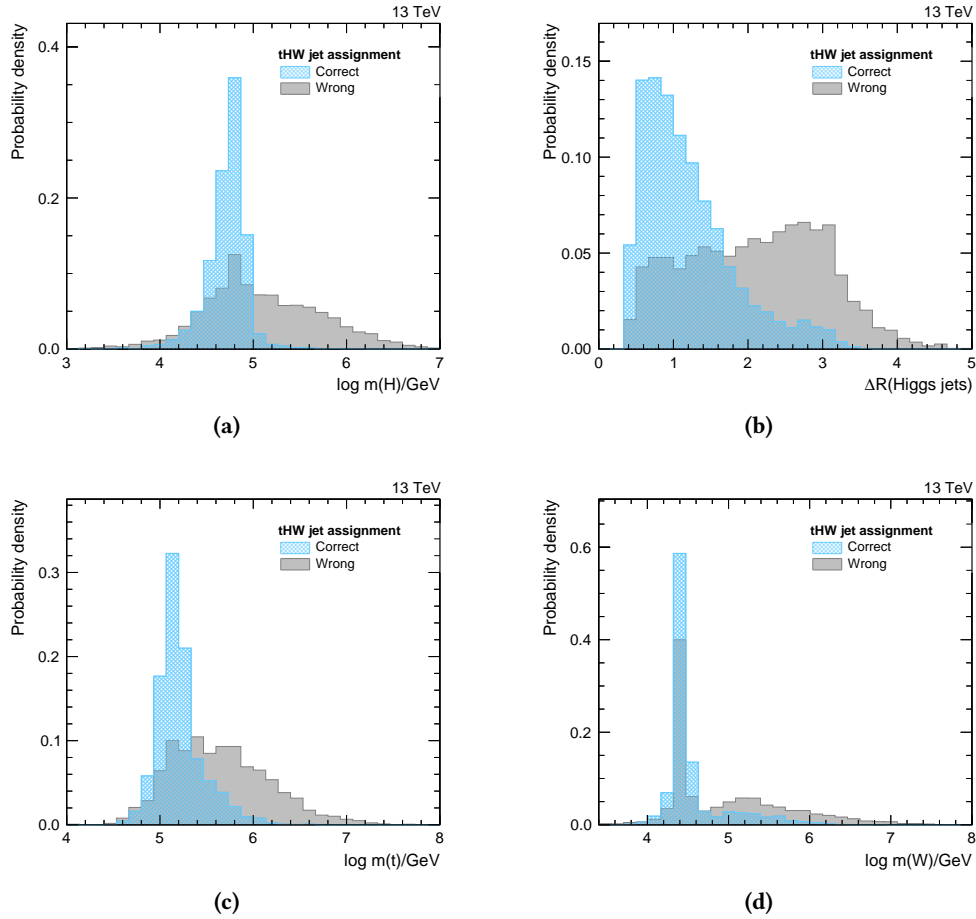
Figure C.8: Distributions of input variables for the tHW event reconstruction, ranked 1 st to 4 th in the training of the BDT: the invariant mass of the reconstructed Higgs boson (a), \Delta R between the two jets from the Higgs boson decay (b), the invariant mass of the reconstructed top quark (c) and the invariant mass of the W boson from the top quark production vertex (d).
