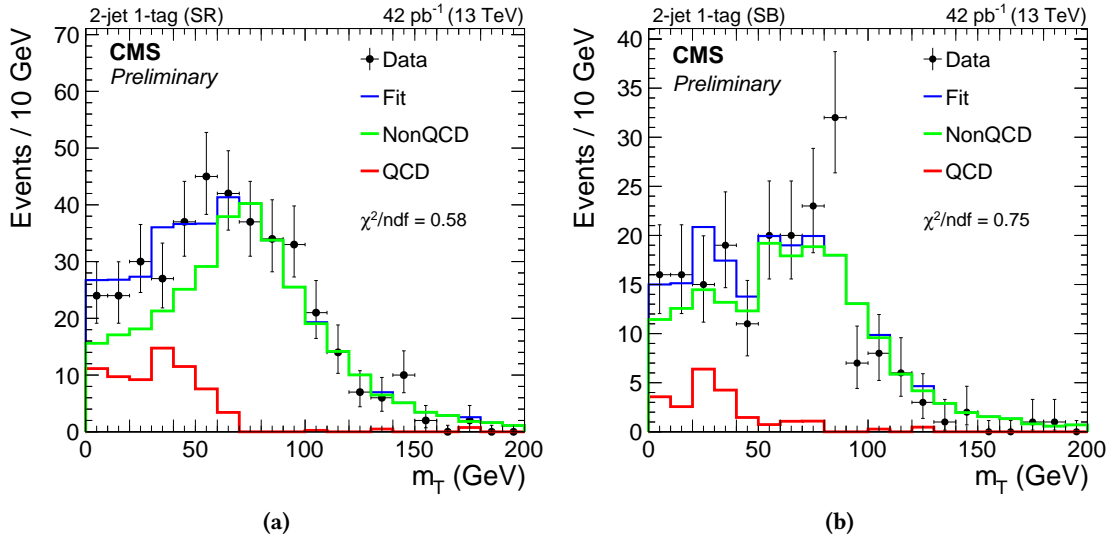
Figure 6.9.: Result of the QCD multijet background estimation in the 2-jets-1-tag region, following the description in Section 6.5, performed independently for the signal region (a) and the sideband (b). The templates are scaled to the result of the fit.
