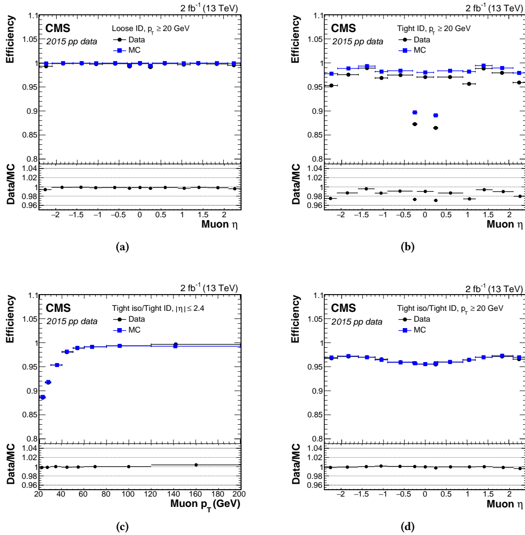
Figure 5.1.: The efficiency of muon ID and isolation requirements. The efficiency in simulation and data is shown for the loose (a) and tight muon ID (b) dependent on the pseudorapidity of the muon. Efficiencies for the combined selection of tight muon ID and tight muon isolation ( I_\mu < 0.15 ) are shown dependent on the transverse momentum of the muon (c) and the pseudorapidity of the muon (d). Differences in efficiency of simulation and data are corrected in the respective analyses.
