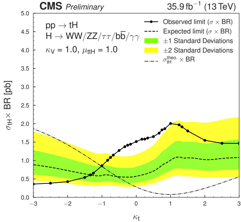
Figure 8.29.: Observed and expected 95% C.L. exclusion limits obtained for the scan over different \kappa_t/\kappa_V ratios on the tH production cross section after combining different Higgs boson decay channels. An exclusion curve for the tH production cross section times branching ratio is shown as dotted-dashed line.
