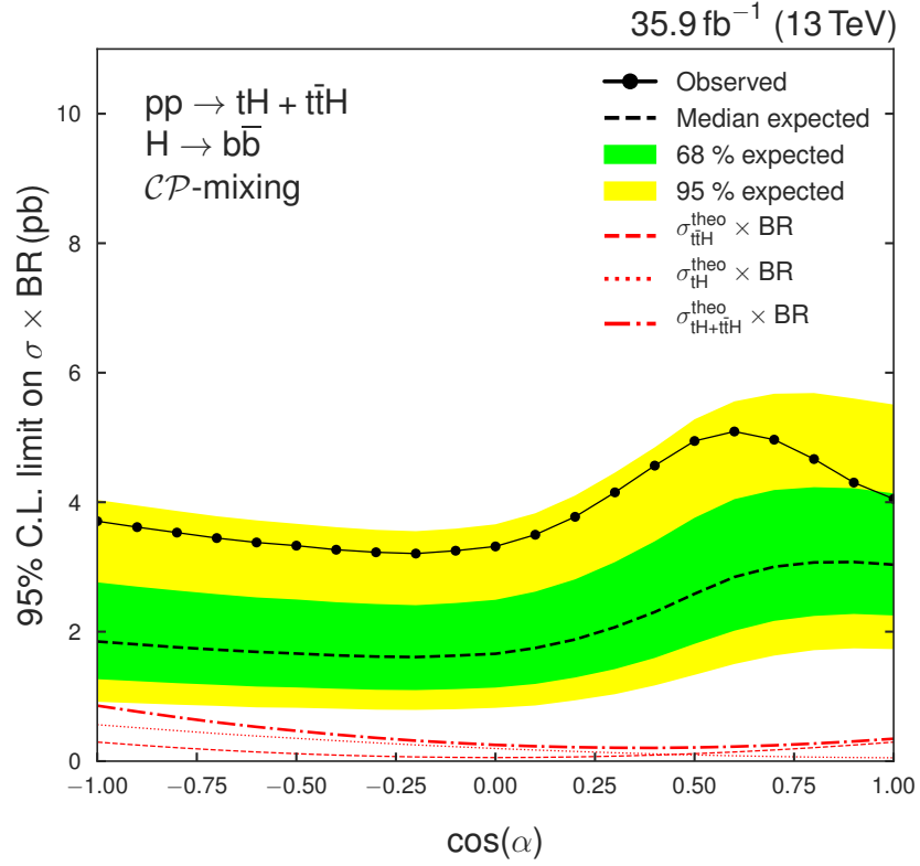
Figure 8.28. : Observed and expected 95% C.L. exclusion limits for different CP-mixing scenarios as a function of the mixing angle \alpha . In addition, the exclusion curves for tH , t\bar{t}H and tH+t\bar{t}H production are shown in red.
