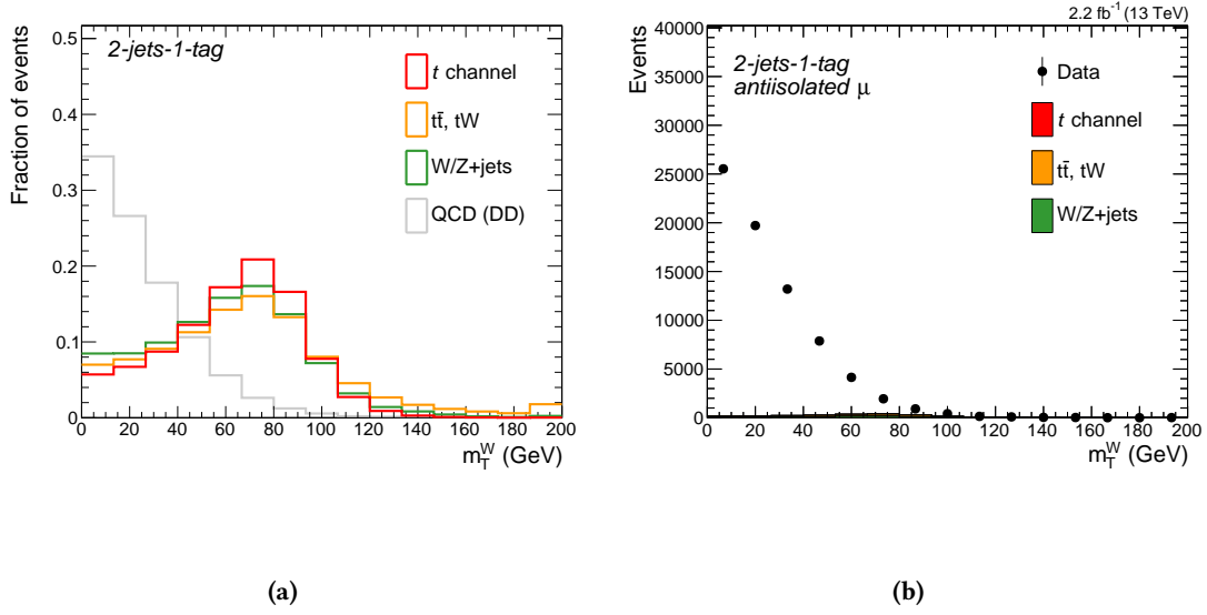
Figure 6.7.: As the distribution of the transverse W boson can distinguish between QCD multijet events and non-QCD processes (a), this variable is well suited to estimate the QCD multijet background contribution. As the size of the simulation sample for the QCD multijet background is not sufficient, a data-driven approach in an antiisolated, QCD-enriched sideband is used (b), with only minor contribution from non-QCD processes.
