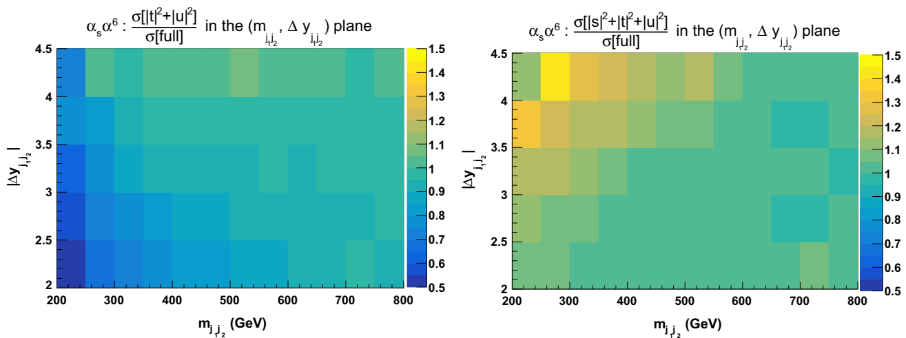
Fig. 7 Ratios for double-differential distributions in the variables m_{jj} and |\Delta y_{jj}| at NLO QCD i.e. at order \mathcal{O}(\alpha_s\alpha^6) of the approximated squared amplitudes over the full matrix element. The approximated
