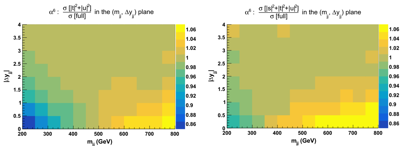
Fig. 4 Ratios for double-differential distributions in the variables m_{jj} and |\Delta y_{jj}| at LO i.e. order \mathcal{O}(\alpha^6) of approximated squared amplitudes over the full matrix element. The approximated squared amplitudes are
