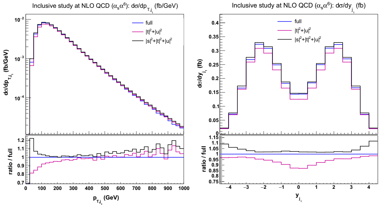
Fig. 8 Differential distributions in the transverse momentum (left) and rapidity (right) of the hardest tagging jet at NLO QCD i.e. at order \mathcal{O}(\alpha_s\alpha^6) for the full computation and two approximations. The upper plots provide the absolute value for each prediction while the lower
