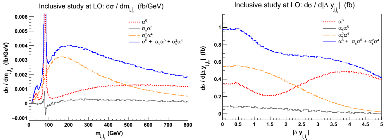
Fig. 2 Differential distribution in the di-jet invariant mass m_{jj} (left) and the difference of the jet rapidities |\Delta y_{jj}| (right) for the three LO contributions to the process pp \rightarrow \mu^+ \nu_\mu e^+ \nu_e jj . The EW contribution
