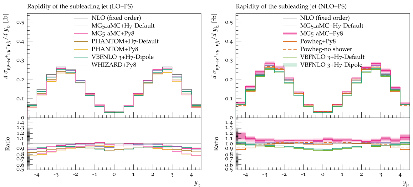
Fig. 18 Differential distribution in the rapidity of the second-hardest jet from predictions matched to parton showers, at LO (left) or NLO (right) accuracy (upper plot), compared with the fixed-NLO result computed with VBFNLO (lower plot). At NLO+PS accuracy, for VBFNLO+HERWIG7- DIPOLE, the three-point scale uncertainties are
