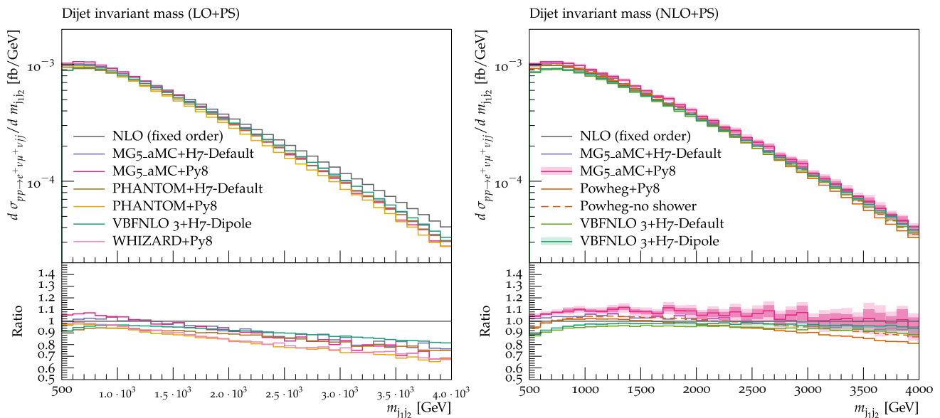
Fig. 14 Differential distribution in the invariant mass of the two tagging jets from predictions matched to parton showers, at LO (left) or NLO (right) accuracy (upper plot), compared with the fixed-NLO result computed with VBFNLO (lower plot). At NLO+PS accuracy, for VBFNLO+HERWIG7- DIPOLE, the three-point scale uncertainties are
