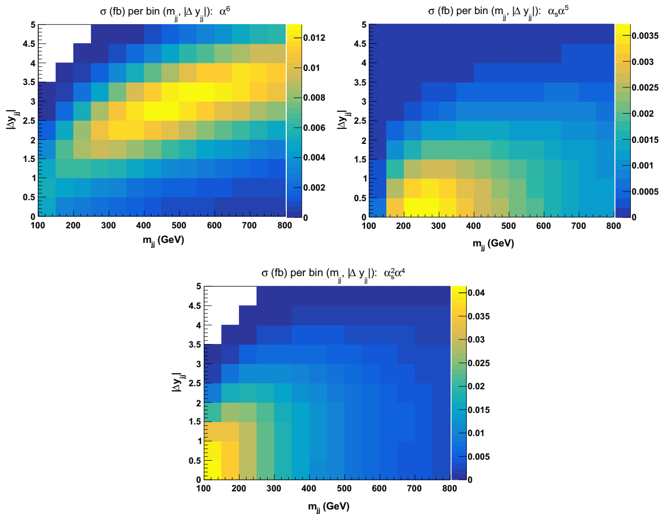
Fig. 3 Double-differential distributions in the variables m_{jj} and |\Delta y_{jj}| for the three LO contributions of orders \mathcal{O}(\alpha^6) (top left), \mathcal{O}(\alpha_s \alpha^5) (top right), and \mathcal{O}(\alpha_s^2 \alpha^4) (bottom). The cuts applied are the ones of Sect. 3.3 but no cuts on m_{jj} and |\Delta y_{jj}| are applied
