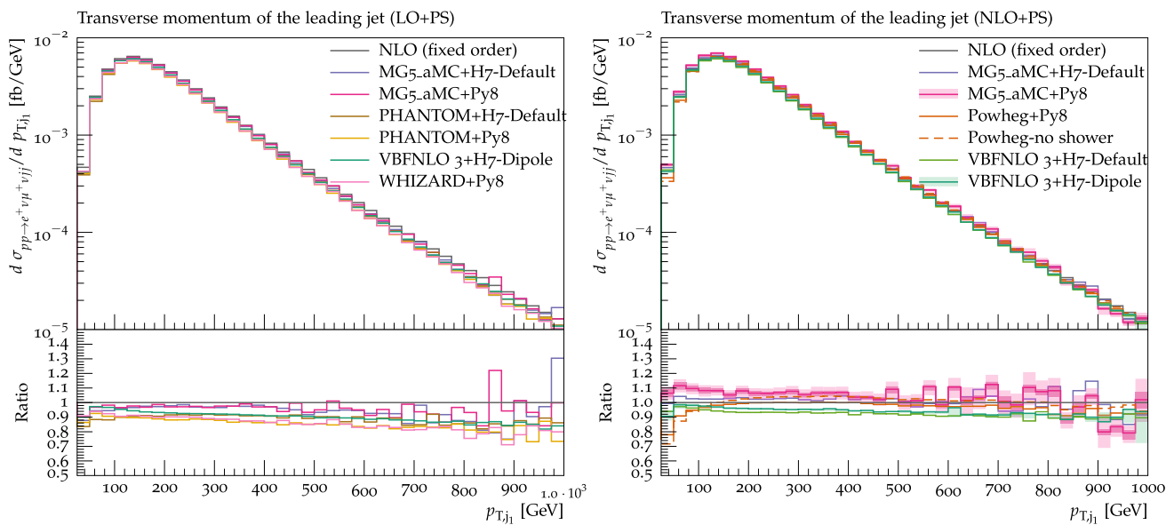
Fig. 16 Differential distribution in the transverse momentum of the hardest jet from predictions matched to parton showers, at LO (left) or NLO (right) accuracy (upper plot), compared with the fixed-NLO result computed with VBFNLO (lower plot). At NLO+PS accuracy, for VBFNLO+HERWIG7- DIPOLE, the three-point scale uncertainties are
