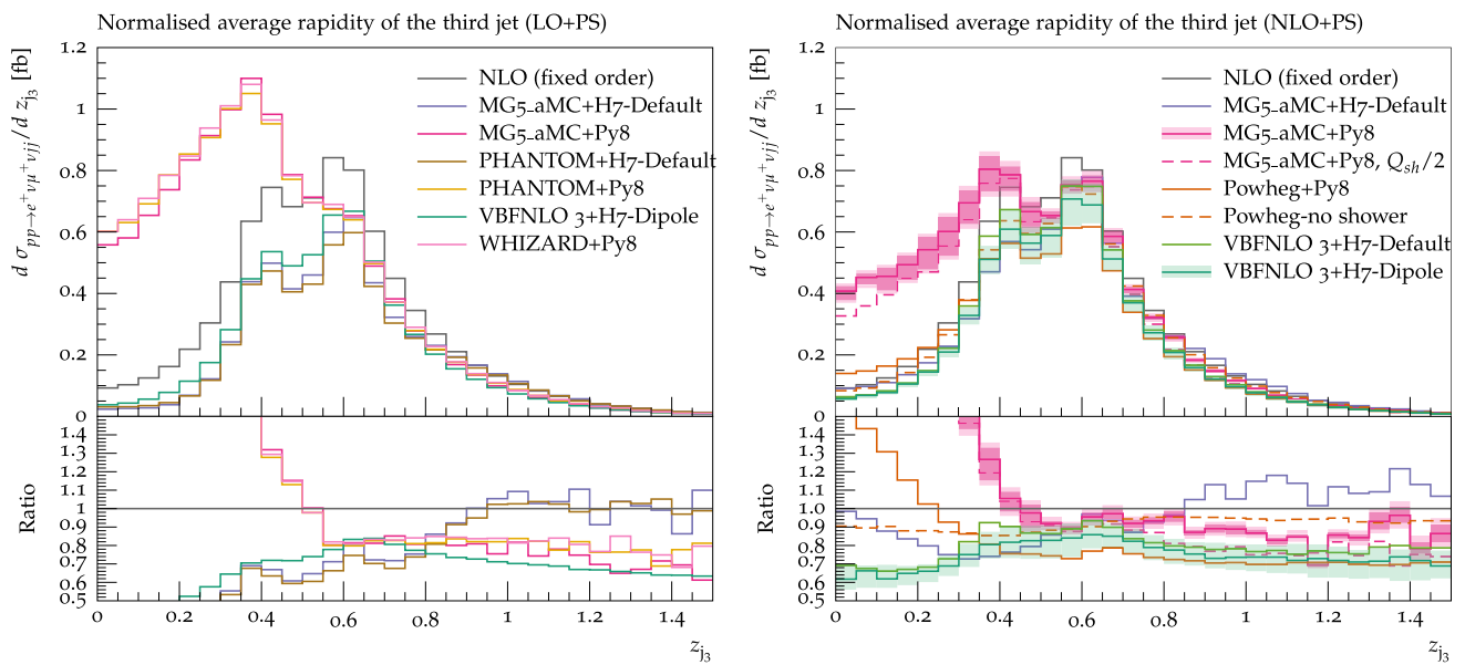
Fig. 19 Differential distribution in the Zeppenfeld variable of the third-hardest jet from predictions matched to parton showers, at LO (left) or NLO (right) accuracy (upper plot), compared with the fixed-NLO result computed with VBFNLO (lower plot). At NLO+PS accuracy, for VBFNLO+HERWIG7- DIPOLE, the three-point scale uncertainties are
