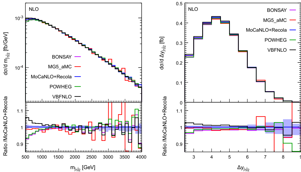
Fig. 10 Differential distributions in the invariant mass (left) and rapidity difference (right) of the two tagging jets at NLO accuracy i.e. at order \mathcal{O}(\alpha_s\alpha^6) . The description of the different programs used can be found in Sect. 3.2. The upper plots provide the absolute value for each prediction while the lower plots present all predictions normalised
