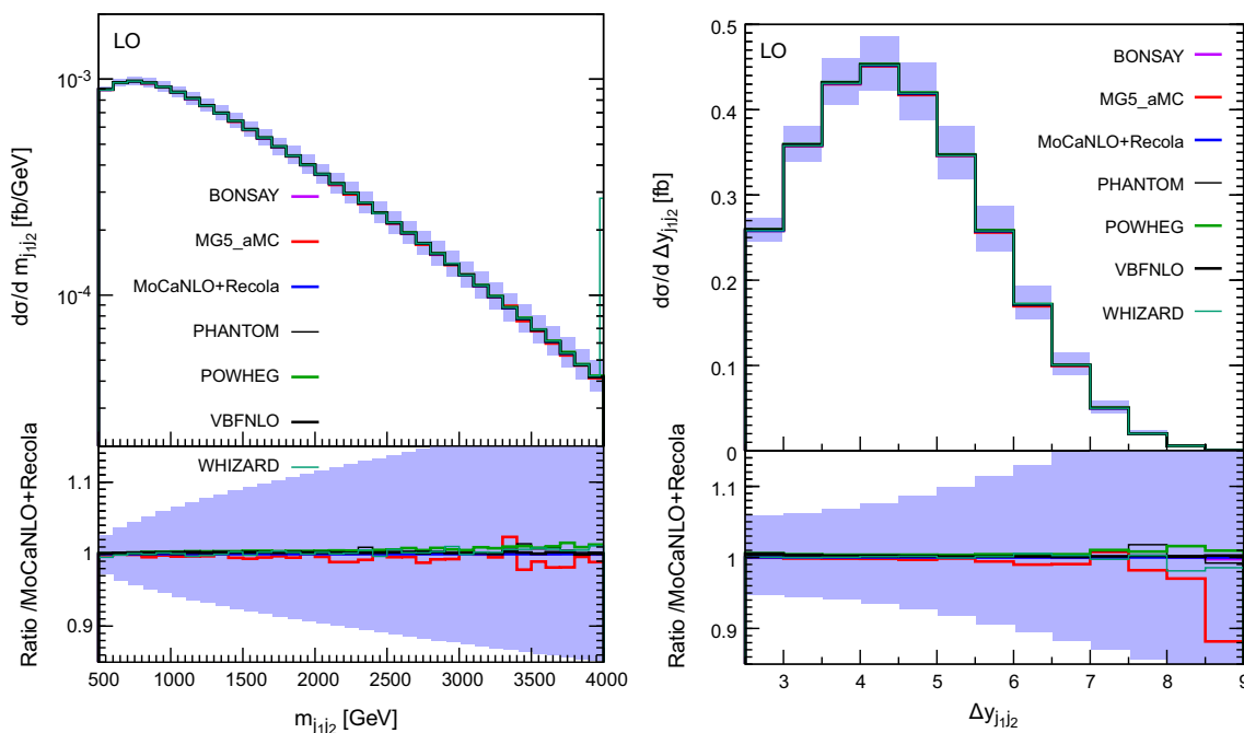
Fig. 5 Differential distributions in the invariant mass (left) and rapidity difference of the two tagging jets (right) at LO accuracy i.e. at order \mathcal{O}(\alpha^6) . The description of the different programs used can be found in Sect. 3.2. The upper plots provides the absolute value for each prediction while the lower plots presents all predictions normalised to
