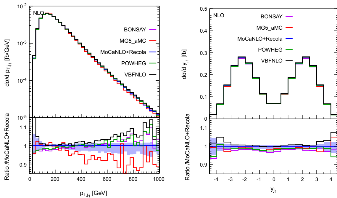
Fig. 11 Differential distributions in the transverse momentum (left) and rapidity (right) of the hardest jet at NLO accuracy i.e. at order \mathcal{O}(\alpha_s\alpha^6) . The description of the different programs used can be found in Sect. 3.2. The upper plots provide the absolute value for each prediction while the lower plots present all predictions normalised to
