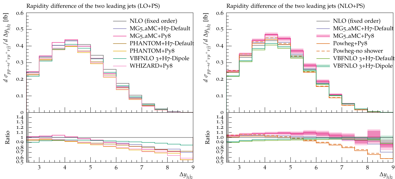
Fig. 15 Differential distribution in the rapidity separation of the two tagging jets from predictions matched to parton showers, at LO (left) or NLO (right) accuracy (upper plot), compared with the fixed-NLO result computed with VBFNLO (lower plot). At NLO+PS accuracy, for VBFNLO+HERWIG7- DIPOLE, the three-point scale uncertainties are
