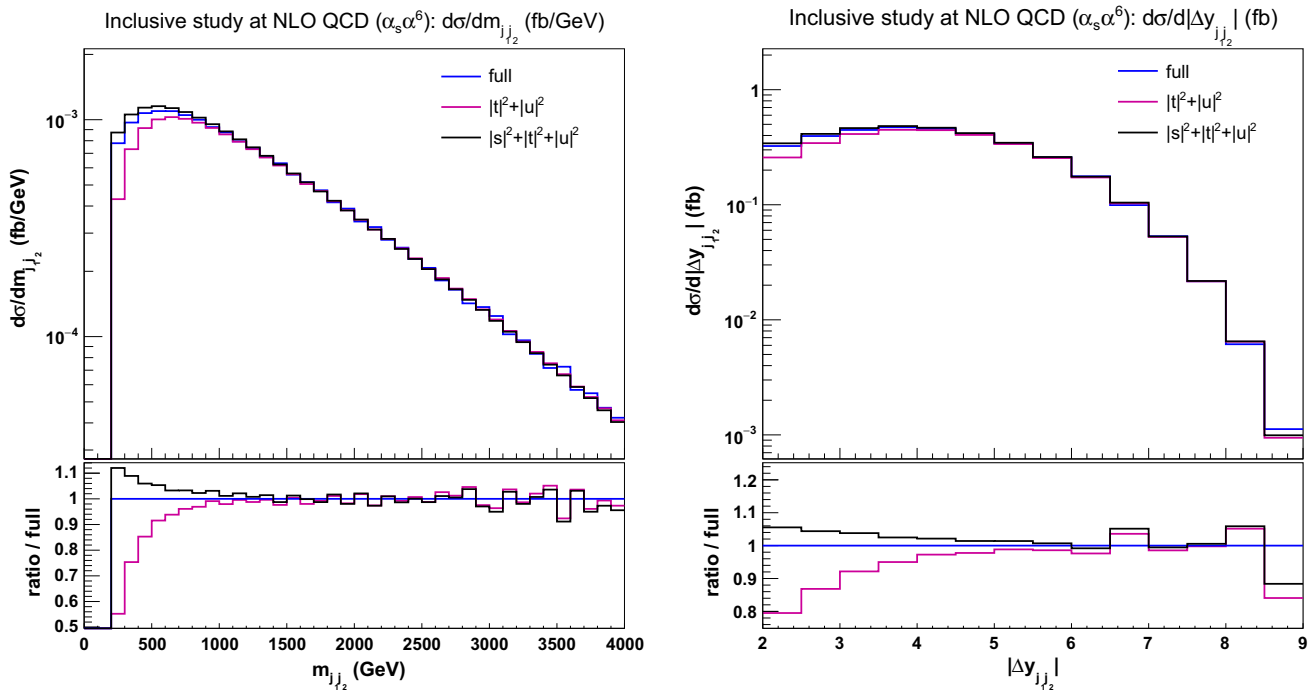
Fig. 6 Differential distributions in the di-jet invariant mass (left) and the rapidity separation (right) of the two tagging jets at NLO QCD i.e. at order \mathcal{O}(\alpha_s\alpha^6) for the full computation and two approximations. The upper plots provide the absolute value for each prediction while the
