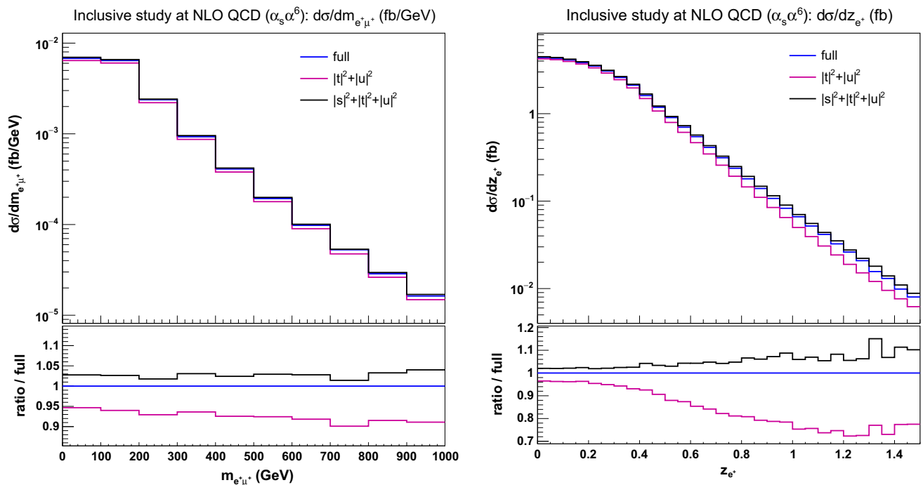
Fig. 9 Differential distributions in the lepton-lepton invariant mass (left) and the electron Zeppenfeld variable (right) at NLO QCD i.e. at order \mathcal{O}(\alpha_s\alpha^6) for the full computation and two approximations. The upper plots provide the absolute value for each prediction while the
