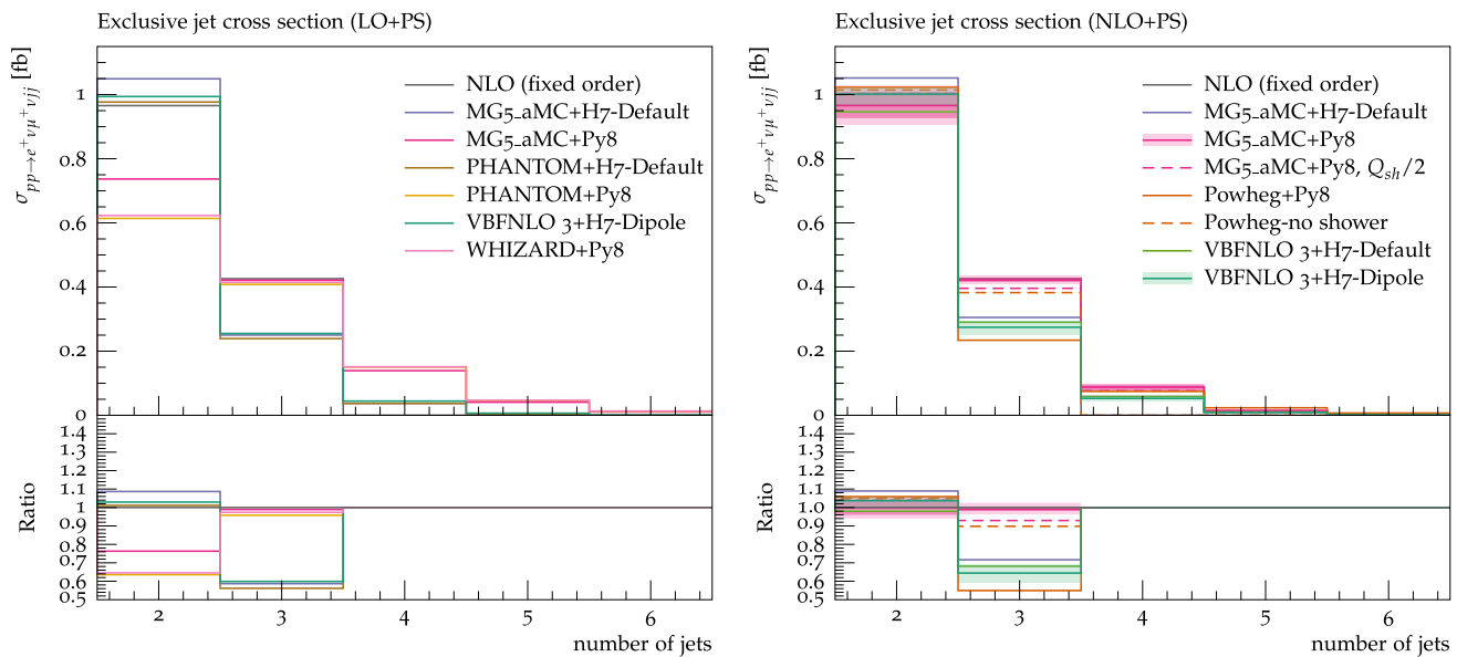
Fig. 13 Differential distribution in the exclusive jet multiplicity from predictions matched to parton showers, at LO (left) or NLO (right) accuracy (upper plot), compared with the fixed-NLO result computed with VBFNLO (lower plot). At NLO+PS accuracy, for VBFNLO+HERWIG7-DIPOLE, the three-point scale uncertainties are
