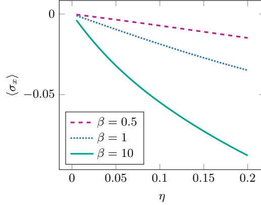
Figure 3.2.: The expectation value of \sigma_x is plotted as a function of the coupling strength \eta . Values of further parameters are \Delta E = 1 , \omega_c = 10 . Reprinted with permission of Ref. [VI]. Copyright (2016) by the American Physical Society.
