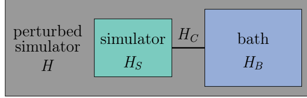
Figure 2.1.: This figure gives a schematic overview of the general setting considered in this work. The full system described by Hamiltonian H is formed by the simulator ( H_S ) that is coupled to external degrees of freedom, which we call bath ( H_B ). The coupling is characterized by the coupling Hamiltonian H_C .
