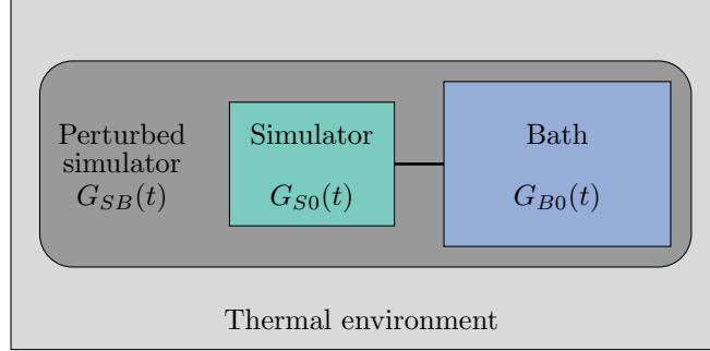
Figure 5.1.: We study a simulator that is perturbed by a bath containing unwanted external degrees of freedom. The whole system is in thermal equilibrium. The different parts of our system are associated with corresponding Green’s functions: the ideal Green’s function of the simulator iG_{S0}(t) = \langle \mathcal{T} \hat{O}(t) \hat{O}(0) \rangle_0 (see Eq. (5.1)) and the free Green’s function of the bath iG_{B0}(t) = \langle \mathcal{T} \hat{X}(t) \hat{X}(0) \rangle_0 . The perturbed simulator is related to the full Green’s function iG_{SB}(t) = \langle \mathcal{T} \hat{O}(t) \hat{O}(0) \rangle . Reprinted with permission of Ref. [I]. Copyright (2018) by the American Physical Society.
