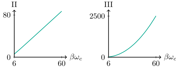
Figure 3.1.: The graphs show the \beta dependence of diagrams II and III (for \eta = 1 ). Reprinted with permission of Ref. [VI]. Copyright (2016) by the American Physical Society.
