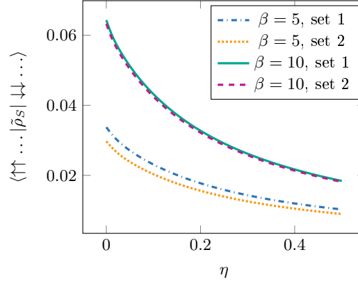
Figure 3.4.: We show the matrix element \langle \uparrow \uparrow \dots | \tilde{\rho}_S | \downarrow \downarrow \dots \rangle as function of the coupling strength \eta . The matrix element decreases strongly with increasing \eta . This graph displays exemplary results for two sets of random variables \xi_1^{(i,j)}, \xi_2^{(i)} (Gaussian random numbers with mean value 1 and variance 0.2 / 0.1) for two temperatures. Further parameters are \epsilon = 0.5 ; \Delta = 3 ; \omega_c = 15 ; J_{ij} = -3.01 for the connections shown in Fig. 3.3, otherwise J_{ij} = 0 . Reprinted with permission of Ref. [VI]. Copyright (2016) by the American Physical Society.
