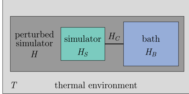
Figure 2.2.: This figure illustrates the general setting of a perturbed simulator in thermal equilibrium. The simulator is connected to a bath that represents the external degrees of freedom creating the perturbation. Additionally, this perturbed simulator couples infinitesimally small to another bath that has no other effect on the system than to create a thermal equilibrium with temperature T .
