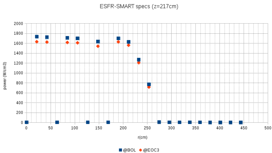
Figure 6. Power density radial distribution in ESRF-SMART: at BOL and End Of Cycle 3 (EOC3).
