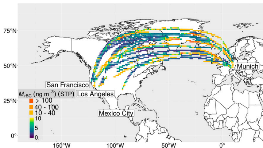
Fig. 1. Spatial distribution of M_{rBC} between Europe and North America in the LMS as obtained by 22 CARIBIC flights flying between Munich and San Francisco, between Munich and Los Angeles, and between Munich and Mexico City from August 2014 through October 2015. Flights mainly cover the region of 123.75°W–11.25°E and 35°N–77°N. The M_{rBC} data have been converted to STP conditions (273.15 K, 1,013.25 hPa) on a 1^\circ \times 1^\circ grid.
