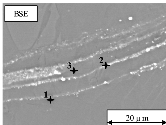
Figure 6. SEM micrograph obtained using the BSE mode of the as-received Mg-10Gd. Several lines of particles are curved inside the TZ and DZ of the Mg-10Gd material. EDS analysis was done at the three positions indicated to determine the Gd content.
