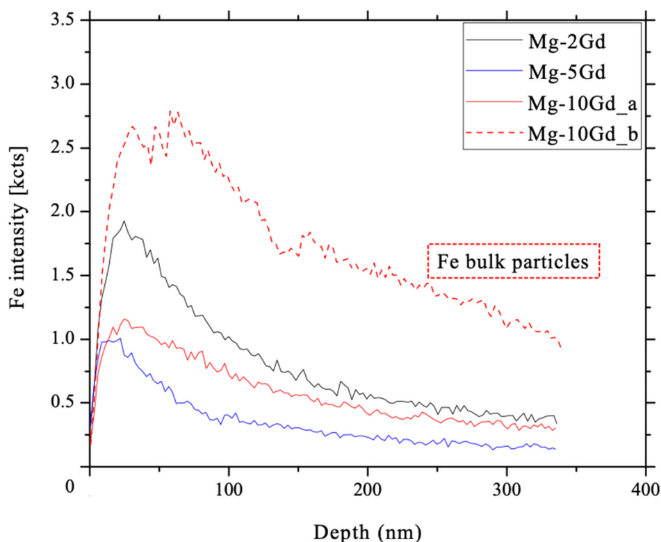
Figure 10. Depth profiles for Fe in the sub-surface of as-received Mg-xGd alloys. The Fe intensity decreases at a depth around 30 nm. One profile of each alloy (Mg-2Gd, Mg-5Gd, Mg-10Gd_a) is plotted and show the decrease of Fe intensity to be virtually zero for the case of Fe surface contamination. The decrease of Mg-10Gd_b is not virtually zero after around 340 nm, due to additional bigger Fe particles inside the bulk.
