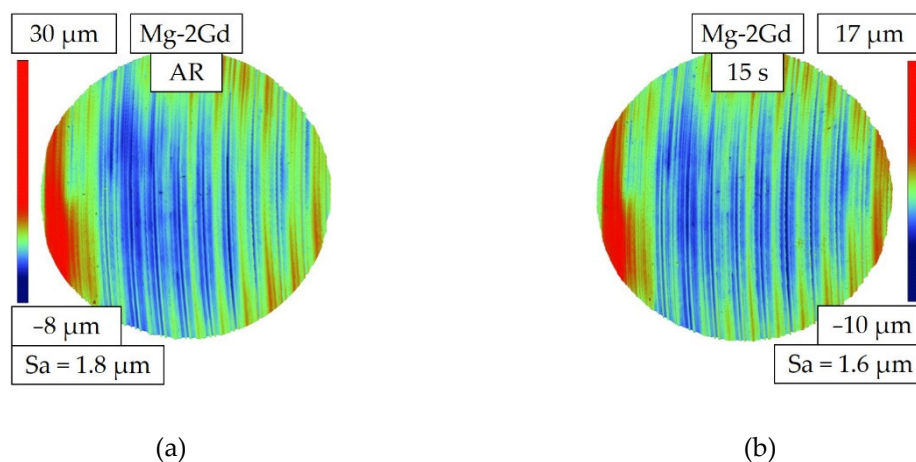
Figure 8. Topographies of the Mg-2Gd alloy as measured by white light interferometry (WLI): (a) Topography in as-received (AR) state with machining marks and a peak-valley difference of 38 (30 μm to -8 μm) (b) Topography after etching with 250 g/L HAc for 15 s in 5 mL of solution. Machining marks are still visible and the peak-valley difference of 27 μm (17 μm to -10 μm) is reduced in as compared to the AR state.
