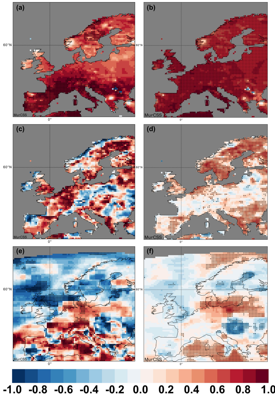
Figure 6. Spatial distribution of the ACC for the multi-annual mean anomalies of lead years 1–5 in MPI_b1 for (a, b) temperature, (c, d) precipitation, and (e, f) wind speed. For (a, c, e) five start years (dec1960, dec1970, dec1980, dec1990, dec2000) have been used, while for (b, d, f) all start years from dec1960 to dec2000 are taken into account. The black dots indicate significant skill at the 95 % level (bootstrapping). For more details see the main text.
