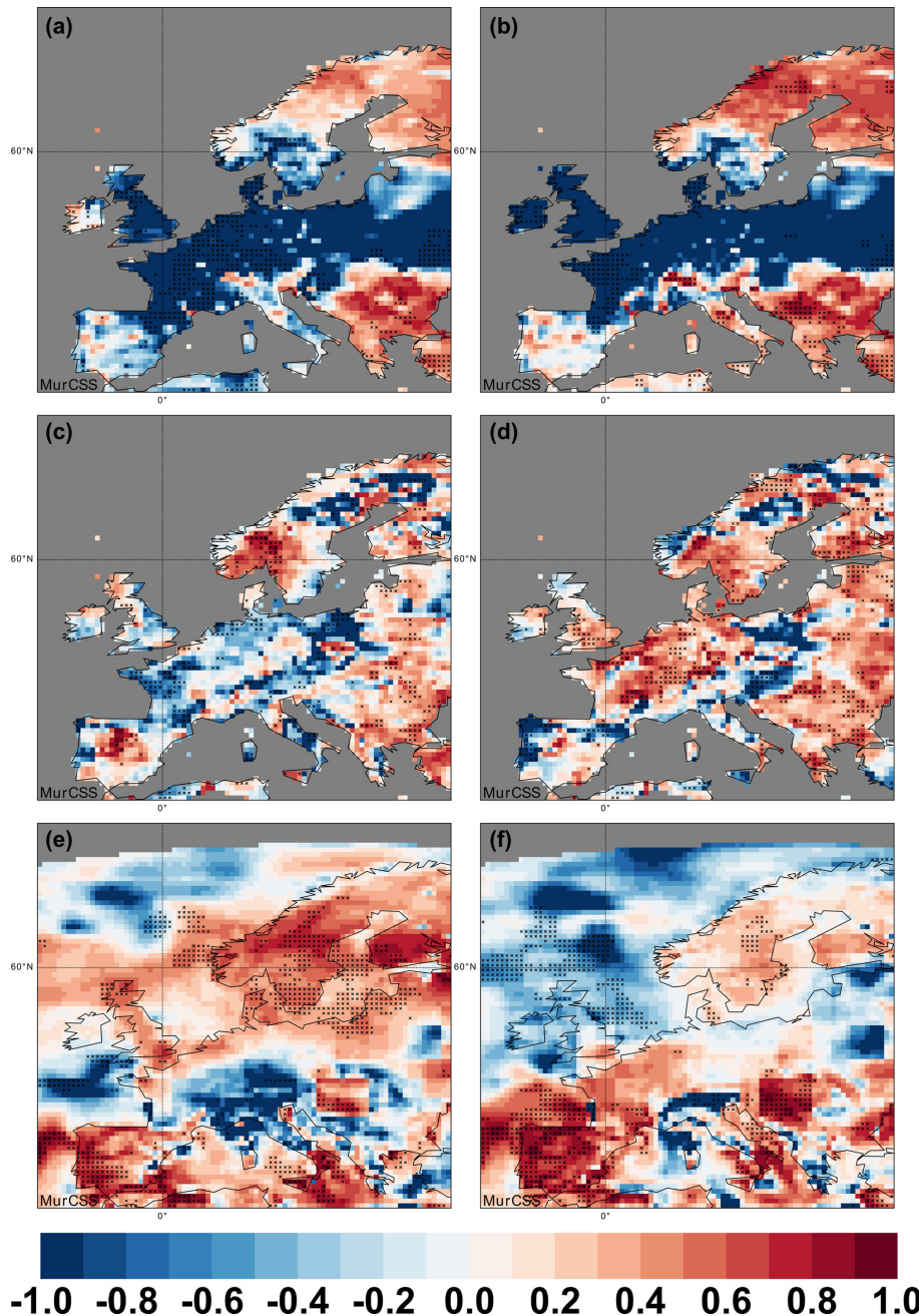
Figure 3. Spatial distribution of the MESS for the multi-annual mean anomalies of lead years 1–5 for (a) temperature in CCLM_b0, (b) temperature in CCLM_b1, (c) precipitation in CCLM_b0, (d) precipitation in CCLM_b1, (e) wind speed in CCLM_b0, and (f) wind speed in CCLM_b1. As reference dataset we have used the uninitialized historical ensemble. The black dots indicate significant skill at the 95 % level (bootstrapping).
