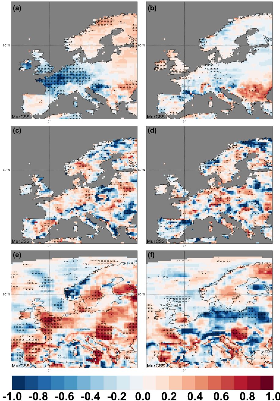
Figure 4. Spatial distribution of the MSESS for the multi-annual mean anomalies of lead years 1–5 for (a) temperature in CCLM_b0, (b) temperature in CCLM_b1, (c) precipitation in CCLM_b0, (d) precipitation in CCLM_b1, (e) wind speed in CCLM_b0, and (f) wind speed in CCLM_b1. As reference dataset we have used the respective global MPI data. The black dots indicate significant skill at the 95 % level (bootstrapping).
