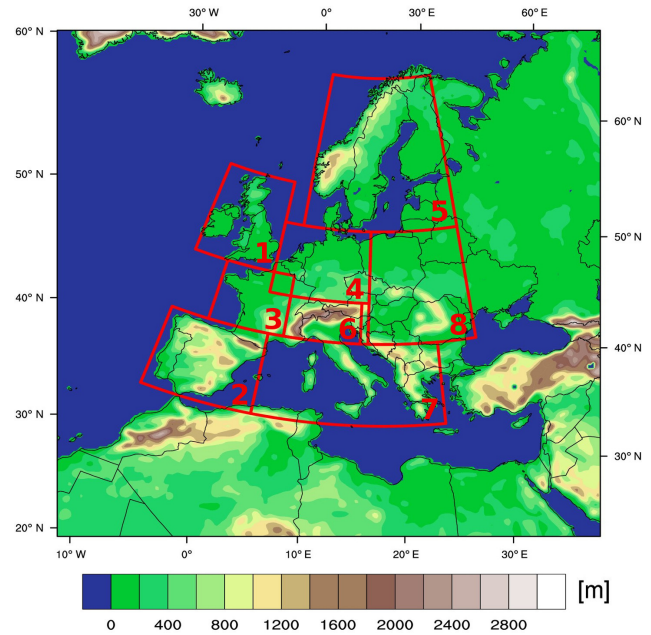
Figure 1. CCLM modelling domain (EURO-CORDEX domain): Model orography and PRUDENCE regions. 1: British Isles, BI; 2: Iberian Peninsula, IP; 3: France, FR; 4: Mid-Europe, ME; 5: Scandinavia, SC; 6: Alps, AL; 7: Mediterranean, MD; and 8: eastern Europe, EA.
