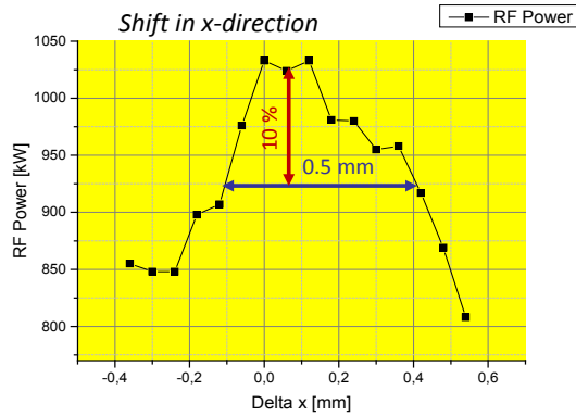
Fig. 4. Influence of the electron beam deviation (x-direction) on the RF power measurements carried out on the SP gyrotron.
