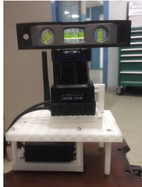
Fig. 2. Hokuyo laser on a stand. Laser is strictly parallel to the surface of the floor.
