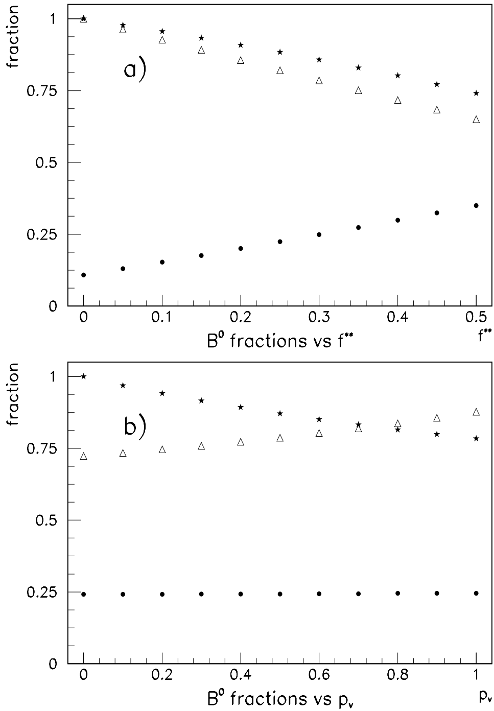
Figure 4: Predicted fraction of B^0 mesons in the samples of \bar{D}^0 \ell^+ events ( \bullet ), D^- \ell^+ events ( \triangle ) and D^{*-} \ell^+ events ( \star ) as a function of (a) f^{**} with p_v = 0.54 and (b) p_v with f^{**} = 0.36 .
