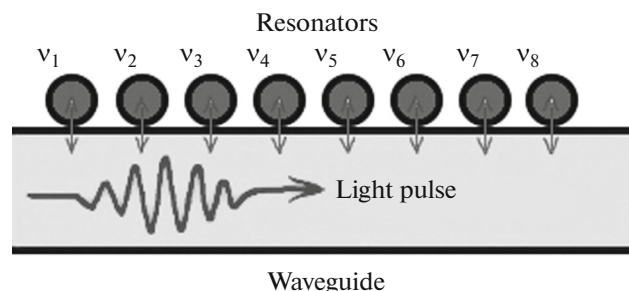
Fig. 1. MR scheme of quantum memory. The waveguide is coupled to a system of resonators through slits in the wall. The distance between neighboring resonators is equal to the wavelength, and the frequencies of the resonators form a periodic structure. The frequency and Q -factor of each resonator can be controlled independently.
