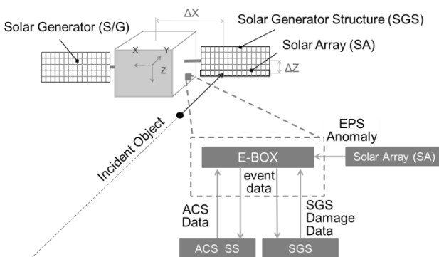
Figure 2: Functional principle of SOLID concept
