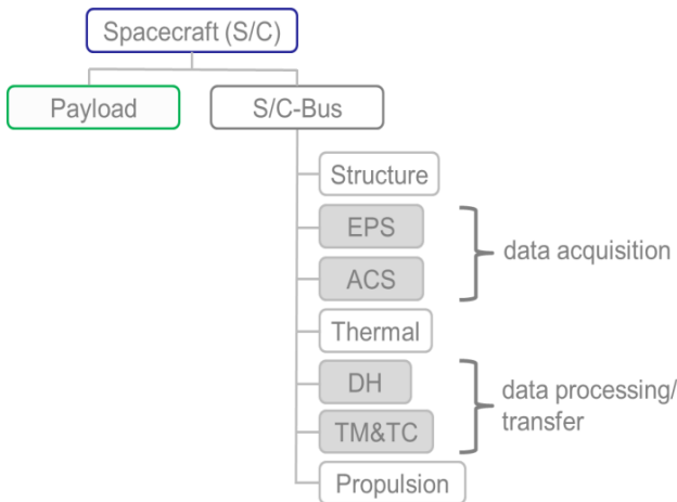
Figure 1: S/C Subsystems Adaptation
