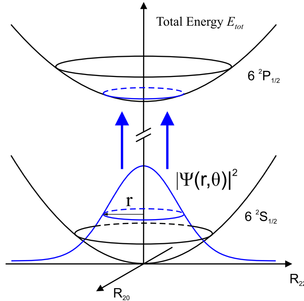
FIG. 4. Energy diagram for the Ba + D_1 transition (excitation) perturbed by quadrupolar bubble oscillations. Potential energy surfaces are plotted for the fixed parameters \alpha and R_0 obtained from ABM and corresponding to 6s\ ^2S_{1/2} state. For clarity, calculated potential energy surfaces for the D_1 emission are not drawn.
