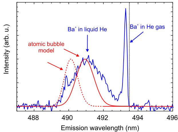
FIG. 7. Observed emission spectrum of \text{Ba}^+ ions in superfluid He. D_1 ( 6p^2P_{1/2} - 6s^2S_{1/2} ) transition, T = 2.13 K, ablation at 10 Hz, f_{dis} = 3.3 kHz, \tau_{dis} = 10 \mu\text{s} , E_{\perp} = 3200 V/cm. Red curve is a calculated spectrum of \text{Ba}^+ in liquid He according to the atomic bubble model (solid curve for pair potentials, 7,26 dashed curve for pair potentials 23 ). Vertical dashed line indicates the wavelength of the D_1 transition in a free ion.
