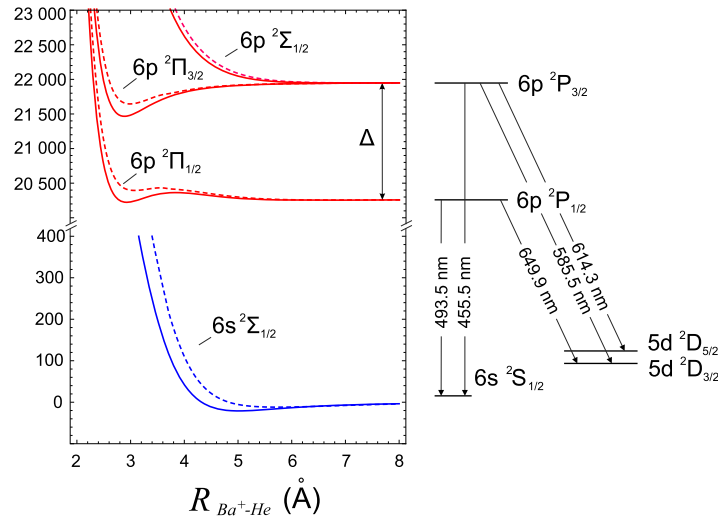
FIG. 1. Left side: Adiabatic Ba + -He pair-potentials with the spin-orbit interaction included. Dashed curves - pair potentials taken from Ref. 23, solid curves - pair potentials taken from Refs. 7 and 26. Right side: Energy levels and electronic transitions of a free Ba + ion.
