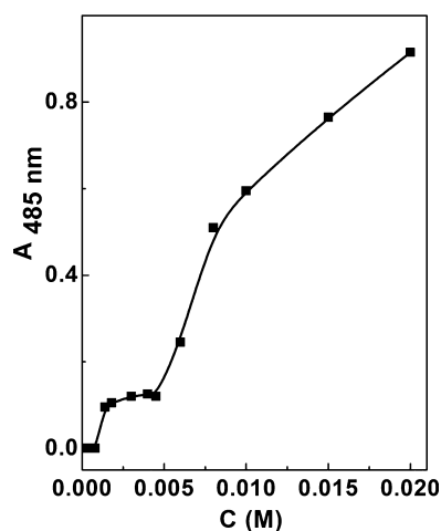
Fig. 7. Optical density of Sudan I in aqueous solutions of CS 2 vs. concentration of CS 2 at fixed CR concentration of 0.5 mM; \lambda = 485 nm; L = 0.1 cm; 25 °C.
