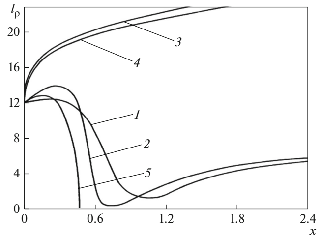
Fig. 3. Changing of a cross-section of the wave beam under its propagation in the x -direction: (1) \lambda = 1 , \varepsilon = 1.34 ; (2) \lambda = 1 , \varepsilon = 2.24 ; (3) \lambda = -1 , \varepsilon = 1.34 ; (4) \lambda = -1 , \varepsilon = -1.34 ; (5) \lambda = 0 , \varepsilon = -1.34 .
