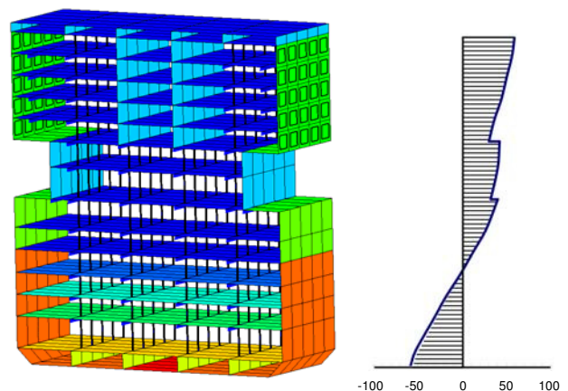
Figure 1. Main frame of modern passenger ship with large balcony openings and several pillar lines (left) leads to low shear stiffness and non-linear distribution of normal stress (right).
