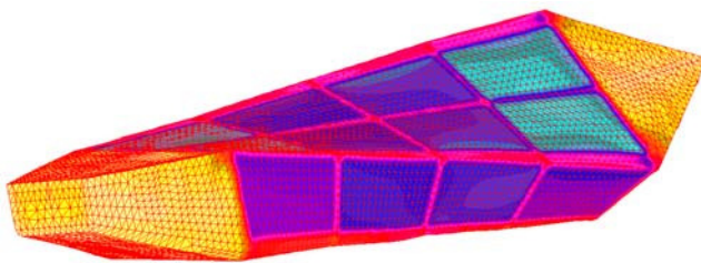
Figure 7. First torsional modal shape (COSMOS)
