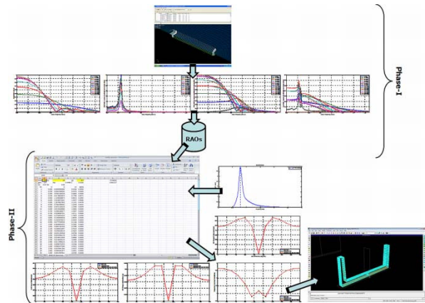
Figure 13. Schematic diagram of WILC
