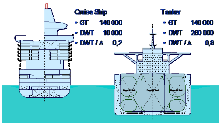
Figure 3. Deadweight and capacity carriers
