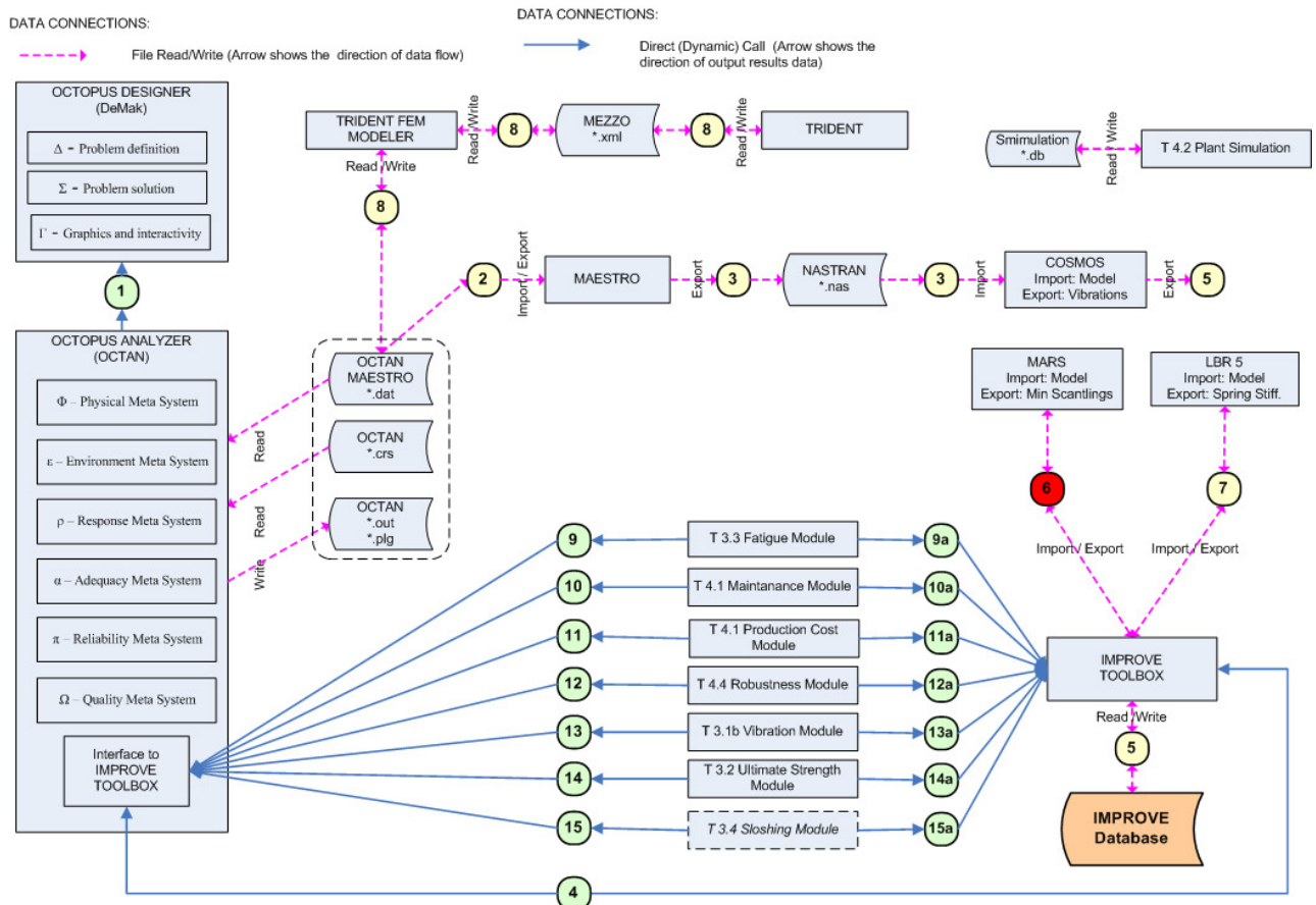
Figure 18. Scheme of the dataflow used for OCTOPUS and MAESTRO tools within the scope of the IMPROVE framework.
