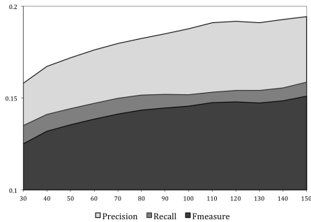
Figure 7: OntoMap Performance on Documents with Different Lengths
