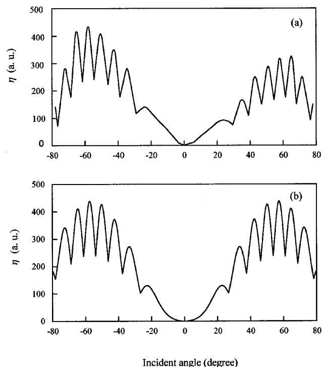
FIG. 1. Experimental Maker fringe pattern (a) and the doubly fitted one (b) for a poled silica sample in which both the near-surface and bulk nonlinearities are significant. The fitting gives the ratio d_{33v}/d_{33s}=0.38 .
