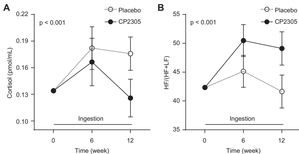
Fig. 5. Time-dependent changes in the salivary cortisol concentration (A) and the ratio of parasympathetic nerve activity (HF/HF + LF) (B). Open and closed circles represent individuals in the placebo ( \circ ) and paraprobiotic CP2305-fed ( \bullet ) groups, respectively. Dotted and solid lines indicate the placebo and paraprobiotic CP2305-fed groups, respectively. Repeated-measures ANCOVA was applied to the time-dependent changes of both items in the whole model. ANCOVA was applied to each time point as a post hoc test.
