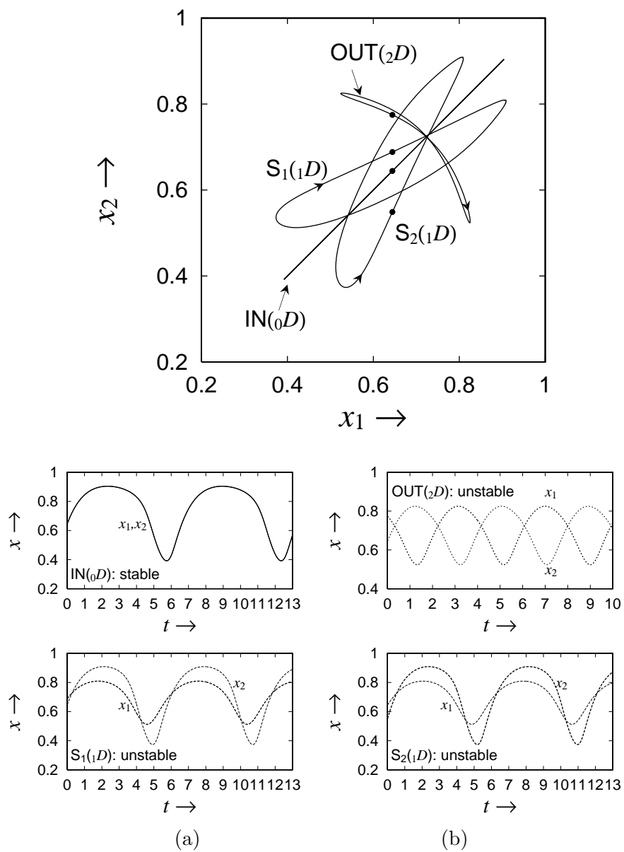
Figure 3: Co-existence of solutions. c = 12.0 , \delta = 2.747 . Black circles are fixed points of the Poincaré map.
