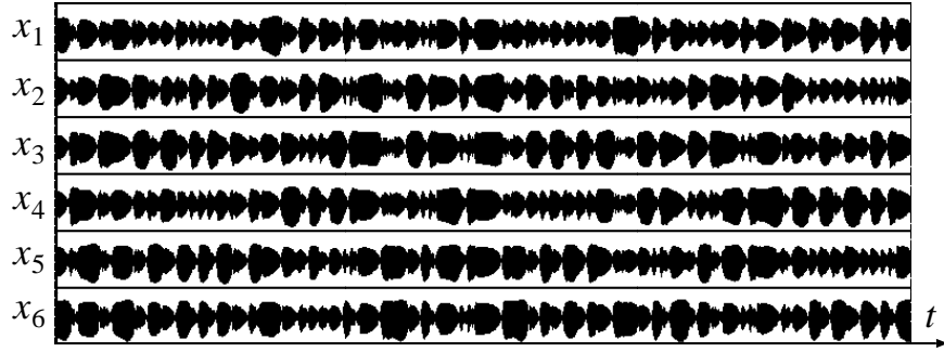
Figure 10: A snapshot of the wave form x_i in six coupled-neurons. c = 10 , \delta = 1.09 , 1000 < t < 6000 . The average value of return time for a cycle is about 6.14 sec.
