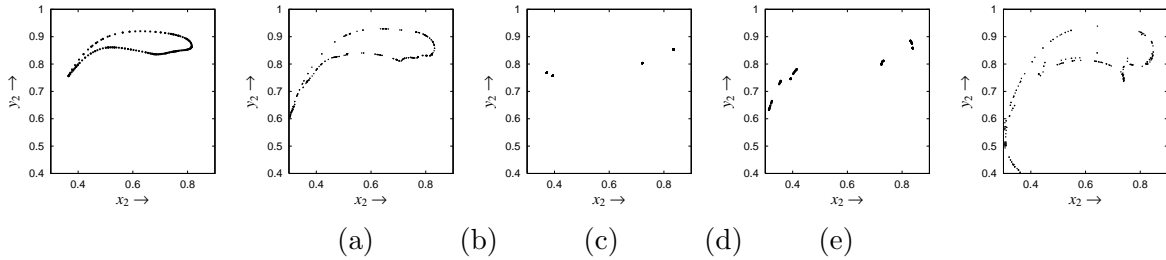
Figure 8: Phase portraits according to parameter values indicated in Fig. 7. (a) torus, \delta = 2.7 . (b) chaotic, \delta = 2.738 . (c) 4-periodic locking, \delta = 2.742 . (d) chaos via cascade period-doubling for a period-4 solution, \delta = 2.763 . (e) chaos, \delta = 2.79 .
