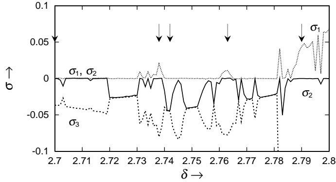
Figure 7: Lyapunov exponents near torus breakdown. c = 13 .
