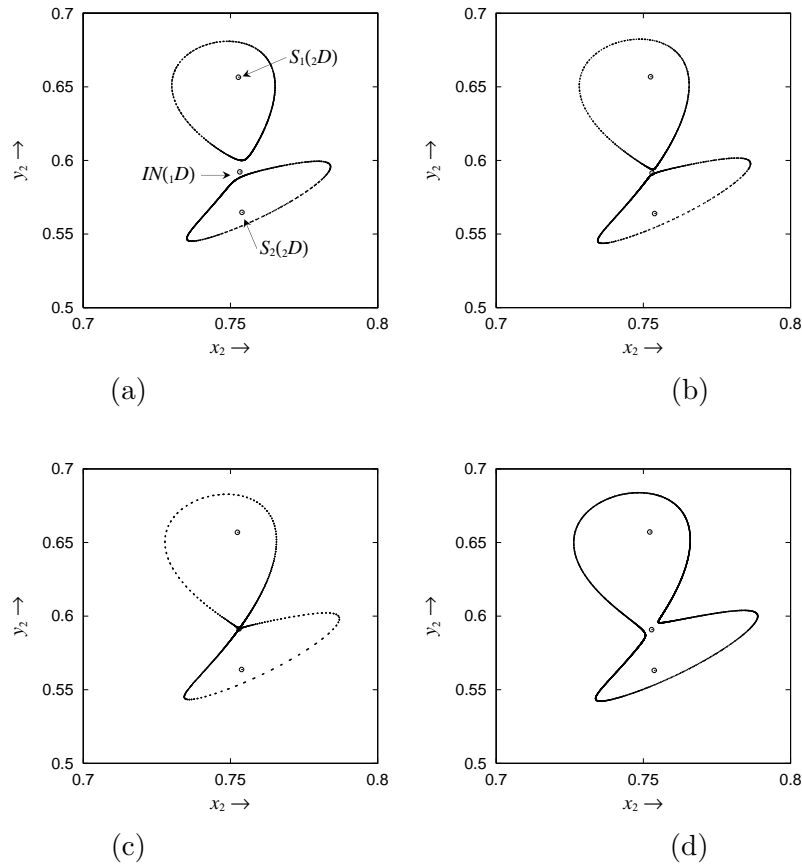
Figure 11: Coalesce of tori. All points are projections of the Poincaré map on the x_2 - y_2 plane. (a): \delta = 1.529 . (b): \delta = 1.528 , (c): \delta = 1.52774 , (d): \delta = 1.527 , a = b = 10 , c = 9 , d = -2 , \rho_x = 0 , \rho_y = -6 .
