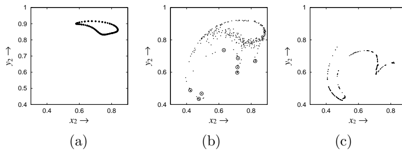
Figure 6: The Poincaré map in the x_2 - y_2 plane. c = 11 . (a) A torus. \delta = 2.32 (b) \delta = 2.339 . The torus is broken, and the orbit behaves chaotically for a while; finally, it is trapped into eight-periodic points (marked by circles). (c) A chaotic attractor. \delta = 2.34 .
