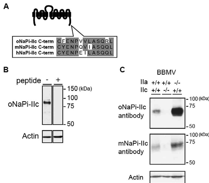
Fig. 1 Production and characterization of anti-oNaPi-IIc antibody A Alignment of the C-terminus 13-amino acid sequence of NaPi-IIc (opossum, mouse, human). B Peptide competition assay. Total cell lysates from OK cells at day 2 after seeding were separated by SDS-PAGE, and the blotted membrane was probed with anti-oNaPi-IIc antibody, which was preincubated for 1 h at room temperature with (+) or without (-) recombinant fragments corresponding to the 13- amino acid of the oNaPi-IIc C-terminus, as indicated. C Western blotting analysis using renal BBMVs isolated from the kidney of WT, NaPi-IIc-KO (NaPi-IIc -/-), and NaPi-IIa-KO (NaPi-IIa -/-) mice by opossum and mouse NaPi-IIc antibodies. Actin was used as an internal control.
