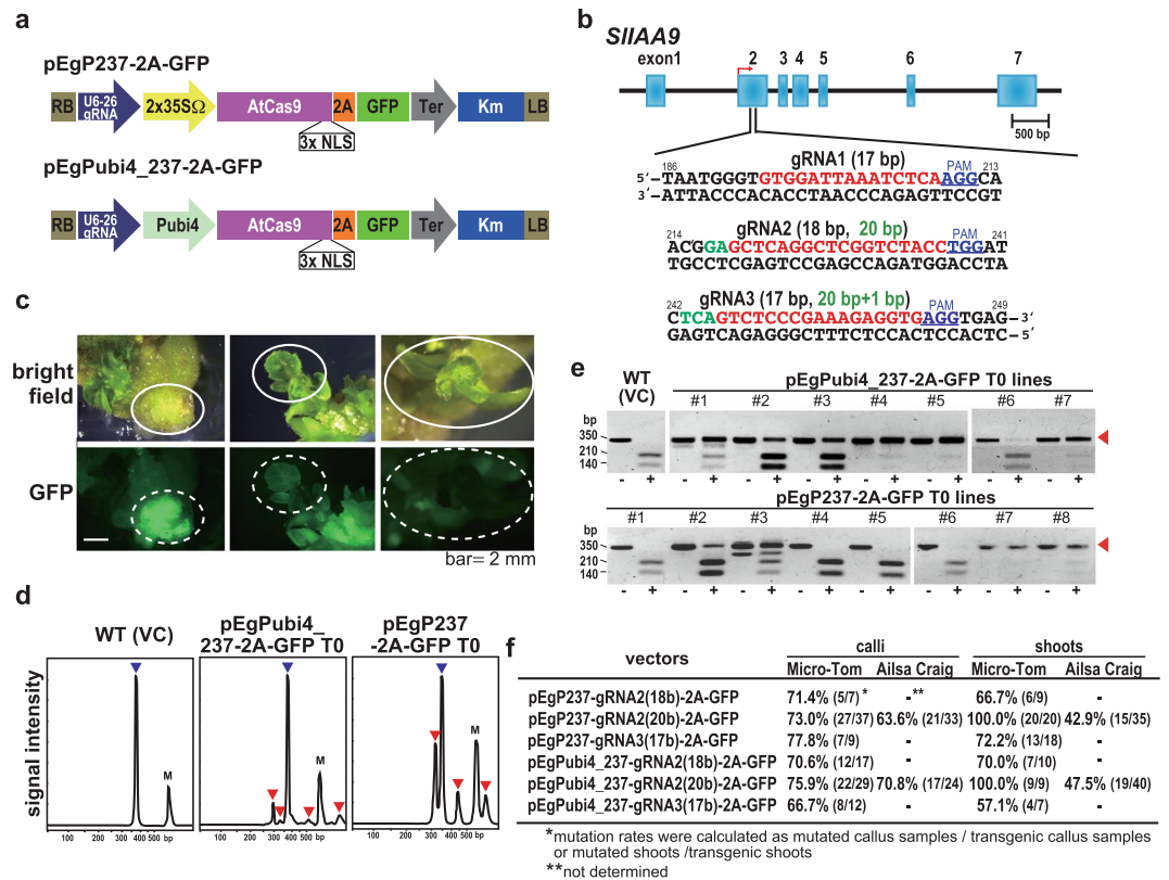
Figure 1. Site-directed mutagenesis in SlIAA9 using CRISPR/Cas9. (a) Schematic representation of T-DNA regions of the CRISPR/Cas9 binary vectors used in this study. U6-26 gRNA: Arabidopsis U6 snRNA-26 promoter and the gRNA sequence, 2 \times 35S\Omega : 2 \times CaMV35S promoter with the omega enhancer sequence, Pubi4: parsley ubiquitin 4-2 promoter, AtCas9: Arabidopsis-codon optimized SpCas9, 2A: 2A self-cleavage peptide, Km: the kanamycin resistant marker expression cassette, RB: right border of T-DNA, LB: left border of T-DNA. (b) Target sites for SlIAA9 . 17 b/18 b-length target sequences are in red. The 2–3 base extensions of the 5' end for the 20 b-length target sequences are in green. The PAM is in blue. A bent arrow indicates the translational start site. (c) Visual GFP-selection of transgenic calli with introduced gRNA and Cas9-2A-GFP. Tissues indicated by white circles (white dotted-circles in lower panels “GFP”) were used for mutation analysis or plantlet-regeneration. (d) Heteroduplex mobility assay with the MultiNA electrophoresis system. Multiple heteroduplex peaks (red arrows) were detected in PCR amplicons from the CRISPR/Cas9 transgenic tomato calli, whereas a single peak was detected from the wild-type control (blue arrow). VC: vector control. M; internal marker. (e) PCR-RFLP analysis of the genome editing in Micro-Tom calli (RNA2-20b). +; Acc I digested PCR products, –; non-digested PCR products. Numbers show the regenerated T0 plant lines. (f) Determination of mutation ratios in transgenic calli and shoots. The mutation ratios were calculated by dividing number of mutant calli or shoots by the total number of transformed calli or shoots.
