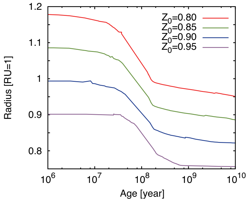
Figure 2.19: The time evolution of the planetary radius divided by the present radius of Uranus RU = 4.01 R_{\oplus} . Line colors represent the initial mass fraction H_2O in the atmosphere and envelope. The initial fraction of NH_3/H_2O = 0.05675 and CH_4/H_2O = 0.135 . We assume (Z_0, Z_{tot}) = (0.80, 0.81) , (0.85, 0.86) , (0.90, 0.91) , and (0.95, 0.96) , respectively. We assume Z_w = 0.97 and Z_0 in the envelope is constant through the evolution. The equilibrium temperature is 58.2 K.
