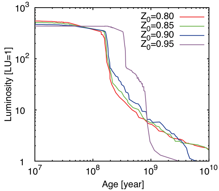
Figure 2.18: The time evolution of the planetary luminosity divided by the present luminosity of Uranus LU = 5.6 \times 10^{22} \text{ erg s}^{-1} . Line colors represent the initial mass fraction \text{H}_2\text{O} in the atmosphere and envelope. The initial fraction of \text{NH}_3/\text{H}_2\text{O} = 0.05675 and \text{CH}_4/\text{H}_2\text{O} = 0.135 . We assume (Z_0, Z_{\text{tot}}) = (0.80, 0.81) , (0.85, 0.86) , (0.90, 0.91) , and (0.95, 0.96) , respectively. We assume Z_w = 0.97 and Z_0 in the envelope is constant through the evolution. The equilibrium temperature is 58.2 K.
