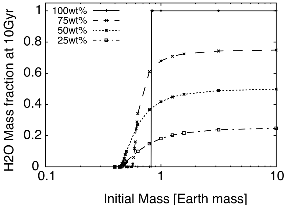
Figure 3.5: Relationship between the initial planetary mass and the fraction of the water envelope at 10 gigayears for four initial water mass fractions of X_{\text{wt},0} = 100\% (solid), 75\% (dashed), 50\% (dotted), and 25\% (dot-dashed). We have assumed L_0 = 1 \times 10^{24} \text{ erg s}^{-1} , a = 0.1 \text{ AU} and \varepsilon = 0.1 .
