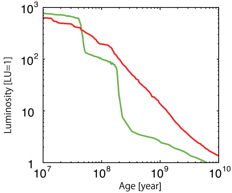
Figure 2.6: The time evolution of the planetary luminosity divided by the present luminosity of Uranus LU = 5.6 \times 10^{22} \text{ erg s}^{-1} . We set 70 mol % of \text{H}_2\text{O} , 9.45 mol % of \text{NH}_3 , and 3.97 mol % of \text{CH}_4 , respectively. The red line is the relationship without the effect of the condensation of \text{H}_2\text{O} , \text{NH}_3 , and \text{CH}_4 . The green line is the relationship with the effect of condensation of \text{H}_2\text{O} , \text{NH}_3 , and \text{CH}_4 . We assume Z_{\text{tot}} = 0.8 , Z_0 = 0.3 , and Z_w = 0.5 . The equilibrium temperature is 58.2 K
