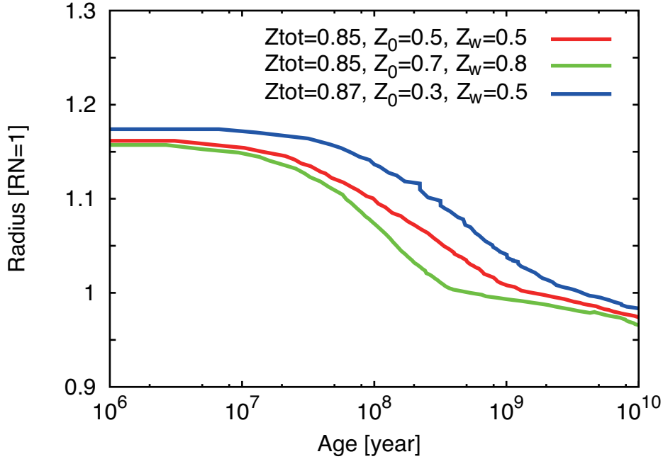
Figure 2.20: The time evolution of the planetary radius divided by the present radius of Neptune RN = 3.89 R_{\oplus} . The initial fraction of \text{NH}_3/\text{H}_2\text{O} = 0.458 and \text{CH}_4/\text{H}_2\text{O} = 0.135 . Lines' colors represent the parameters of Z_0, Z_{\text{tot}} and Z_w . The red, green, and blue represent (Z_0, Z_{\text{tot}}, Z_w) = (0.5, 0.85, 0.5) , (0.7, 0.85, 0.8) , and (0.3, 0.87, 0.5) , respectively. We assume Z_0 in the envelope is constant through the evolution. The equilibrium temperature is 46.6 K.
