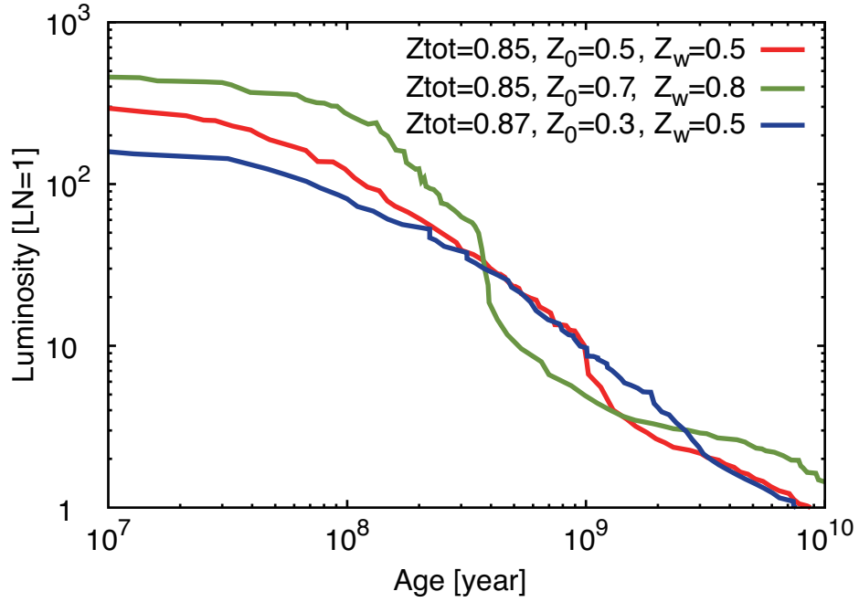
Figure 2.21: The time evolution of the planetary luminosity divided by the present luminosity of Neptune LN = 5.3 \times 10^{22} \text{erg s}^{-1} . The initial fraction of \text{NH}_3/\text{H}_2\text{O} = 0.458 and \text{CH}_4/\text{H}_2\text{O} = 0.135 . Lines' colors represent the parameters of Z_0, Z_{tot} . The red, green, and blue represent (Z_0, Z_{tot}, Z_w) = (0.5, 0.85, 0.5), (0.7, 0.85, 0.8), and (0.3, 0.87, 0.5) , respectively. We assume Z_0 in the envelope is constant through the evolution. The equilibrium temperature is 46.6 K.
