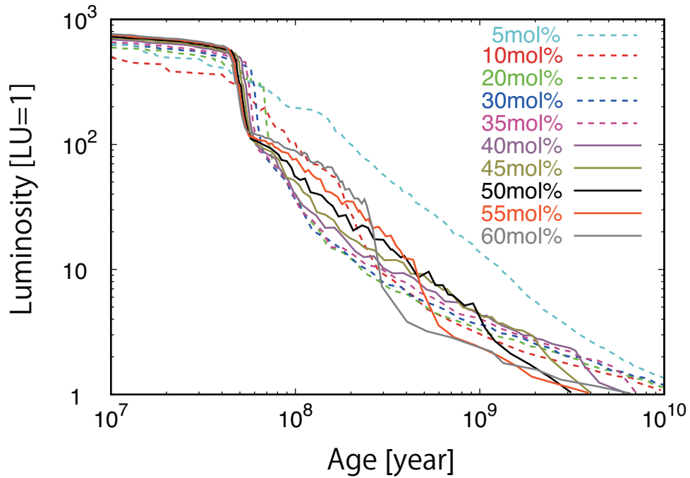
Figure 2.8: The time evolution of the planetary luminosity divided by the present luminosity of Uranus LU = 5.6 \times 10^{22} \text{ erg s}^{-1} . Line colors represent the initial mole fraction of H_2O . We set 5-60 mol % of H_2O . The initial fraction of NH_3/H_2O = 0.135 and CH_4/H_2O = 0.05675 . We assume Z_{\text{tot}} = 0.8 , Z_0 = 0.3 , and Z_w = 0.5 . The equilibrium temperature is 58.2 K.
