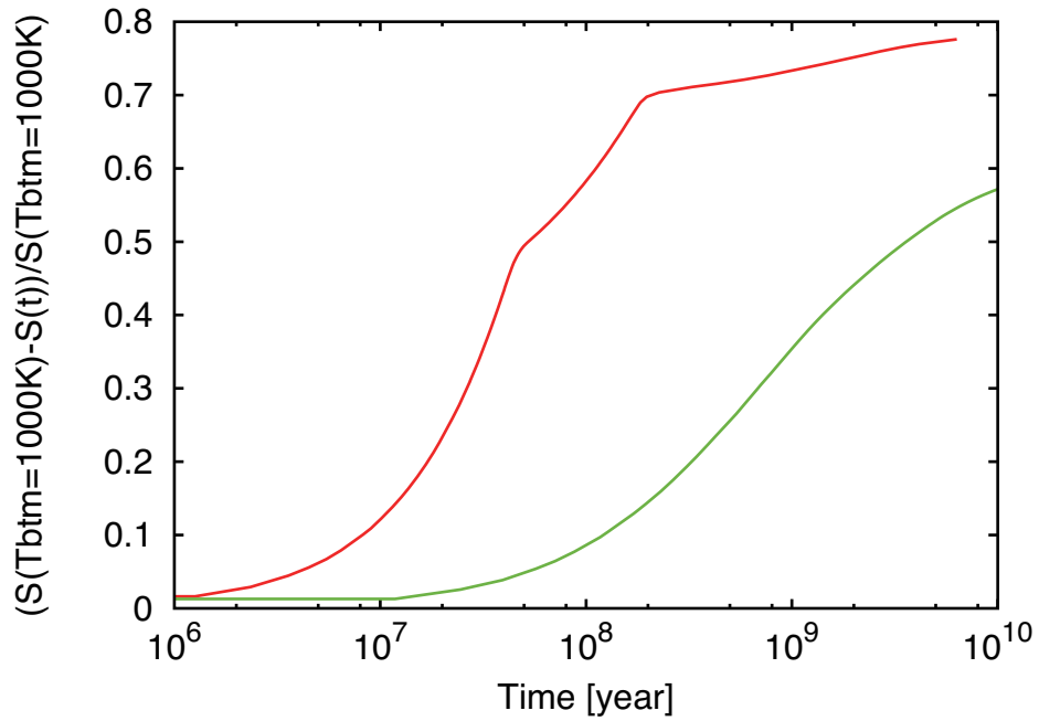
Figure 2.7: The time evolution of the planetary entropy. t = 0 represents the temperature at 100 bar 1000 K. We set 70 mol % of \text{H}_2\text{O} , 9.45 mol % of \text{NH}_3 , and 3.97 mol % of \text{CH}_4 , respectively. The red line is the relationship the effect of the condensation of \text{H}_2\text{O} , \text{NH}_3 , and \text{CH}_4 . The green line is the relationship without the effect of condensation of \text{H}_2\text{O} , \text{NH}_3 , and \text{CH}_4 . We assume Z_{\text{tot}} = 0.8 , Z_0 = 0.3 , and Z_w = 0.5 . The equilibrium temperature is 58.2 K.
