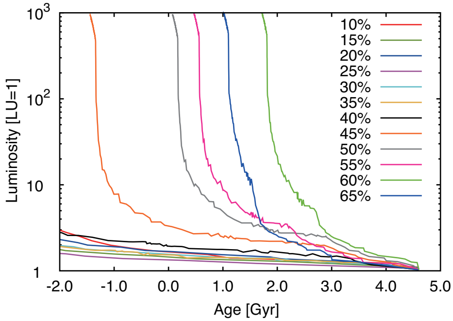
Figure 2.9: The time evolution of the planetary luminosity divided by the present luminosity of Uranus LU = 5.6 \times 10^{22} \text{ erg s}^{-1} . Line colors represent the initial mole fraction of \text{H}_2\text{O} . We set 10-65 mol % of \text{H}_2\text{O} . The initial fraction of \text{NH}_3/\text{H}_2\text{O} = 0.135 and \text{CH}_4/\text{H}_2\text{O} = 0.05675 . We assume Z_{\text{tot}} = 0.8 , Z_0 = 0.3 , and Z_w = 0.5 . The equilibrium temperature is 58.2 K. The evolutions is calculated backward from the age is 4.6 \times 10^9 years.
