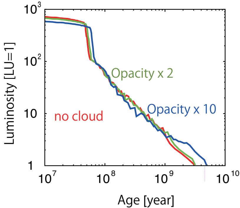
Figure 2.14: The time evolution of the planetary luminosity divided by the present luminosity of Uranus LU = 5.6 \times 10^{22} \text{ erg s}^{-1} . Line colors represent the difference of the effect of cloud. The red, green, blue, and purple lines are no cloud, \kappa_{\text{th}} \times 2 , and \kappa_{\text{th}} \times 10 , respectively, where \kappa_{\text{th}} is the infrared opacity of the atmosphere. We set 70 mol % of \text{H}_2\text{O} , 9.45 mol % of \text{NH}_3 , and 3.97 mol % of \text{CH}_4 , respectively. We assume Z_{\text{tot}} = 0.8 , Z_0 = 0.3 , and Z_w = 0.5 . The equilibrium temperature is 58.2 K.
