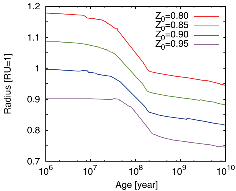
Figure 2.17: The time evolution of the planetary radius divided by the present radius of Uranus RU = 4.01 R_{\oplus} . Line colors represent the initial mass fraction H_2O in the atmosphere and envelope. The initial fraction of NH_3/H_2O = 0.458 and CH_4/H_2O = 0.135 . We assume (Z_0, Z_{tot}) = (0.80, 0.81) , (0.85, 0.86) , (0.90, 0.91) , and (0.95, 0.96) , respectively. We assume Z_w = 0.97 and Z_0 in the envelope is constant through the evolution. The equilibrium temperature is 58.2 K.
