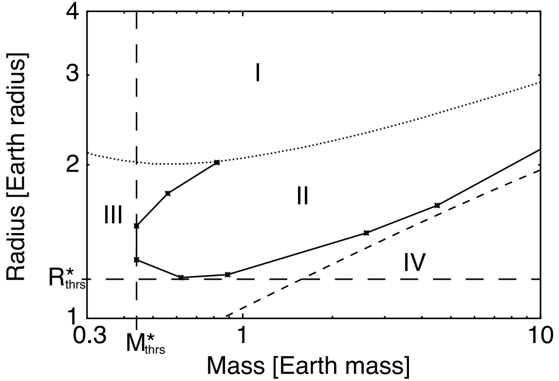
Figure 3.8: Relationship between the threshold mass and the threshold radius. The latter is defined by the radius that the planet with M_{\text{thrs}} would have at 10 giga years without ever experiencing mass loss (denoted by R_{\text{thrs}} ). The squares, which are connected with a solid line, are M_{\text{thrs}} and R_{\text{thrs}} for 0.1 AU and seven different initial water mass fractions X_{\text{wt},0} = 100\% , 75\% , 50\% , 25\% , 10\% , 5\% , 1\% and 0.5\% . The dashed and dotted lines represent mass-radius relationships, respectively, for rocky planets and pure-water planets at 0.1 AU. M_{\text{thrs}}^* and R_{\text{thrs}}^* represent the minimum values of M_{\text{thrs}} and R_{\text{thrs}} , respectively.
