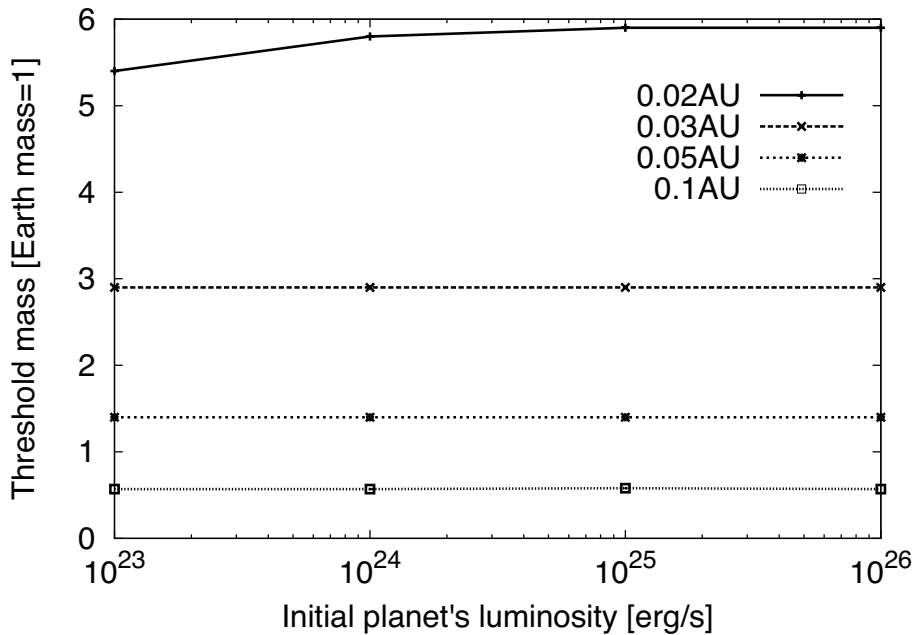
Figure 3.4: The threshold mass in M_{\oplus} as a function of the initial planet's luminosity in \text{erg s}^{-1} for four choices of semimajor axes. The solid, dashed, dotted and dot-dashed represent a = 0.02, 0.03, 0.05 and 0.1 AU, respectively. We have assumed X_{\text{wt}} = 75\% and \varepsilon = 0.1 .
