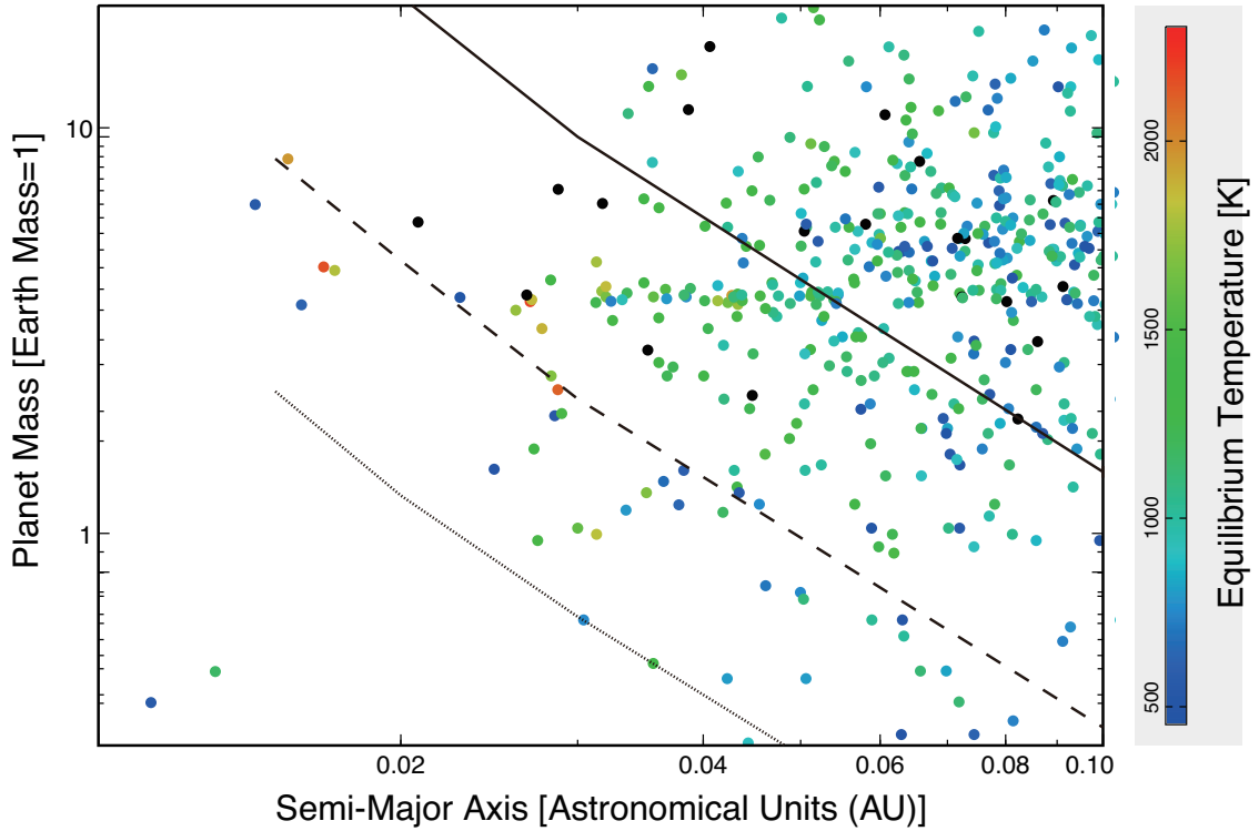
Figure 3.11: Distribution of masses and semimajor axes (or incident fluxes) of detected exoplanets compared with the minimum threshold mass, M_{\text{thrs}}^* , derived in this study (see § 3.3 for definition). We have shown three M_{\text{thrs}}^* - a relationships for different heating efficiencies: \varepsilon = 1 (solid line), \varepsilon = 0.1 (dashed line) and \varepsilon = 0.01 (dotted line). Filled circles with error bars represent observational data (from http://exoplanet.org (Wright et al. 2011), as of February 12, 2016) for planets orbiting host stars with effective temperature of 5000-6000 K (relatively early K-type stars and G-type stars). Planets are colored according to their zero-albedo equilibrium temperatures in K. In the planet names, "CoR" and "Kep" stand for CoRoT and Kepler, respectively.
