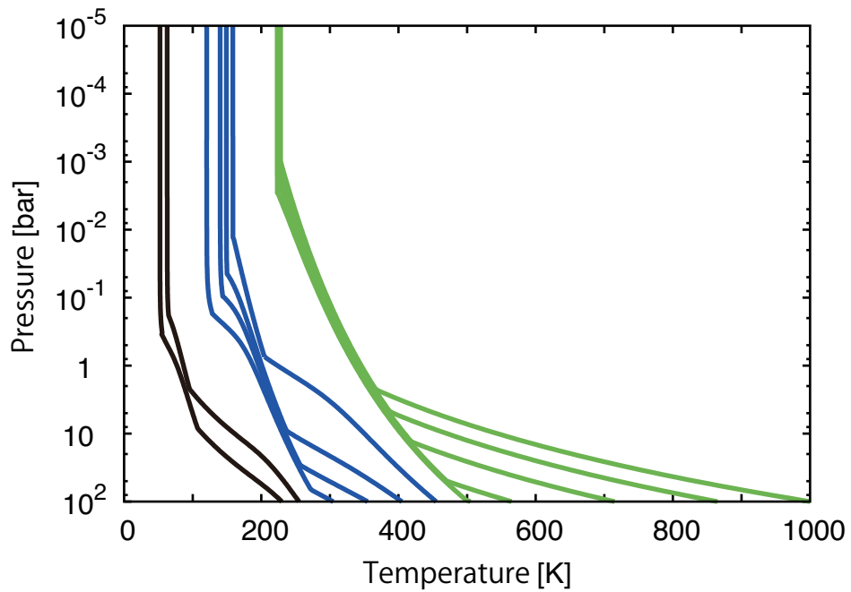
Figure 2.4: The temperature-pressure relation of atmosphere. We set 70 mol % of \text{H}_2\text{O} , 9.45 mol % of \text{NH}_3 , and 3.97 mol % of \text{CH}_4 , respectively. Line colors represent main compositions in the atmosphere. Green, blue, and black lines are \text{H}_2\text{O} , \text{NH}_3 , and \text{CH}_4 , respectively. We assume Z_{\text{tot}} = 0.8 , Z_0 = 0.3 , and Z_w = 0.5 . The equilibrium temperature is 58.2 K.
