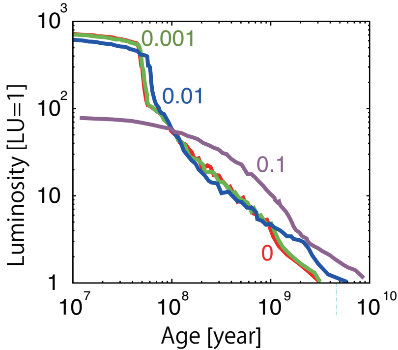
Figure 2.13: The time evolution of the planetary luminosity divided by the present luminosity of Uranus LU = 5.6 \times 10^{22} \text{ erg s}^{-1} . The red, green, blue, and purple lines are \delta\nabla = 0, 0.001, 0.01, and 0.1 , respectively (see Eq. (2.58) for the definition of \delta\nabla ). We set 70 mol % of \text{H}_2\text{O} , 9.45 mol % of \text{NH}_3 , and 3.97 mol % of \text{CH}_4 , respectively. We assume Z_{\text{tot}} = 0.8 , Z_0 = 0.3 , and Z_w = 0.5 . The equilibrium temperature is 58.2 K.
