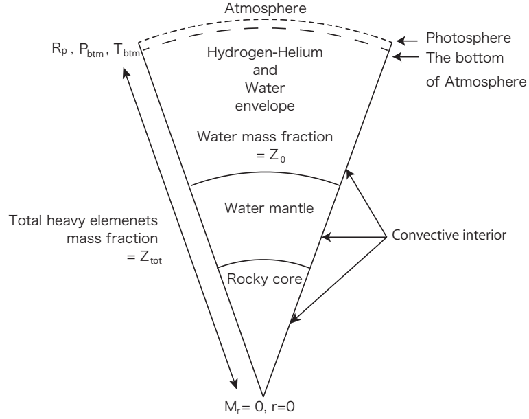
Figure 2.2: Model of the planetary structure in this study.
