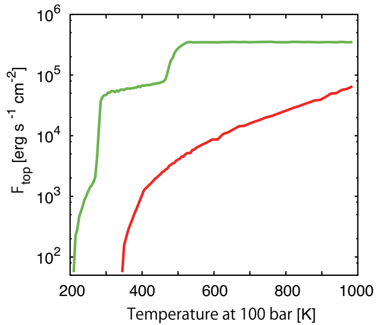
Figure 2.5: The relationship between the F_{\text{top}} and the temperature at 100 bar in the atmosphere. We set 70 mol % of \text{H}_2\text{O} , 9.45 mol % of \text{NH}_3 , and 3.97 mol % of \text{CH}_4 , respectively. The red line is the relationship without the effect of the condensation of \text{H}_2\text{O} , \text{NH}_3 , and \text{CH}_4 . The green line is the relationship with the effect of condensation of \text{H}_2\text{O} , \text{NH}_3 , and \text{CH}_4 . We assume Z_{\text{tot}} = 0.8 , Z_0 = 0.3 , and Z_w = 0.5 . The equilibrium temperature is 58.2 K.
