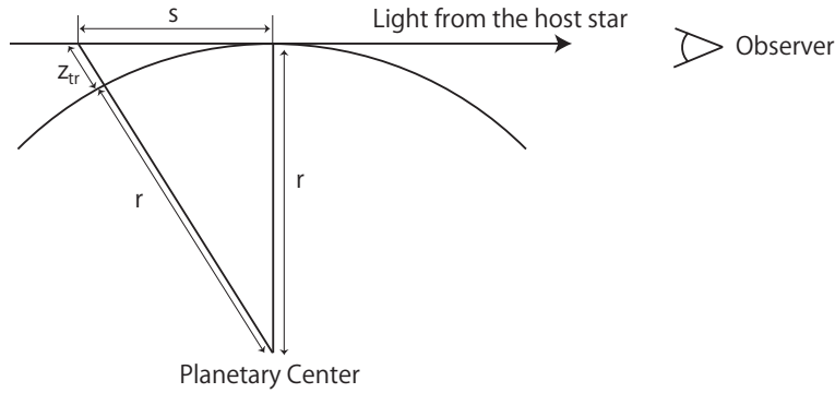
Figure 3.2: The figure of the chord optical depth.
