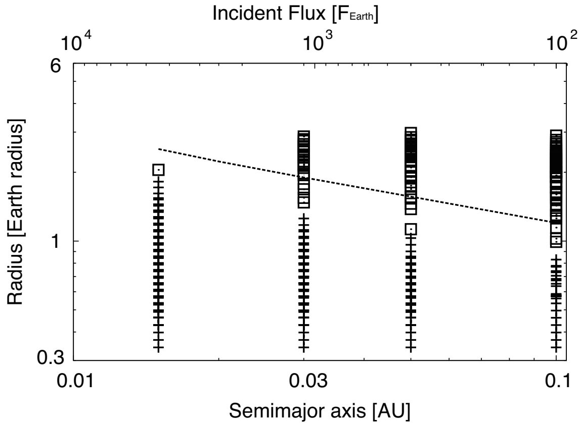
Figure 3.12: Theoretical distribution of radii and semi-major axes or incident fluxes of planets at 10 giga years with various initial masses and water mass fractions. Cross points represent planets that lost their water envelopes completely due to the photo-evaporation in 10 giga years, while open squares represent planets that survive significant loss of the water envelopes. The green line is the minimum threshold radii, R_{\text{thrs}}^* . Here we have adopted \varepsilon = 0.1 .
