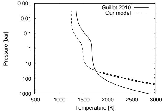
Figure F.1: Temperature-pressure profiles for a solar-composition atmosphere (see the details in text). The solid and dotted lines represent the \gamma = 0.4 (Guillot, 2010) and our models, respectively. The thin and thick parts of the lines represent the radiative and convective regions, respectively. We assumed g = 980 \text{ cm s}^{-2} , T_{\text{int}} = 300 \text{ K} and T_{\text{irr}} = 1500 \text{ K} .
