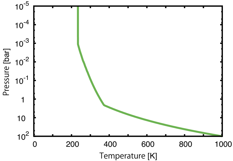
Figure 2.3: The temperature-pressure relation of atmosphere. We set 70 mol % of \text{H}_2\text{O} , 9.45 mol % of \text{NH}_3 , and 3.97 mol % of \text{CH}_4 , respectively. We assume Z_{\text{tot}} = 0.8 , Z_0 = 0.3 , and Z_w = 0.5 . The bottom of atmosphere is P = 100 bar. Temperature at P = 100 bar is 1000 K. The equilibrium temperature is 58.2 K.
