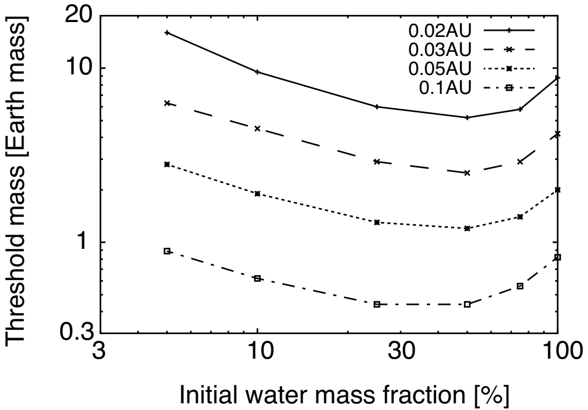
Figure 3.7: Relationship between the initial water mass fraction X_{\text{wt},0} in % and the threshold mass M_{\text{thrs}} in M_{\oplus} for four choices of semi-major axes of 0.02 AU (solid), 0.03 AU (dashed), 0.05 AU (dotted) and 0.1 AU (dot-dashed). We have assumed L_0 = 1 \times 10^{24} erg \text{s}^{-1} and \varepsilon = 0.1 .
