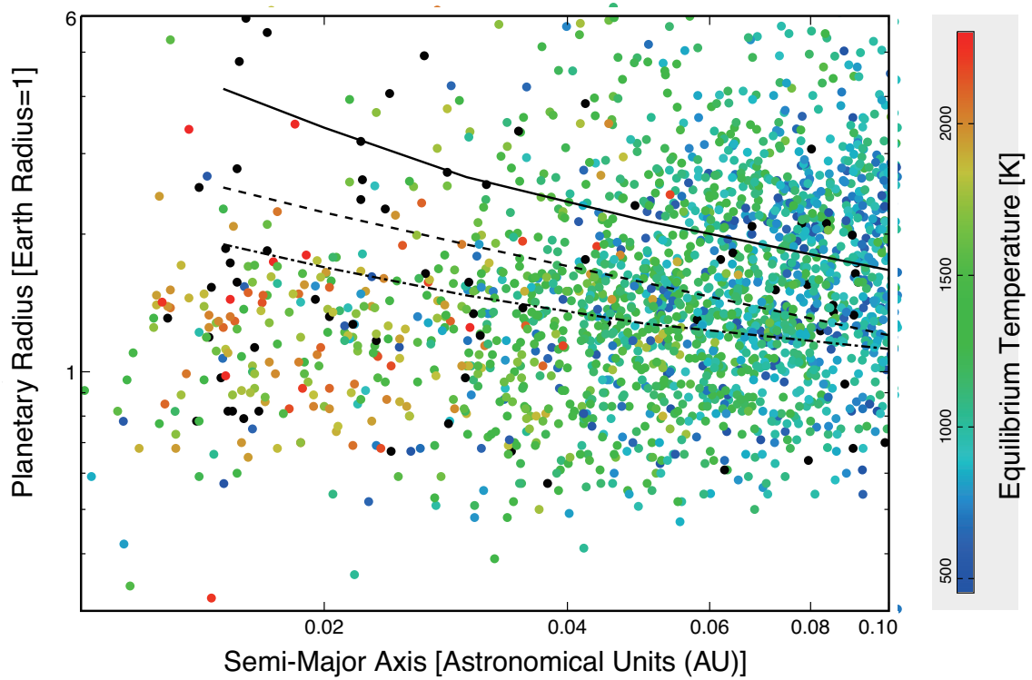
Figure 3.13: Distribution of radii and semi-major axes (or incident fluxes) of Kepler planetary candidates, compared with the threshold radius, R_{\text{thrs}}^* (see § 3.3 for definition). We have shown three R_{\text{thrs}}^* - a relationships for different heating efficiencies: \epsilon = 1 (solid line), \epsilon = 0.1 (dashed line) and \epsilon = 0.01 (dotted line). Filled squares represent observational data (from http://exoplanet.org (Wright et al. 2011), as of February 12, 2016) for planets orbiting host stars with effective temperature of 5300-6000 K (G-type stars).
