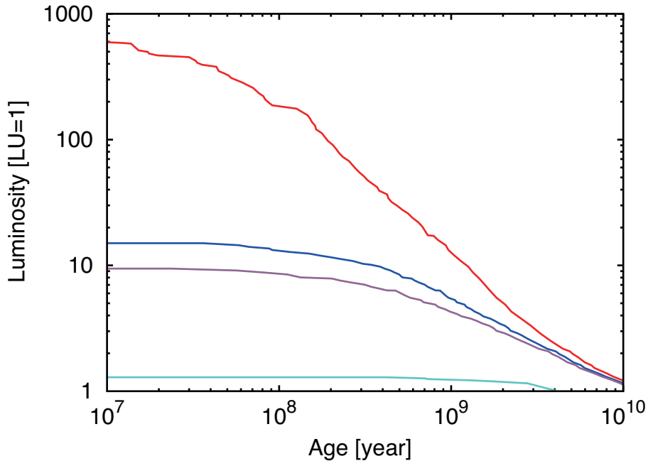
Figure 2.1: The time evolution of planetary luminosity with various initial luminosity. The luminosity and age are normalized by the present luminosity of Uranus LU = 5.6 \times 10^{22} \text{ erg s}^{-1} and year, respectively. Lines' colors represent the initial luminosity. The red, blue, purple, and aqua blue represent \tau_{\text{acc}} = 200 \text{ Myr} , 4.6 Gyr, 13 Gyr, 500 Gyr, respectively. We assume Z_0 = 0.3 , Z_{\text{tot}} = 0.8 , and Z_w = 0.5 , respectively. The condensation of ice compositions (water, ammonia, and methane) are ignored. See § 2.2 for the detail model description.
