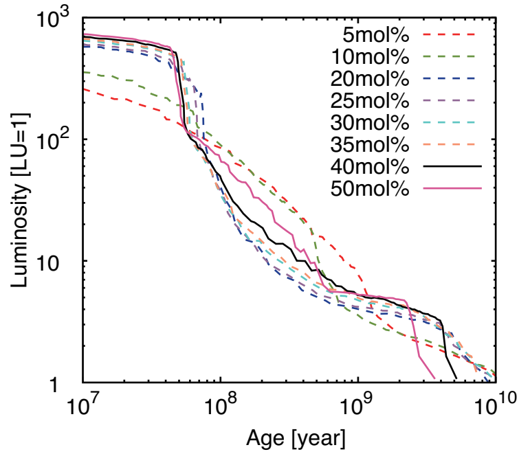
Figure 2.10: The time evolution of the planetary luminosity divided by the present luminosity of Uranus LU = 5.6 \times 10^{22} \text{ erg s}^{-1} . Line colors represent the initial mole fraction of \text{H}_2\text{O} . We set 5-50 mol % of \text{H}_2\text{O} . The initial fraction of \text{NH}_3/\text{H}_2\text{O} = 0.135 and \text{CH}_4/\text{H}_2\text{O} = 0.05675 . We assume Z_{\text{tot}} = 0.8 , Z_0 = 0.3 , and Z_w = 0.5 . The equilibrium temperature is 58.2 K.
