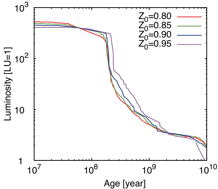
Figure 2.16: The time evolution of the planetary luminosity divided by the present luminosity of Uranus LU = 5.6 \times 10^{22} \text{ erg s}^{-1} . Line colors represent the initial mass fraction \text{H}_2\text{O} in the atmosphere and envelope. The initial fraction of \text{NH}_3/\text{H}_2\text{O} = 0.458 and \text{CH}_4/\text{H}_2\text{O} = 0.135 . We assume (Z_0, Z_{\text{tot}}) = (0.80, 0.81) , (0.85, 0.86) , (0.90, 0.91) , and (0.95, 0.96) , respectively. We assume Z_w = 0.97 and Z_0 in the envelope is constant through the evolution. The equilibrium temperature is 58.2 K
