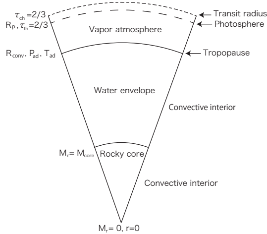
Figure 3.1: Model of the planetary structure in this study.
