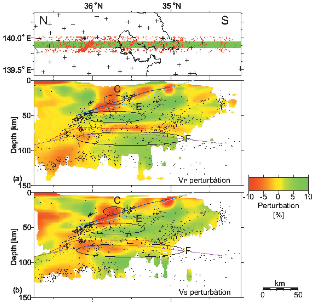
Fig. 4. Vertical cross-sections at 139.9^{\circ}\text{E} (Matsubara et al. 2005). (a) V_p perturbation. (b) V_s perturbation. Red and black dots denote earthquakes between 139.85\text{--}139.95^{\circ}\text{E} . Dashed blue and red lines denote the geometry of the Philippine Sea and Pacific plates, respectively (Matsubara et al. , 2005). Long and short dashed light blue and purple lines denote the configuration of the Philippine Sea and Pacific plates, respectively, as estimated by Ishida [1992]. The area denoted C is interpreted to include up to 30% serpentinized peridotite. Region F, which has high V_p/V_s , represents the oceanic crust of the PAC plate, while the shallower layer (region E) represents heterogeneity in the PHS plate.
