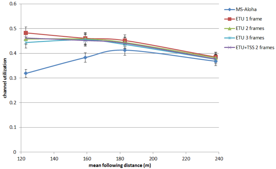
Fig. 31 Channel utilizations of different protocols in Scenario 3
