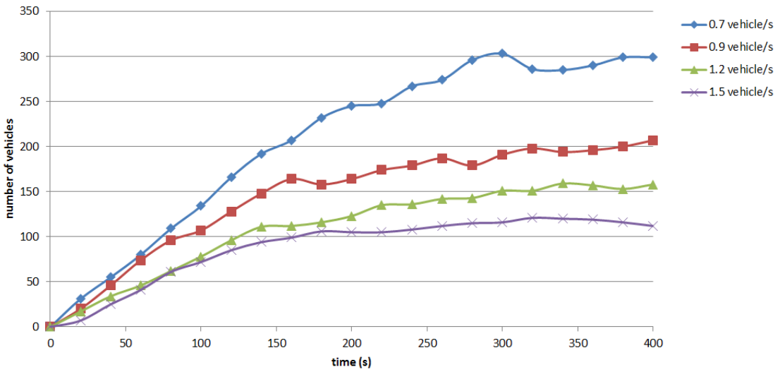
Fig. 15 number of active vehicles in scenario 1
