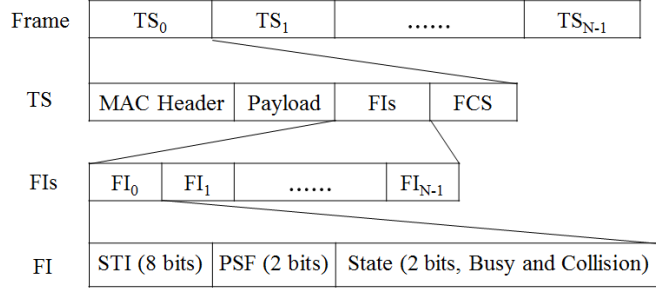
Fig. 7 MS-Aloha frame structure
