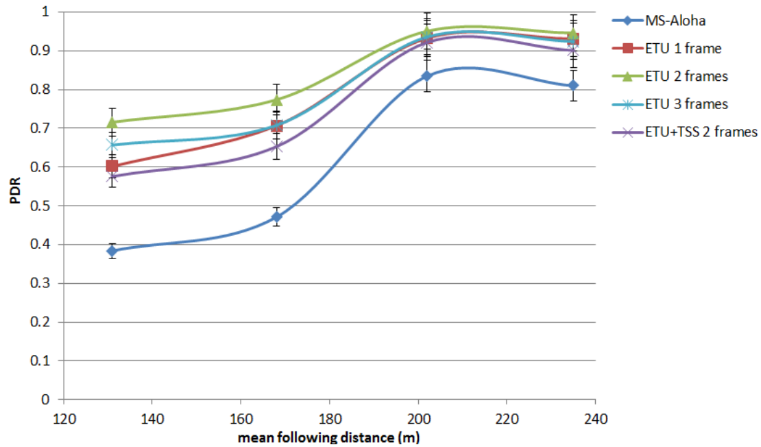
Fig. 25 PDRs of different protocols in Scenario 2
