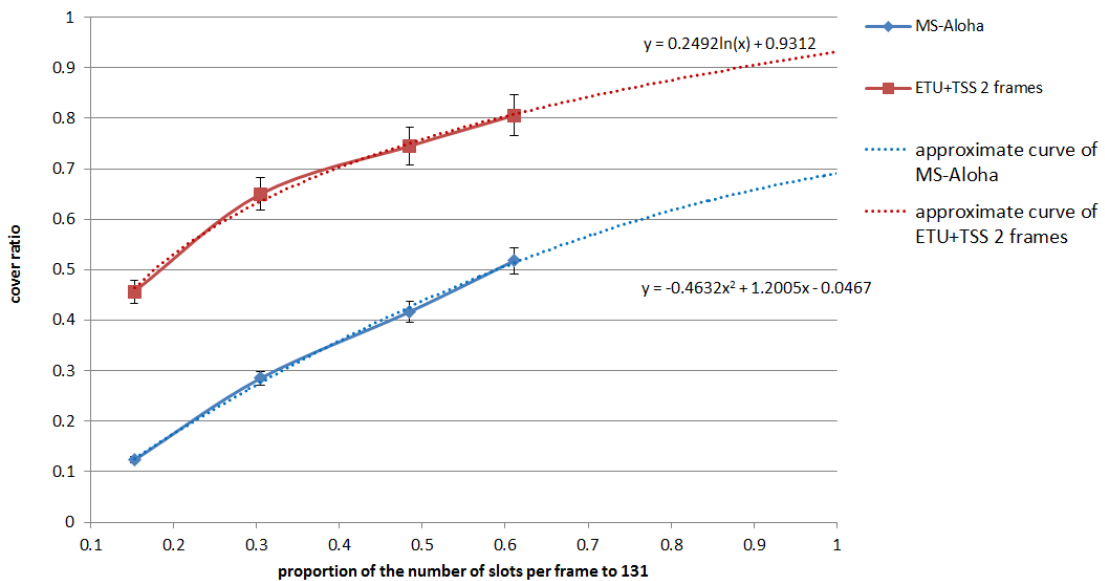
Fig. 33 CRs of MS-Aloha and ETU+TSS 2 frames related to the number of slots per frame
