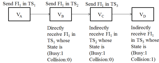
Fig. 8 Role of FI and its propagation mechanism
