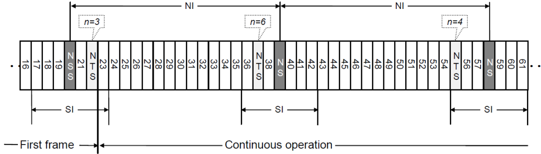
Fig. 6 Continuous operation of STDMA
