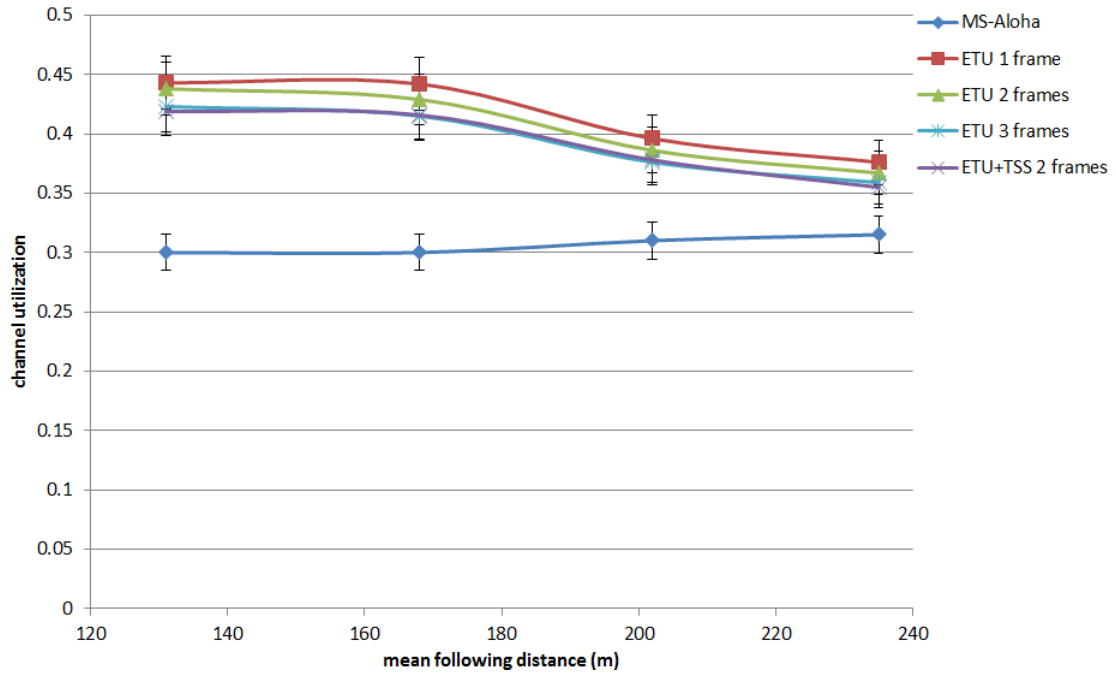
Fig. 27 Channel utilizations of different protocols in Scenario 2
