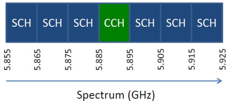
Fig. 1 Spectrum of IEEE 802.11p
