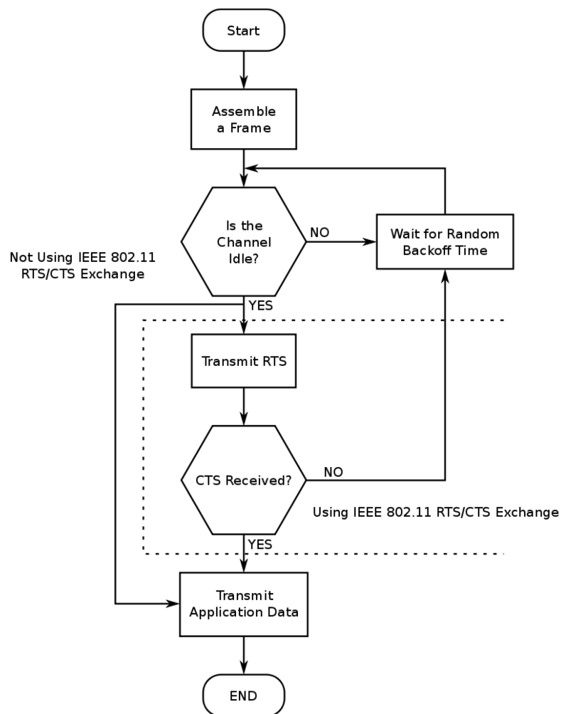
Fig. 2 Mechanism of CSMA/CA ( http://en.wikipedia.org/wiki/Carrier_sense_multiple_access_with_collision_avoidance )
