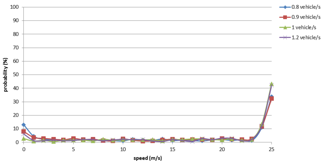
Fig. 18 probability distribution of vehicle speed during 400~500 s in scenario 2
