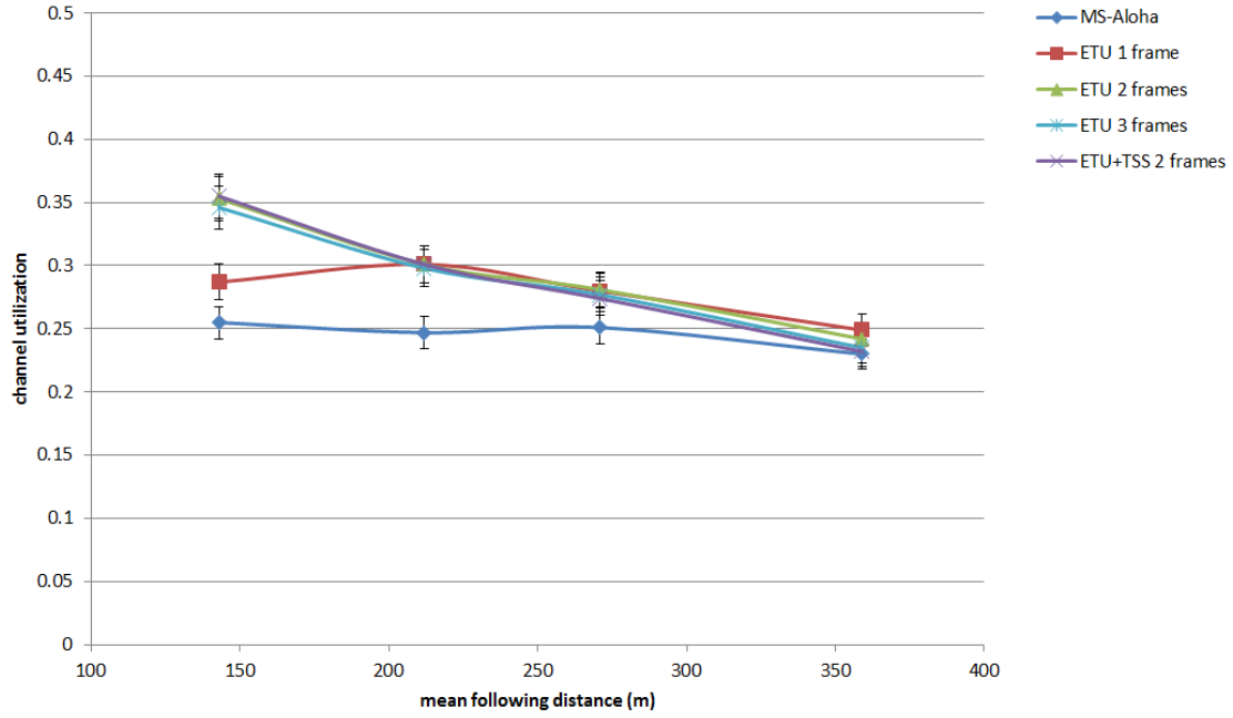
Fig. 23 Channel utilizations of different protocols in Scenario 1
