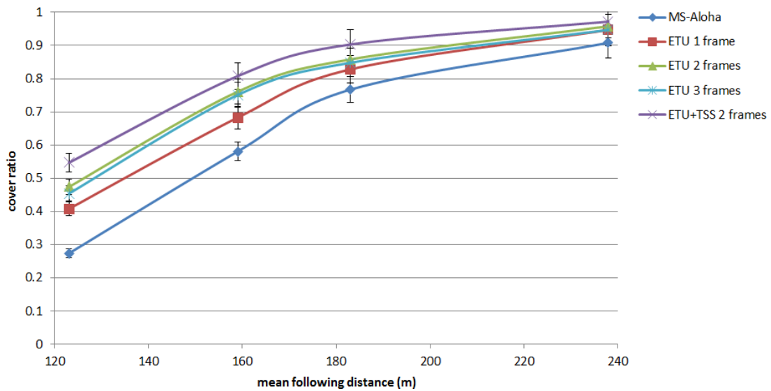
Fig. 32 CRs of different protocols in Scenario 3
