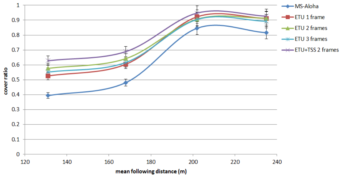
Fig. 28 CRs of different protocols in Scenario 2
