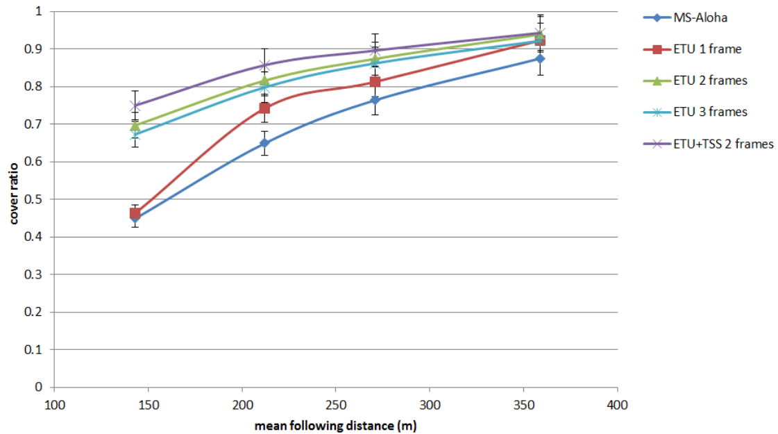
Fig. 24 CRs of different protocols in Scenario 1
