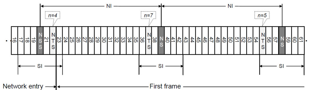
Fig. 5 First frame of STDMA
