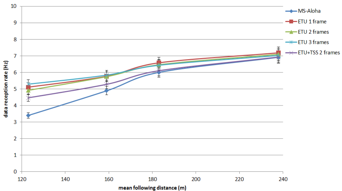
Fig. 30 Data reception rates of different protocols in Scenario 3
