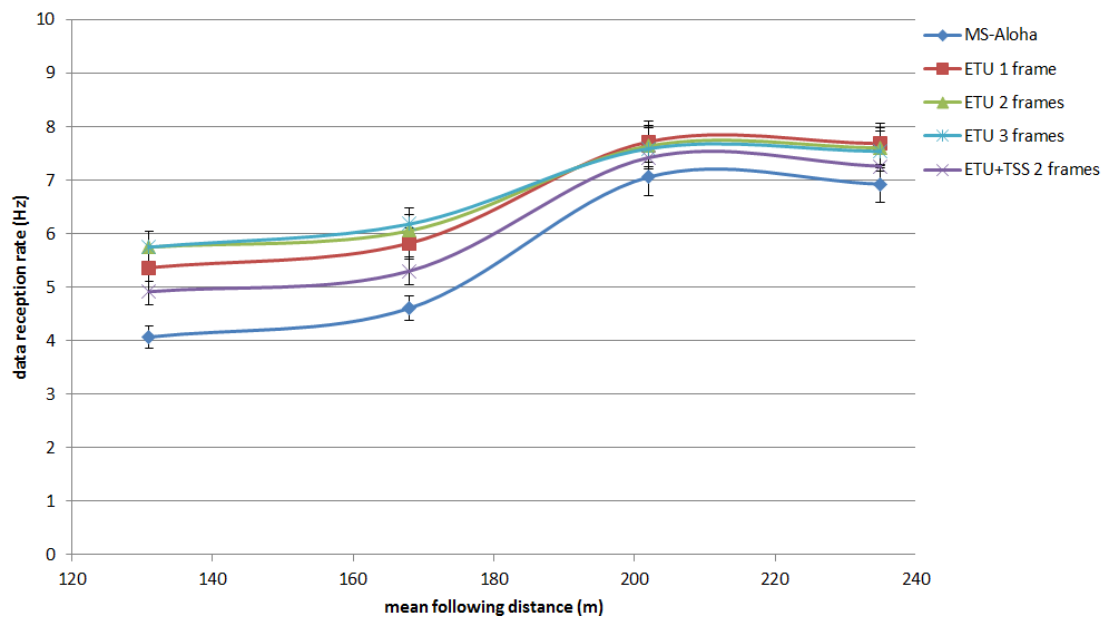
Fig. 26 Data reception rates of different protocols in Scenario 2
