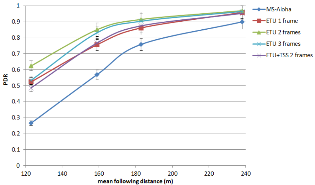
Fig. 29 PDRs of different protocols in Scenario 3
