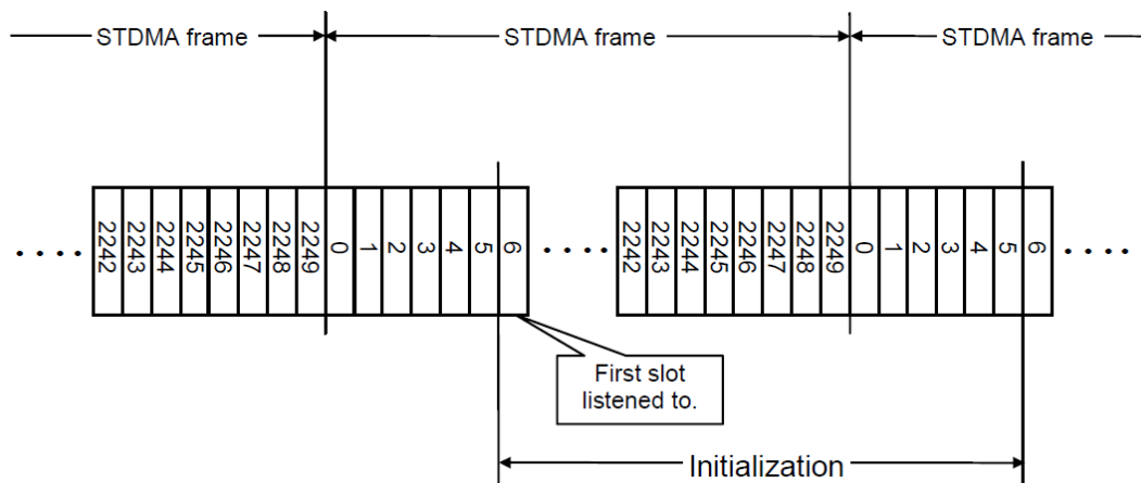
Fig. 3 Initialization of STDMA
