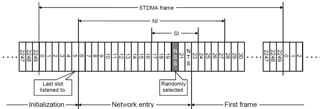
Fig. 4 Network entry of STDMA
