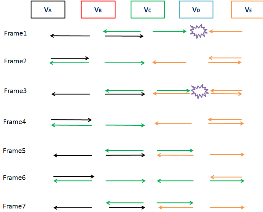
Fig. 14 the mechanism of TSS in five vehicles where STI_A < STI_C < STI_E (colors represent the STIs of different vehicles)
