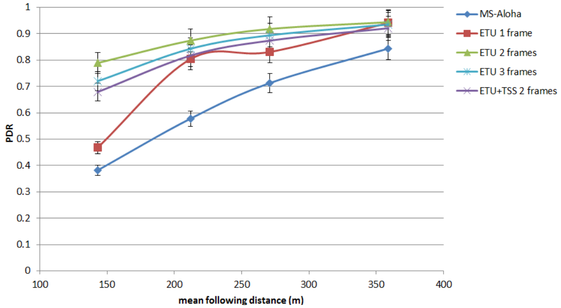
Fig. 21 PDRs of different protocols in Scenario 1
