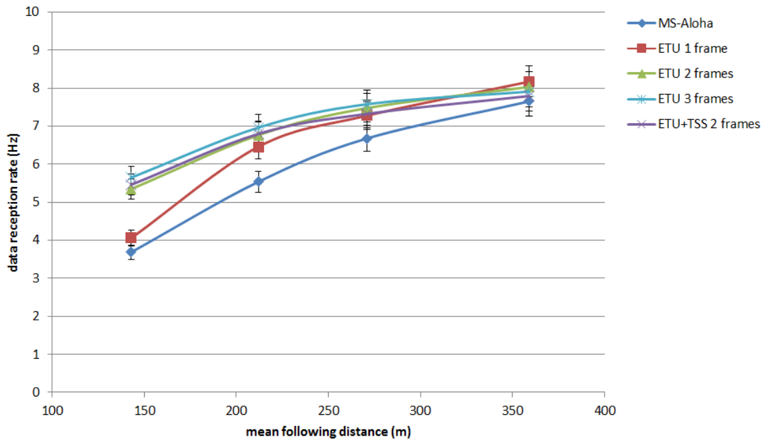
Fig. 22 Data reception rates of different protocols in Scenario 1
