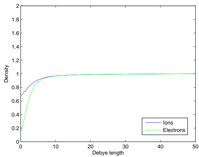
Fig. 2.3: Plasma sheath.
