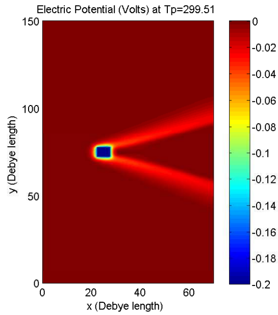
Fig. 3.7: Electric potential (Volts) for ions entering parallel to x-axis.
