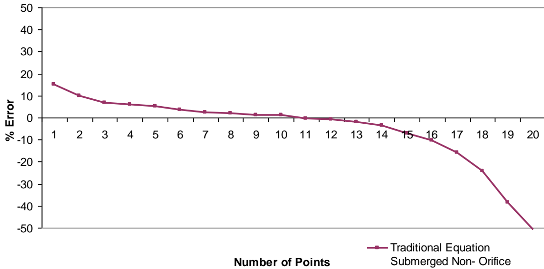
Fig. 43. Difference in error between calculated and measured discharge versus number of points measured for a discharge of 0.135 \text{ m}^3/\text{s} and G_0 of 0.25 \text{ m} (see Table 16)
