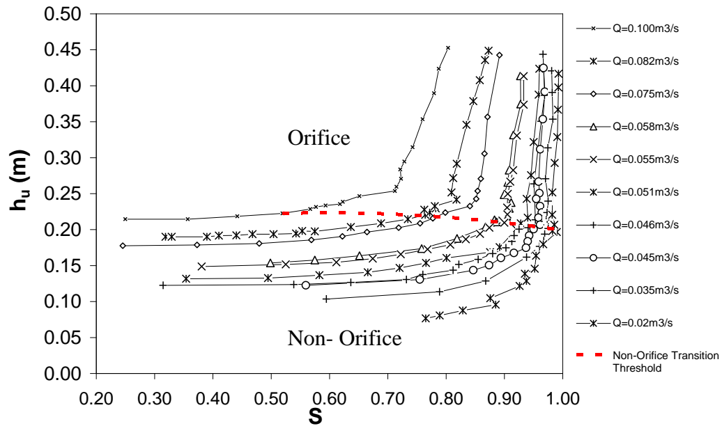
Fig. 13. Upstream water depth ( h_u ) vs. submergence ( S ) for G_o = 0.20 m, where orifice flow exists above the dashed line, and non-orifice flow below the dashed line
