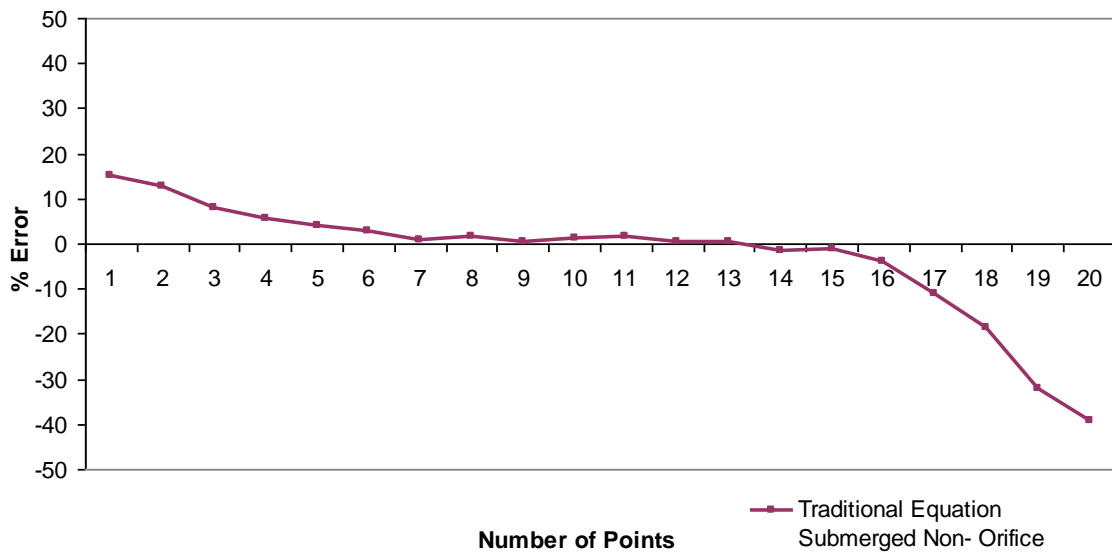
Fig. 44. Difference in error between calculated and measured discharge versus number of points measured for a discharge of 0.151 \text{ m}^3/\text{s} and G_0 of 0.30 \text{ m} (see Table 16)
