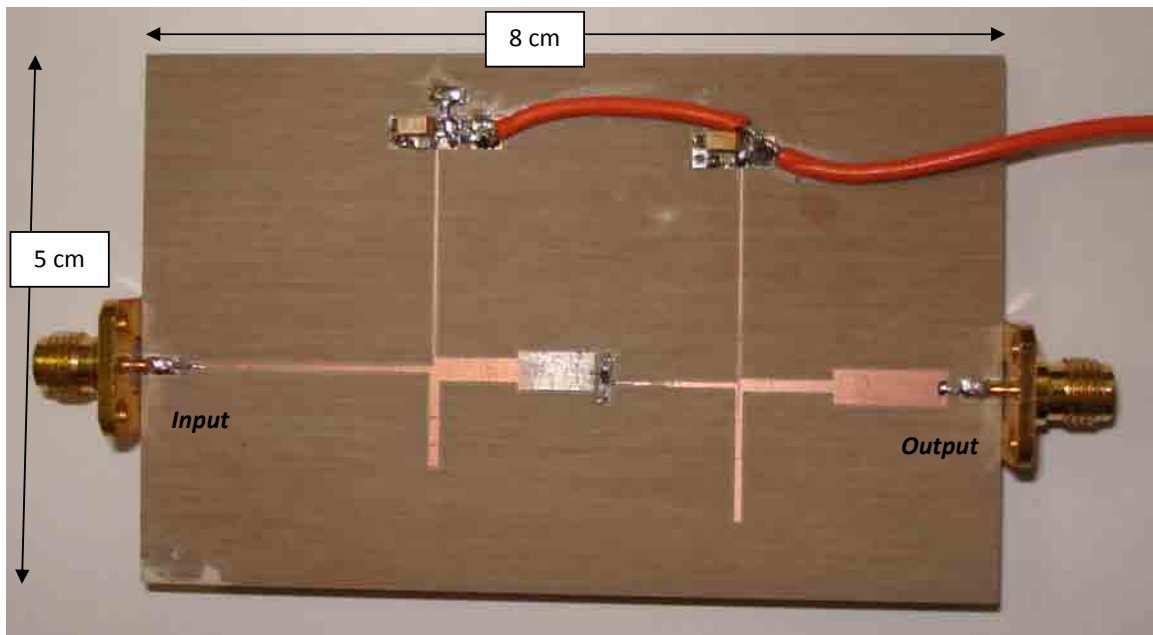
Fig. 2.6: Fabricated amplifier at 2.4\text{ GHz} .
