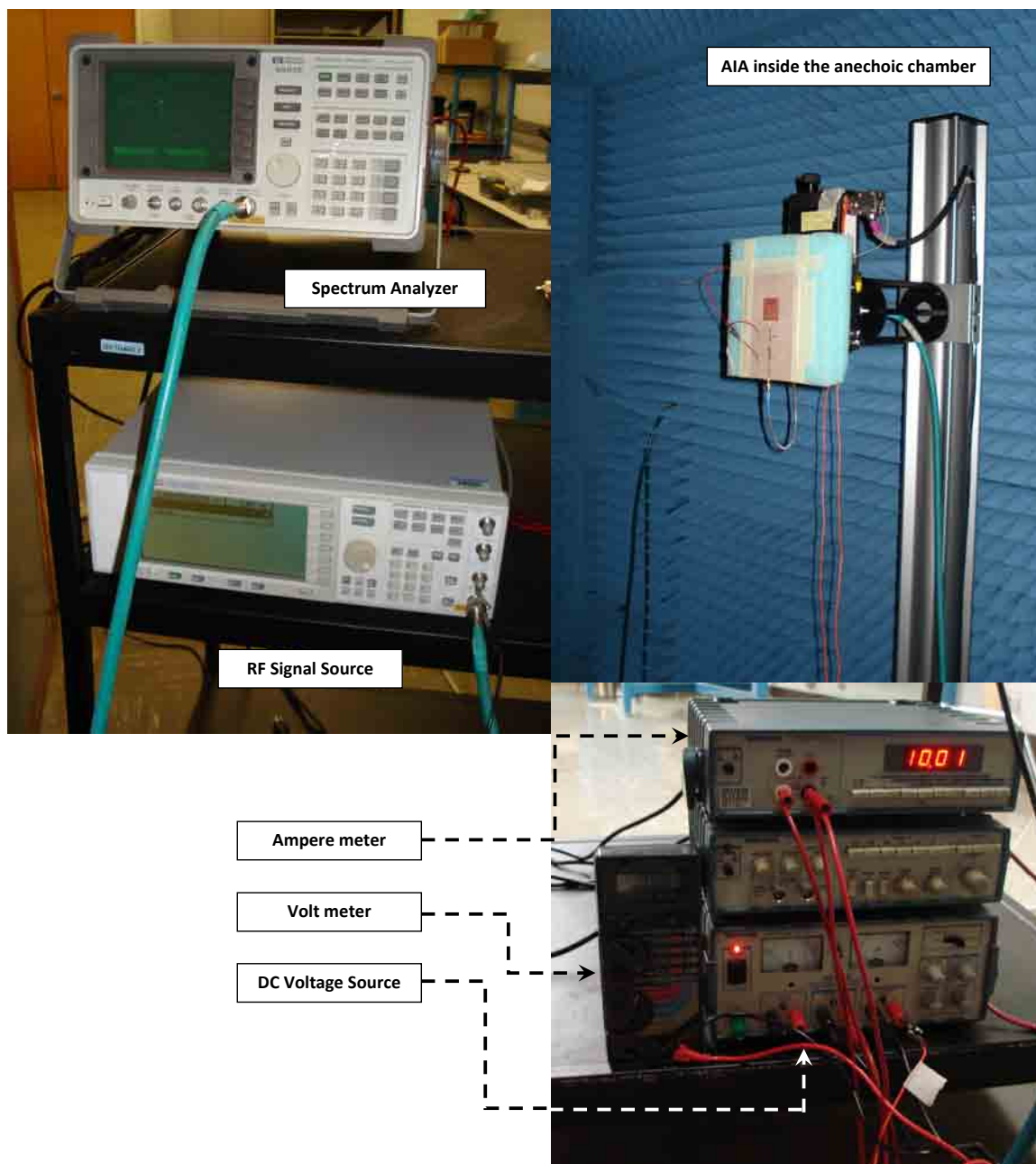
Fig. 4.9: Measurement setup for power measurement.
