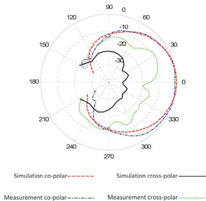
Fig. 5.9: Radiation pattern of active integrated right-hand CP patch antenna at 2.4 GHz in \Phi = 0^\circ cut.
