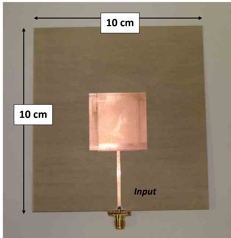
Fig. 4.6: Simple patch used for calibration.
