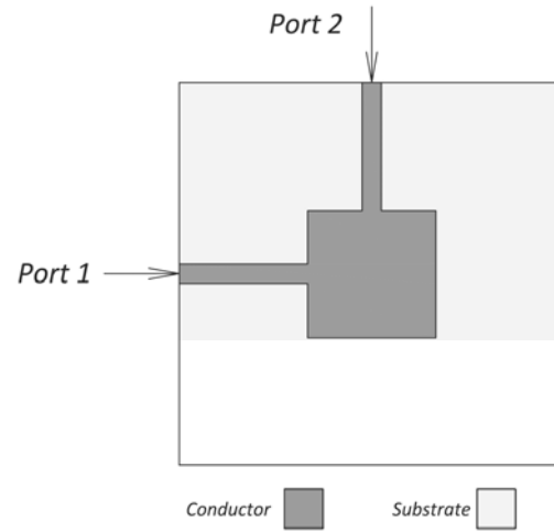
Fig. 3.4: LP and CP patch top view.
