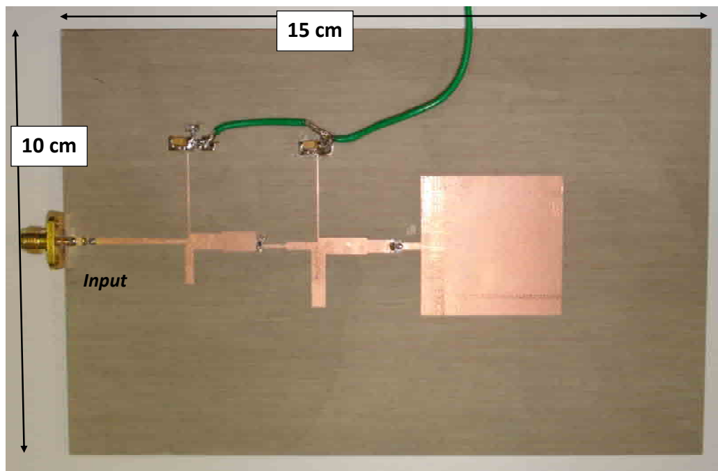
Fig. 4.3: Fabricated 2.4 GHz amplifier integrated with square patch antenna.
