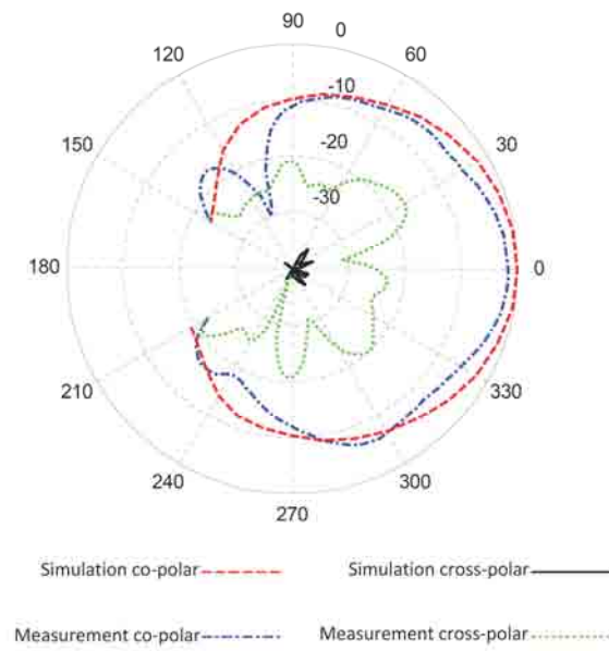
Fig. 4.15: Radiation pattern of simple patch antenna at 2.415\text{ GHz} integrated with the amplifier in \Phi = 0^\circ cut.
