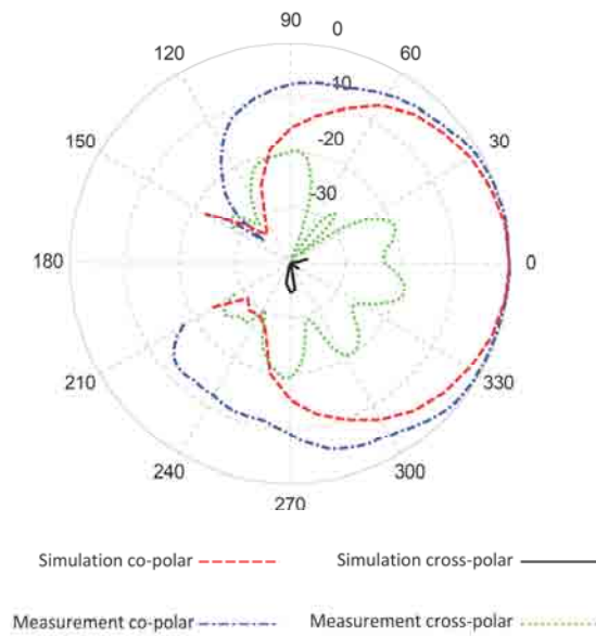
Fig. 4.18: Radiation pattern of the patch antenna with harmonic suppression at 2.4\text{ GHz} integrated with the amplifier \Phi = 90^\circ cut.
