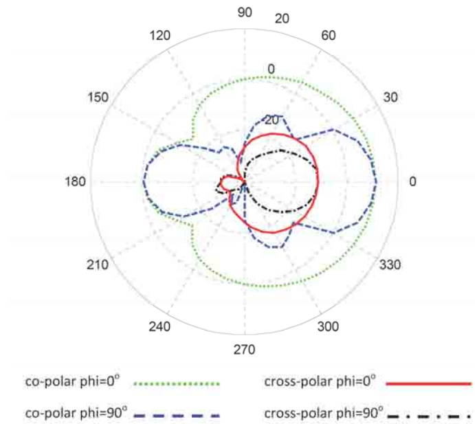
Fig. 6.3: Radiation patterns of array of five elements in two planes of \Phi = 0^\circ and \Phi = 90^\circ for linear polarization.
