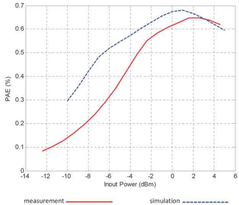
Fig. 2.8: Simulated and measured PAE of the 2.4 GHz amplifier.
