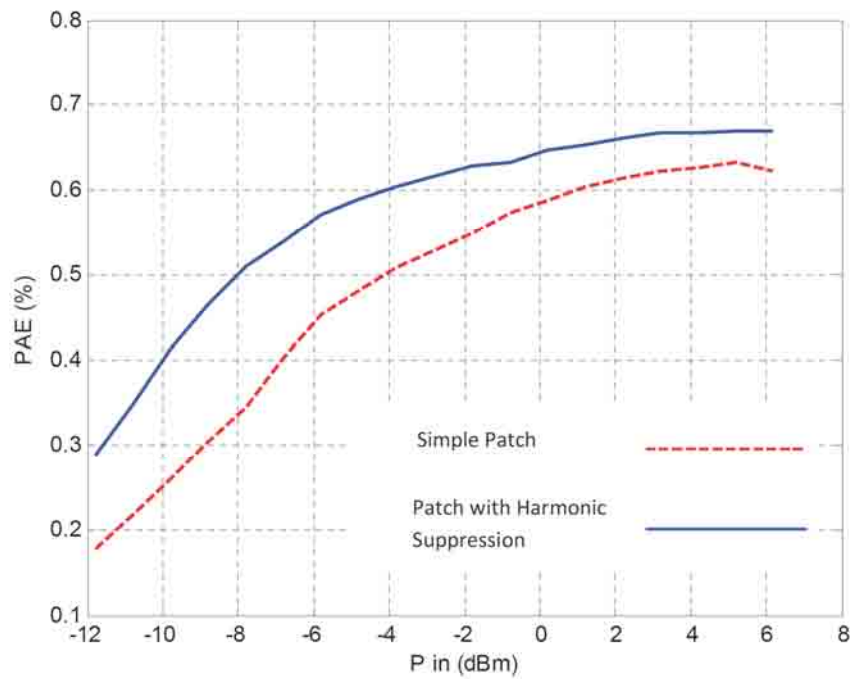
Fig. 4.13: Measurement results of PAE for simple patch and the patch with harmonic suppression.
