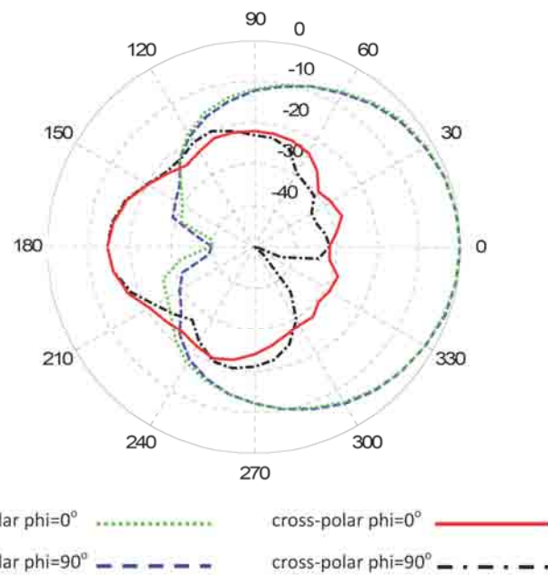
Fig. 3.15: Radiation pattern of CP square patch antenna with harmonic suppression.
