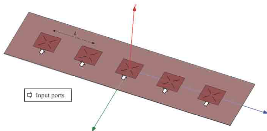
Fig. 6.1: Array of five elements for linear polarization.
