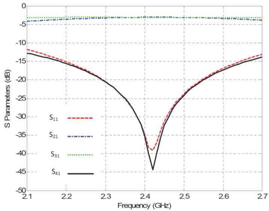
Fig. 5.2: Simulation results for magnitude of S-parameters for the branch-line coupler.
