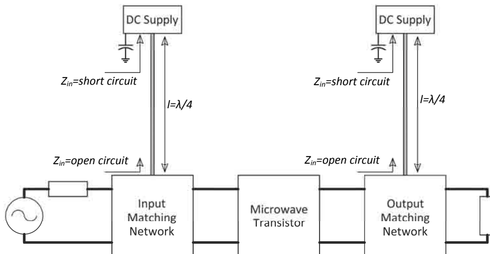
Fig. 2.3: DC circuit for microwave amplifier.
