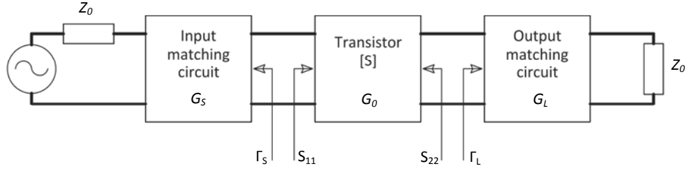
Fig. 2.1: Block diagram of a microwave amplifier to find unilateral transducer power gain.
