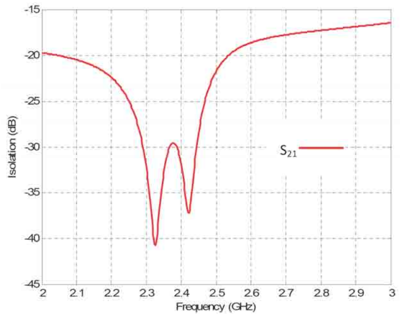
Fig. 3.17: Isolation between two ports of CP square patch antenna with harmonic suppression.
