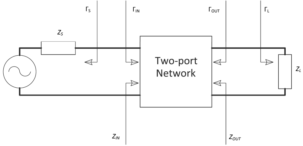
Fig. 2.2: Stability of two-port network.
