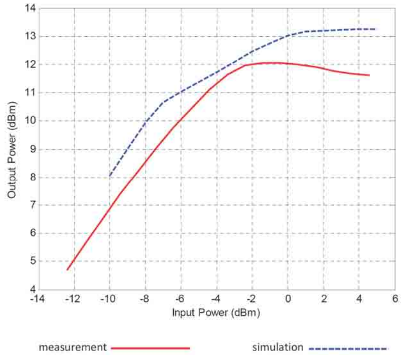
Fig. 2.7: Simulated and measured output power of the 2.4 GHz amplifier.
