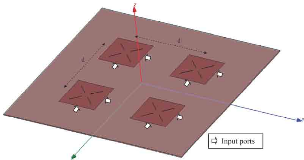
Fig. 6.5: Array of four elements for circular polarization.
