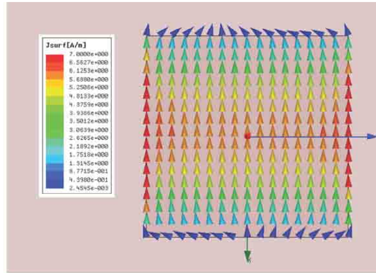
Fig. 3.7: Current distribution of the square patch antenna at the fundamental frequency of operation.
