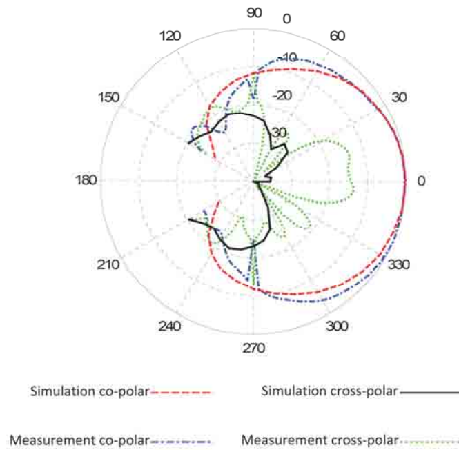
Fig. 5.11: Radiation pattern of active integrated left-hand CP patch antenna at 2.4\text{ GHz} in \Phi = 0^\circ cut.
