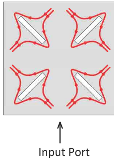
Fig. 3.10: Slits on a square patch to move the second harmonic response.
