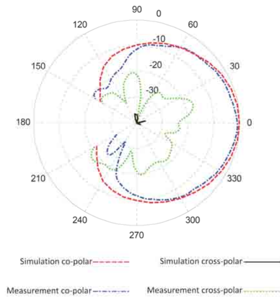
Fig. 4.17: Radiation pattern of the patch antenna with harmonic suppression at 2.4\text{ GHz} integrated with the amplifier in \Phi = 0^\circ cut.
