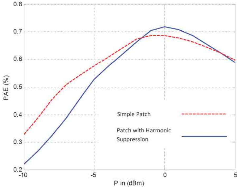
Fig. 4.11: Simulation results of PAE for simple patch and the patch with harmonic suppression.
