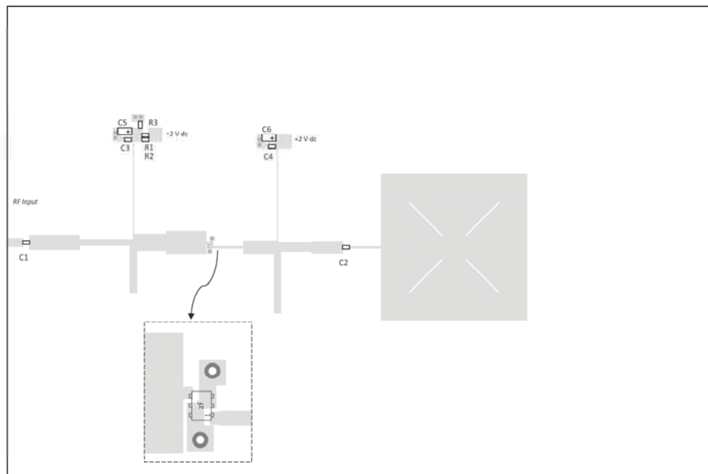
Fig. 4.2: Layout of 2.4 GHz amplifier integrated with square patch antenna with harmonic suppression.
