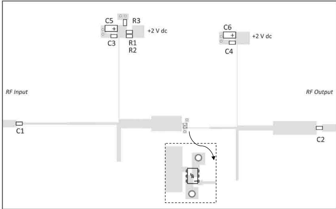
Fig. 2.4: Layout of 2.4 GHz amplifier.
