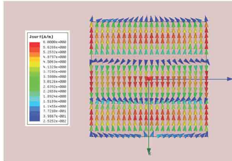
Fig. 3.9: Current distribution of the square patch antenna at its third harmonic.
