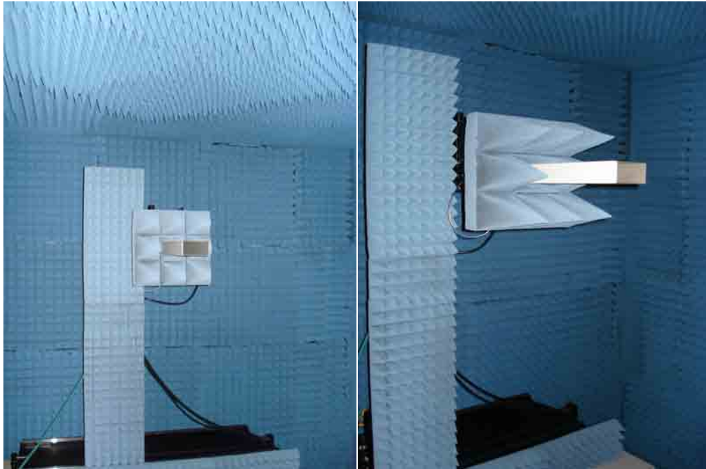
Fig. 4.5: Near-field probe as the receive antenna.
