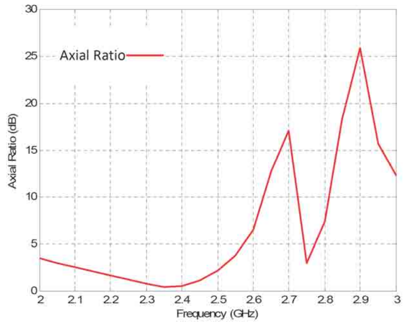
Fig. 3.16: Axial ratio of the CP square patch antenna with harmonic suppression.
