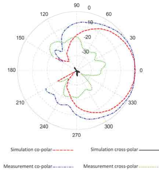
Fig. 4.16: Radiation pattern of simple patch antenna at 2.415\text{ GHz} integrated with the amplifier in \Phi = 90^\circ cut.
