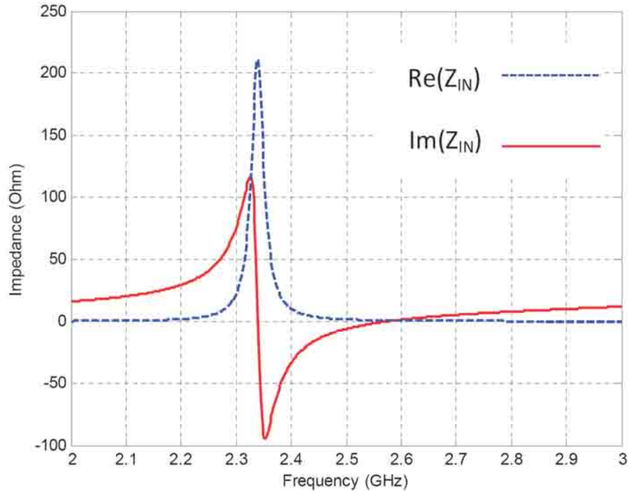
Fig. 3.3: Input impedance of a rectangular patch antenna.
