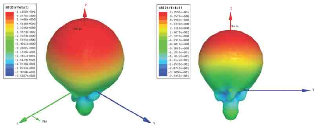
Fig. 6.6: 3-D pattern of directivity for array of four elements 0 degrees beam tilting.
