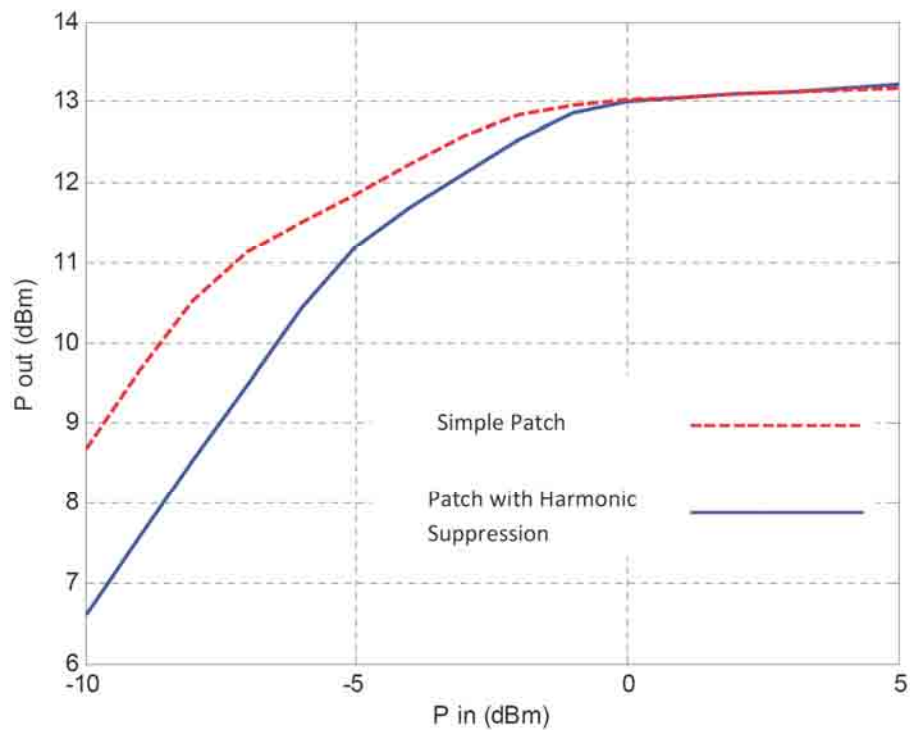
Fig. 4.10: Simulation results of output power for simple patch and the patch with harmonic suppression.
