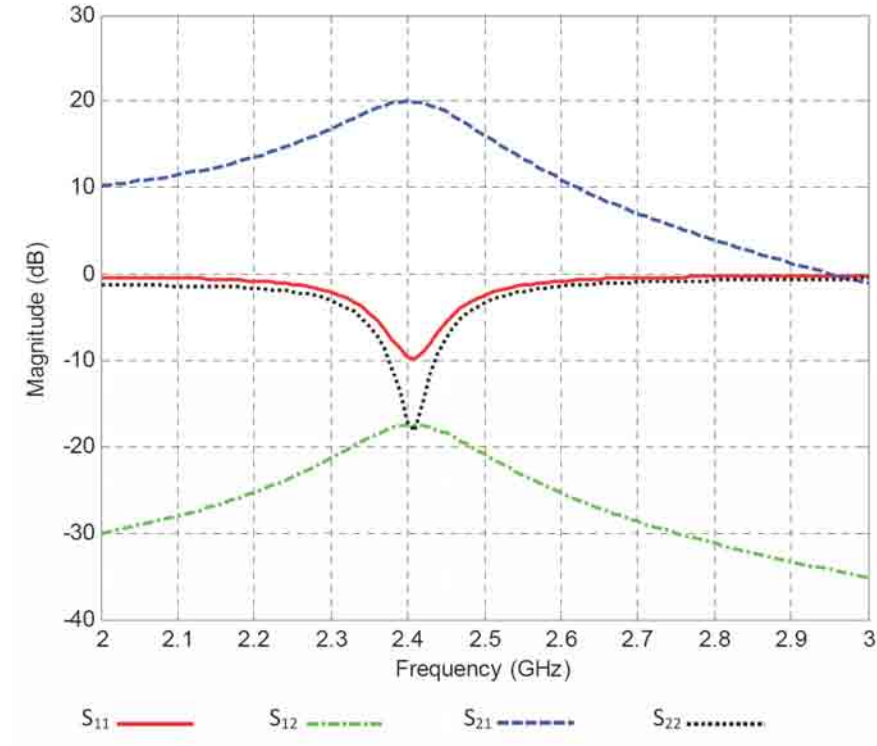
Fig. 2.5: S-parameter simulation results of the 2.4 GHz amplifier.
