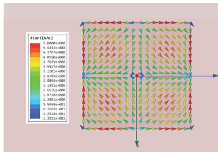
Fig. 3.8: Current distribution of the square patch antenna at its second harmonic.
