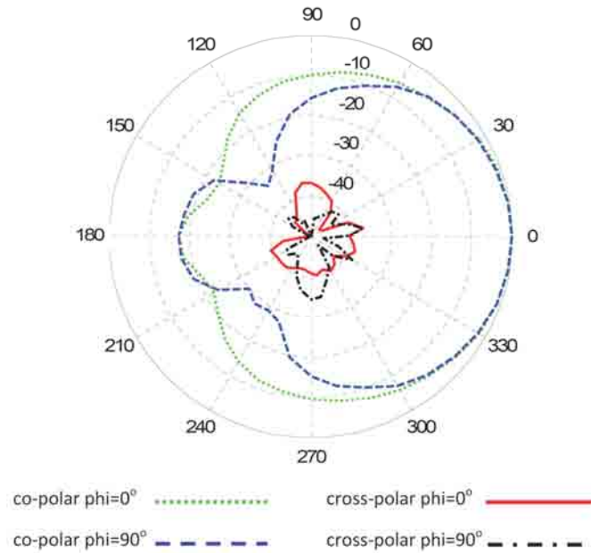
Fig. 3.13: Radiation pattern of LP square patch antenna with harmonic suppression at 2.4\text{ GHz} .
