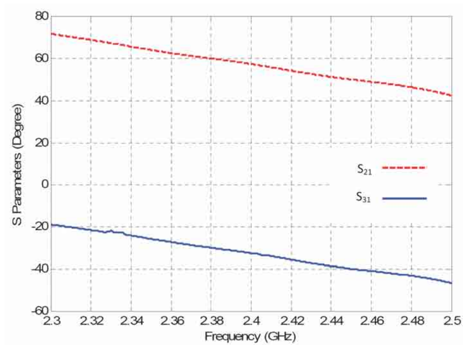
Fig. 5.6: Measurement results for phase of S_{21} and S_{31} for the branch-line coupler.
