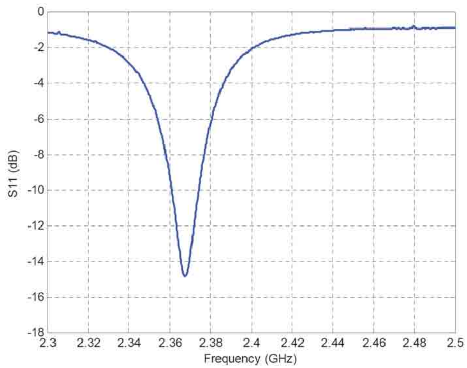
Fig. 4.8: Measurement results of S_{11} for the simple patch antenna with coupling port.
