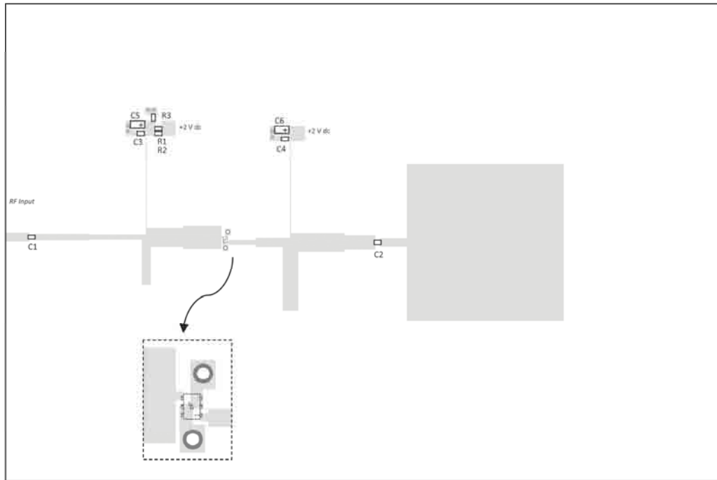
Fig. 4.1: Layout of 2.4 GHz amplifier integrated with square patch antenna.
