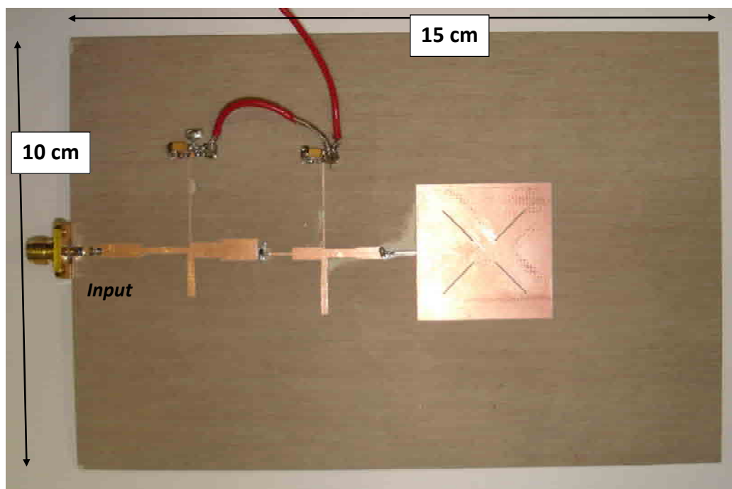
Fig. 4.4: Fabricated 2.4 GHz amplifier integrated with square patch antenna with harmonic suppression.
