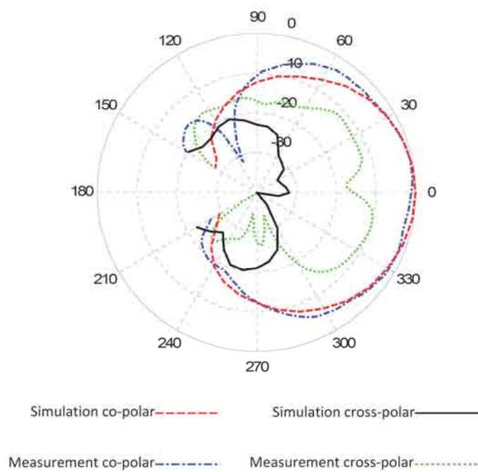
Fig. 5.10: Radiation pattern of active integrated right-hand CP patch antenna at 2.4 GHz in \Phi = 90^\circ cut.
