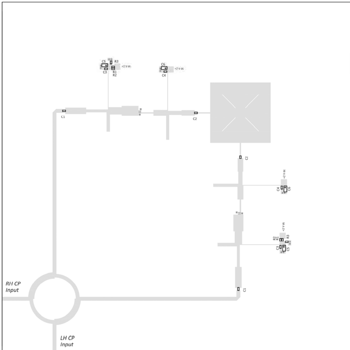
Fig. 5.7: Layout of CP active integrated antenna with harmonic suppression at 2.4 GHz.
