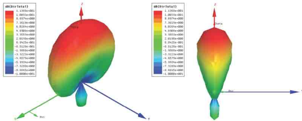
Fig. 6.2: 3-D pattern of directivity for array of five elements 0 degrees beam tilting.
