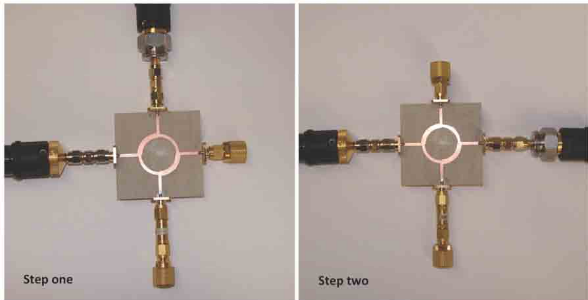
Fig. 5.4: The fabricated branch-line coupler and measurement steps.
