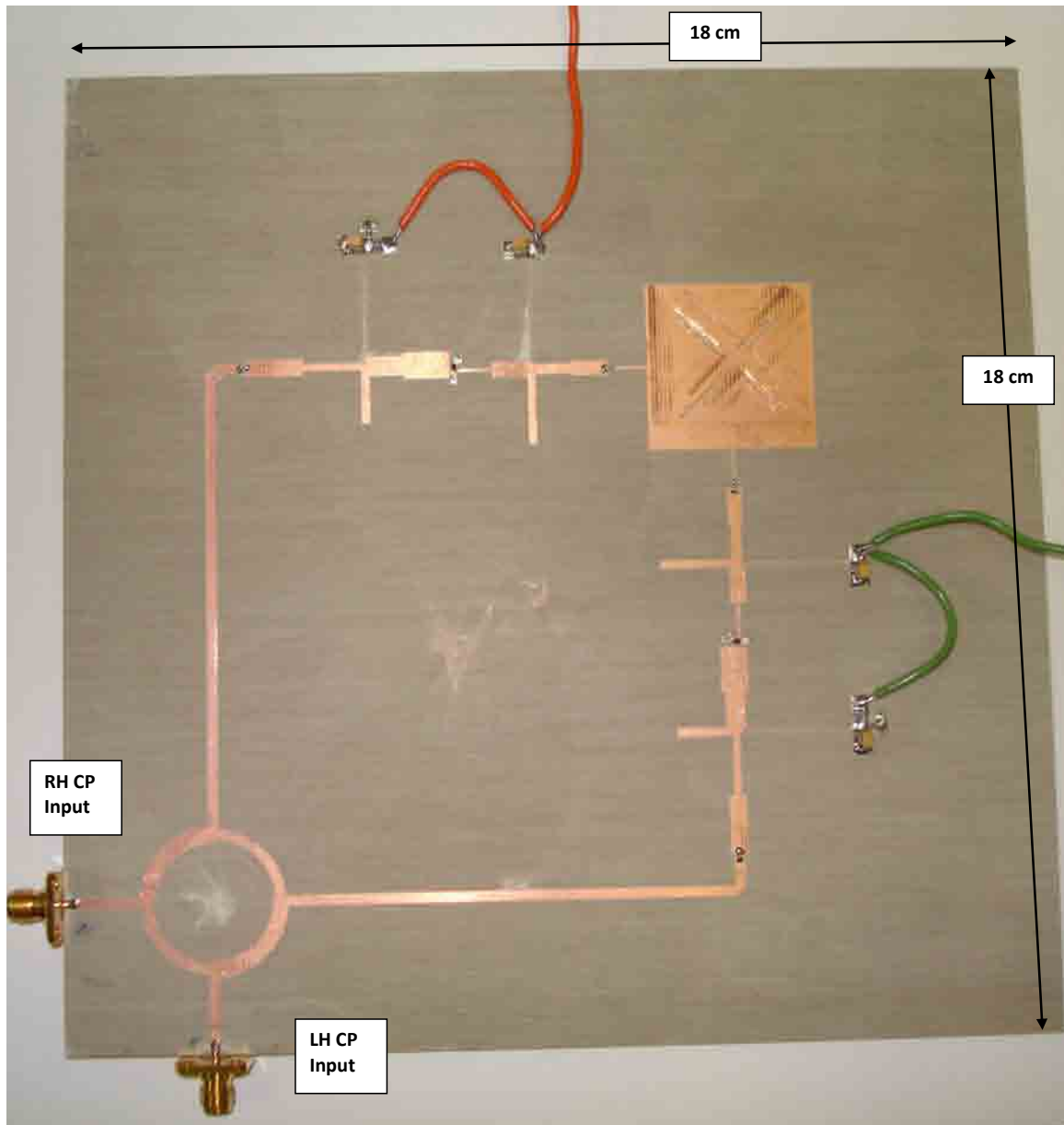
Fig. 5.8: Fabricated CP active integrated antenna with harmonic suppression at 2.4 GHz.
