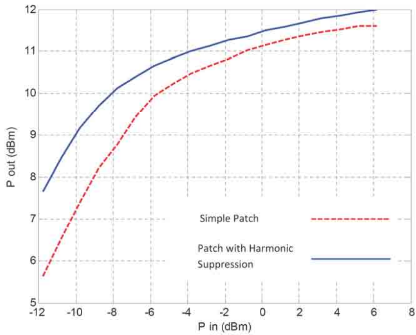
Fig. 4.12: Measurement results of output power for simple patch and the patch with harmonic suppression.
