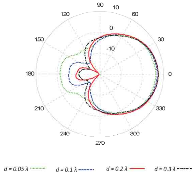
Fig. 3.2: The effect of ground size on the patch directivity.
