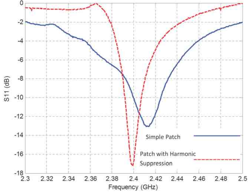
Fig. 4.14: S_{11} plots for simple patch and the patch with harmonic suppression both integrated with the amplifier.
