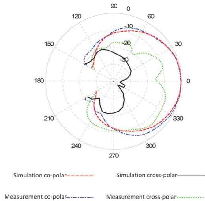
Fig. 5.12: Radiation pattern of active integrated left-hand CP patch antenna at 2.4\text{ GHz} in \Phi = 90^\circ cut.
