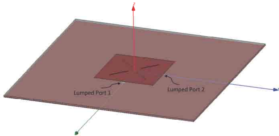
Fig. 3.14: The CP square patch antenna with harmonic suppression.
