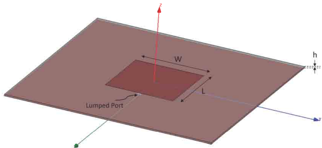
Fig. 3.5: Square patch antenna.
