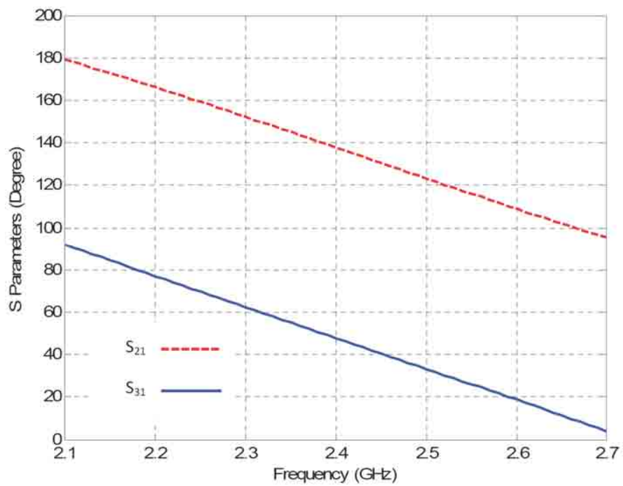
Fig. 5.3: Simulation results for phase of S_{21} and S_{31} for the branch-line coupler.
