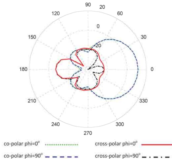
Fig. 6.7: Radiation patterns of array of four elements in two planes of \Phi = 0^\circ and \Phi = 90^\circ for circular polarization.
