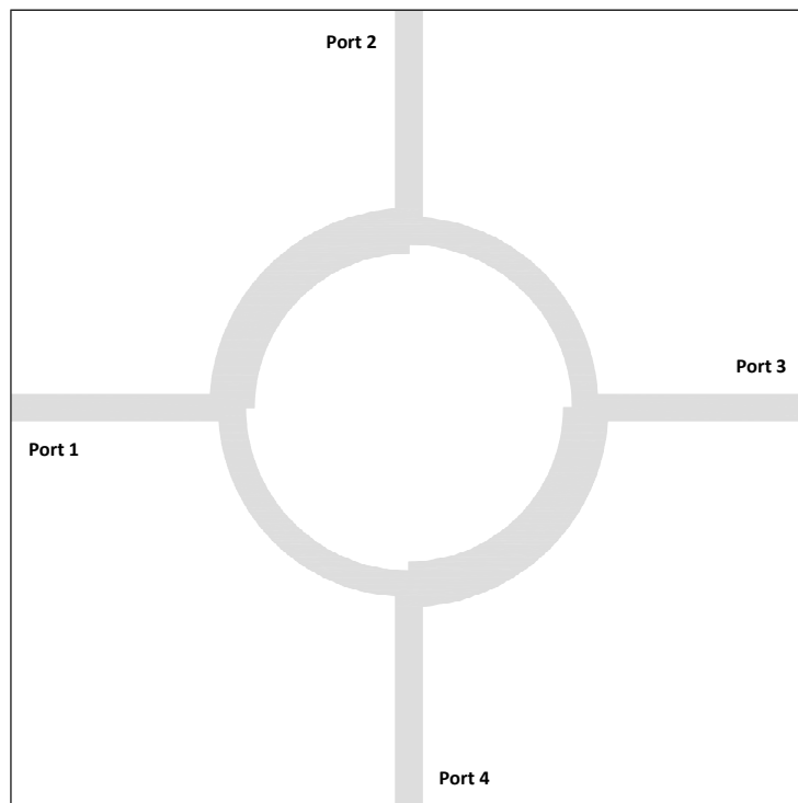
Fig. 5.1: Layout of branch-line coupler at 2.4 GHz.
