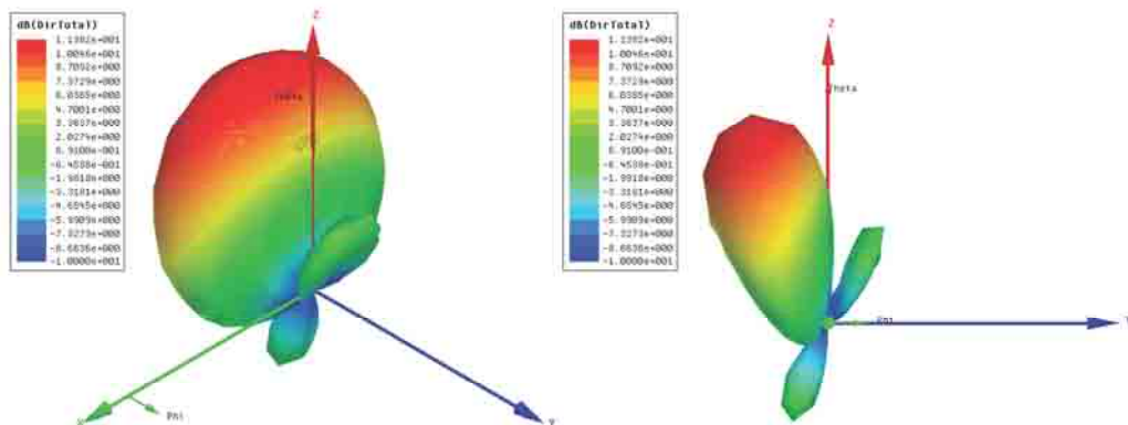
Fig. 6.4: 3-D pattern of directivity for array of five elements 30 degrees beam tilting.
