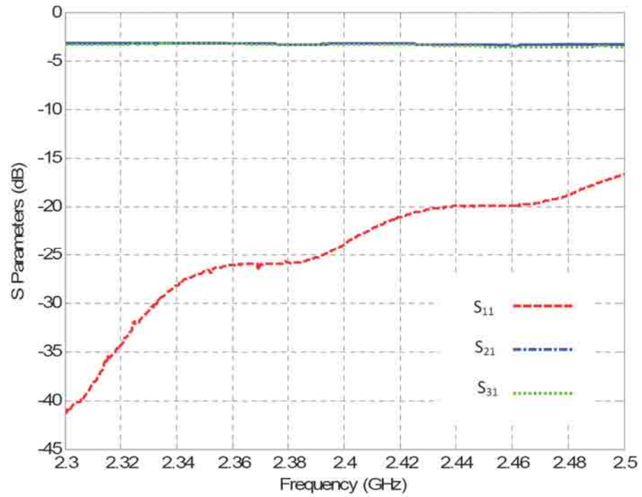
Fig. 5.5: Measurement results for magnitude of S-parameters for the branch-line coupler.
