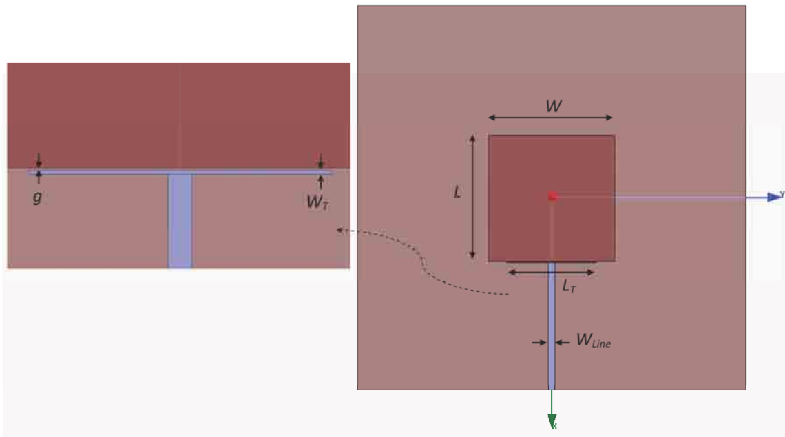
Fig. 4.7: Simple patch antenna with coupling port's schematic and dimensions.
