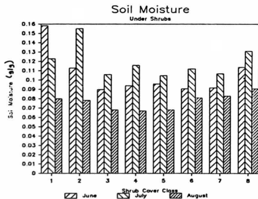
Figures 1 and 2. Soil moisture at landscape positions grouped into eight shrub cover classes: 1-- Artemisia tridentata ssp. vaseyana , 2-- A. tridentata ssp. vaseyana mixed with grasses, 3-- A. tridentata ssp. vaseyana , A. tridentata ssp. wyomingensis , and grasses, 4-- A. tridentata ssp. wyomingensis , 5-- A. tridentata ssp. wyomingensis mixed with grasses, 6-- A. nova , 7-- A. nova mixed with grasses, and 8-- A. nova , grasses and cushion plants. Figure 1 represents soil moisture at between-shrub positions within these shrub cover classes, and Figure 2 represents the under-shrub positions.
