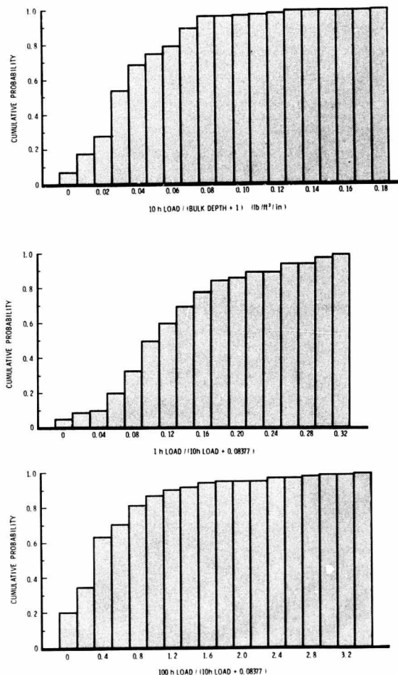
Figure 9.--Cumulative probability distributions for assigning 1h, 10h, and 100h fuel loads to each cell given the bulk depth.
