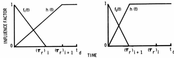
Figure 8.--Influencing factors governing fire transition from cell i to cell (i+1)
