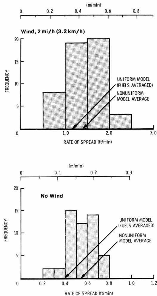
Figure 6.--Frequency distribution of the rate of spread in slash fuels at 0 wind speed and at a 2 mi/h windspeed. The average rate of spread is indicated for the uniform model (average fuel parameters from the simulated array) for comparison with the nonuniform model (average value of the distribution).
