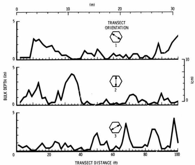
Figure 2.--A representative transect of the bulk depth evaluated every 2 feet. Three orientations are shown: (1) 80° counterclockwise to the uphill direction, (2) uphill, and (3) 80° clockwise to the uphill direction.
