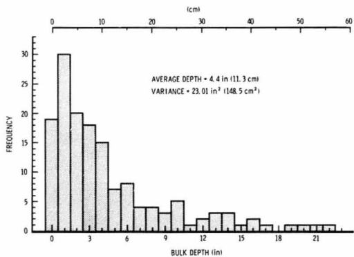
Figure 3.--Frequency distribution of the slash bulk depth. (All measurements were made at a resolution of 1 inc. (2.54 cm).)
