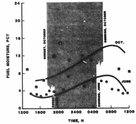
Figure 16.—Diurnal fuel moisture measurements (dots and squares) and model predictions (lines) for June and October in Arizona beneath a 4.4 percent crown closure ponderosa pine stand.
