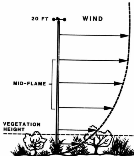
Figure 7.—Near-surface wind profile.
