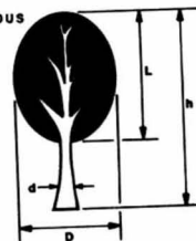
Figure 5.—Tree crown shape assumptions.
