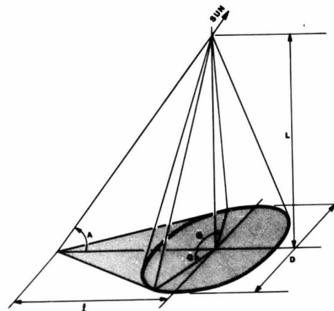
Figure 6A.—Conifer tree shadow configuration.
