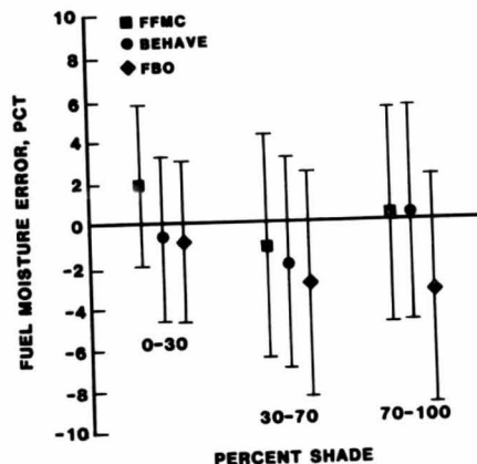
Figure 11.—Early afternoon mean and standard deviation trends for the three moisture models in three shade conditions.
