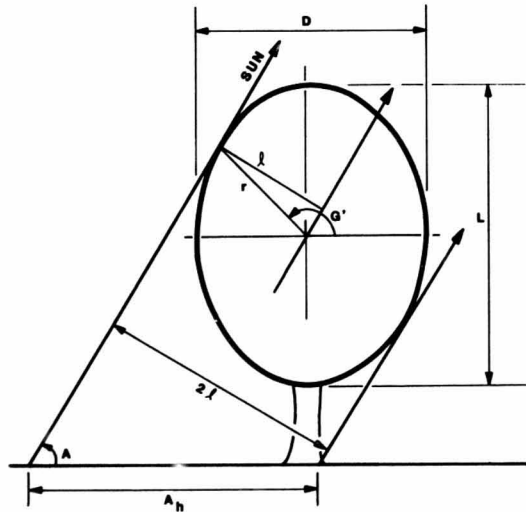
Figure 6B.—Deciduous tree shadow configuration.
