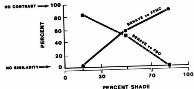
Figure 12.—Contrast P level between BEHAVE and other moisture models.
