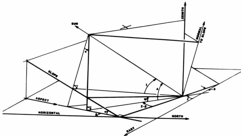
Figure 4.—Diagram of sun/slope geometry.
