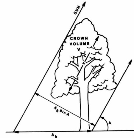
Figure 6C.—Inter-crown path length relationship.
