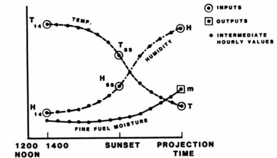
Figure 9.—Typical nighttime weather and moisture relationships.
