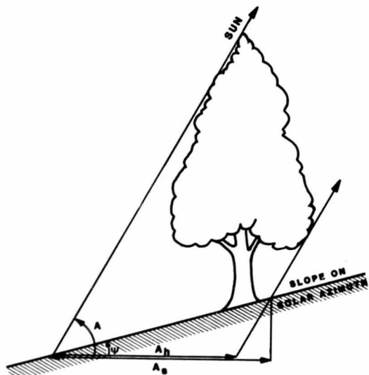
Figure 6D.—Shadow relationship to slope.
