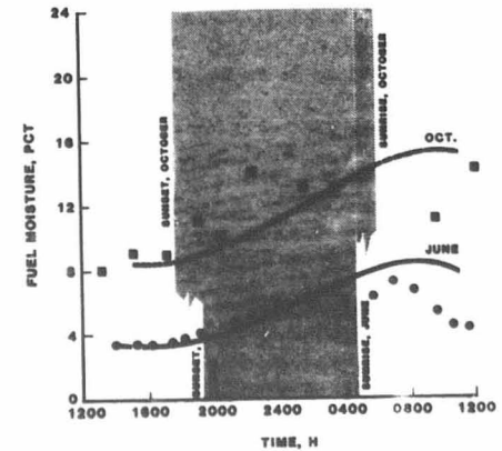
Figure 17.—Diurnal fuel moisture measurements (dots and squares) and model predictions (lines) for June and October in Arizona beneath a 74 percent crown closure ponderosa pine stand.
