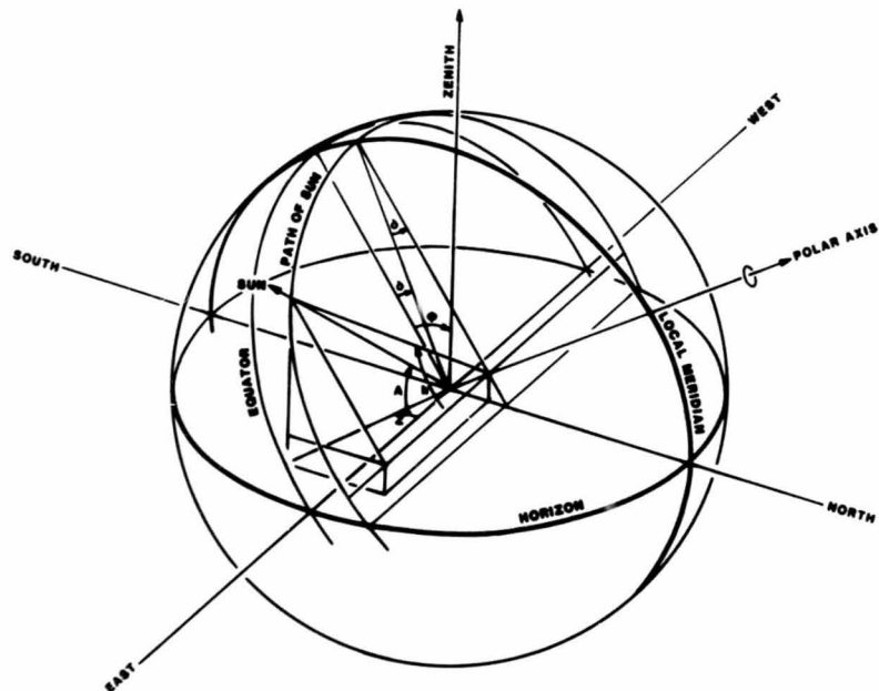
Figure 3.—Diagram of solar geometry.
