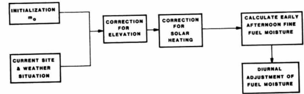
Figure 1.—Flow diagram of fine fuel moisture model.
