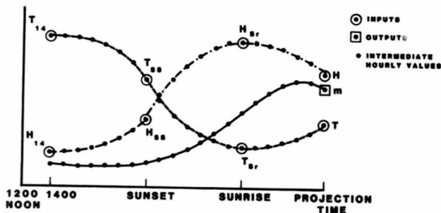
Figure 10.—Typical morning weather and moisture relationships.
