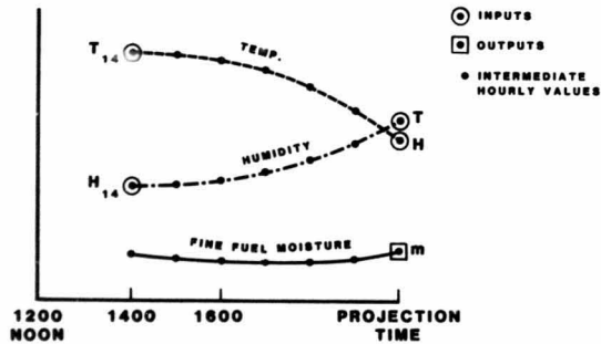
Figure 8.—Typical late afternoon weather and moisture relationships.
