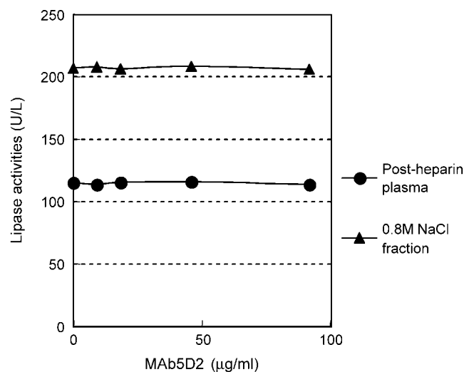
Fig. 2. Effect of anti-lipoprotein lipase monoclonal antibody 5D2 on lipase activity in postheparin plasma (PHP)- or 0.8 NaCl-eluted fraction from heparin-Sepharose. The reaction condition for the measurement of lipase activity was described in Materials and Methods, with the exception that increasing amounts of 5D2 were added in the reaction mixture. PHP was obtained from a normal volunteer 10 min after 30 U/kg heparin injection.
