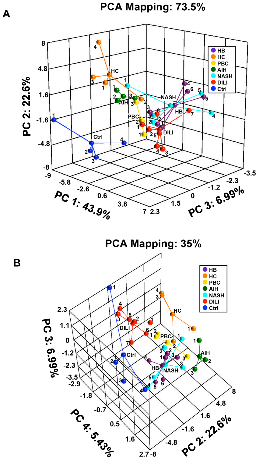
Figure 2. PCA of serum miRNA expression in 6 hepatitis B (HB), 4 hepatitis C (HC), 3 primary biliary cirrhosis (PBC), 3 autoimmune hepatitis (AIH), 5 non-alcoholic steatohepatitis (NASH), 7 drug-induced liver injury (DILI), and 4 control subjects (Ctrl). PCA was performed using 37 miRNAs that exceeded the cut-off value in all subjects (n = 32). (A)
