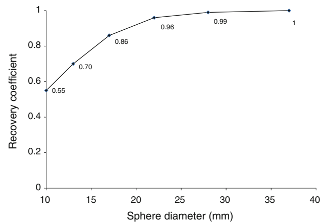
Fig. 1 The recovery coefficient (RC) of the PET/CT system used in this study. The RCs were determined referring to the Japanese Guideline for Oncology PET/CT. The phantom image was reconstructed by the optimal reconstruction parameters for RG PET
