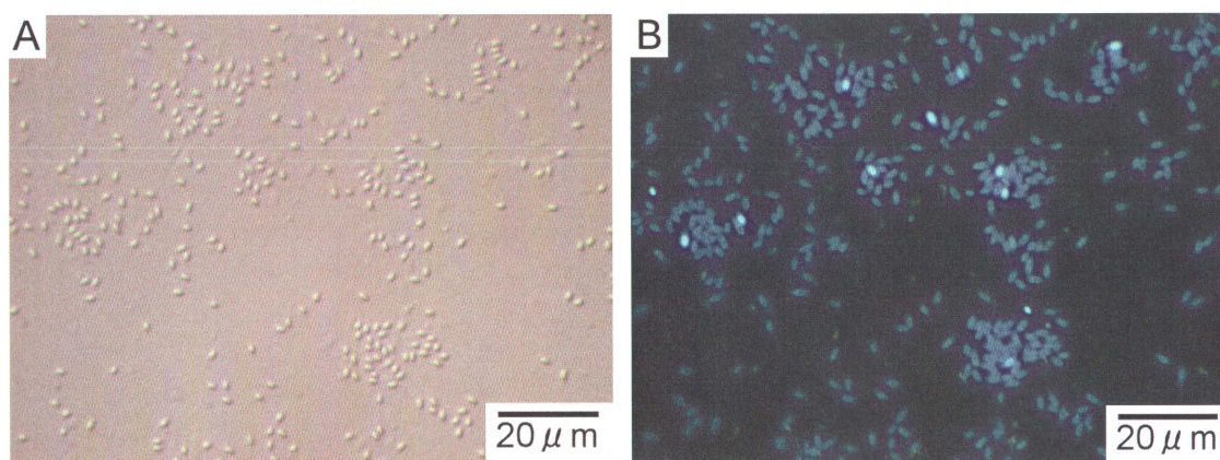
Figure 4 Optical micrographs of hydrocarbon-degrading bacteria of heavy oil polluted sand collected from Atake seashore at the top layer (0 - 30 cm) about 3 - 4 m outside the shoreline (bacterial cell shapes are predominant in short rods-shaped). (A) A differential interference microscopic image. (B) An episcopic fluorescence microscopic image.
