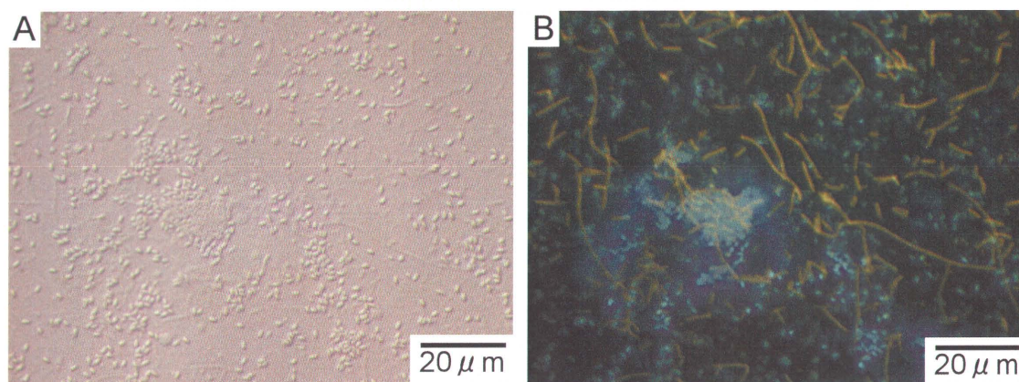
Figure 5 Optical micrographs of hydrocarbon-degrading bacteria of heavy oil polluted sand collected from Atake seashore at the top layer (0 - 60 cm) about 5 - 6 m outside the shoreline. Cells of bacteria form clusters (spherical or rods in long chains), while their shapes are short rods associated with filamentous. (A) A differential interference microscopic image. (B) An episcopic fluorescence microscopic image.
