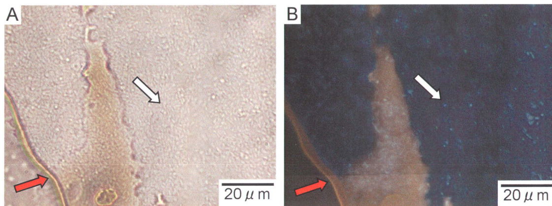
Figure 1 Optical micrographs of hydrocarbon-degrading bacteria in association with oil droplets at the inside building treatment. The sample was collected from Shioya seashore, Ishikawa Prefecture. The white arrow indicates bacteria, and the red arrow indicates heavy oil droplet designated by the brown color in the figure. (A) A differential interference microscopic image. (B)
