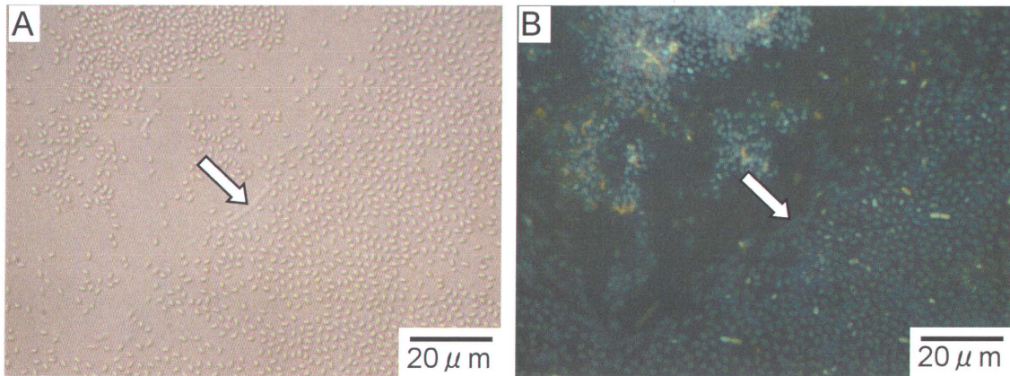
Figure 2 Optical micrographs of hydrocarbon-degrading bacteria in heavy oil at the outside building treatment showing various morphological forms (spherical and filamentous bacteria). The sample was collected from Togi seashore, Ishikawa Prefecture. The arrows indicate filamentous bacteria. (A) A differential interference microscopic image. (B) An episcopic fluorescence microscopic image.
